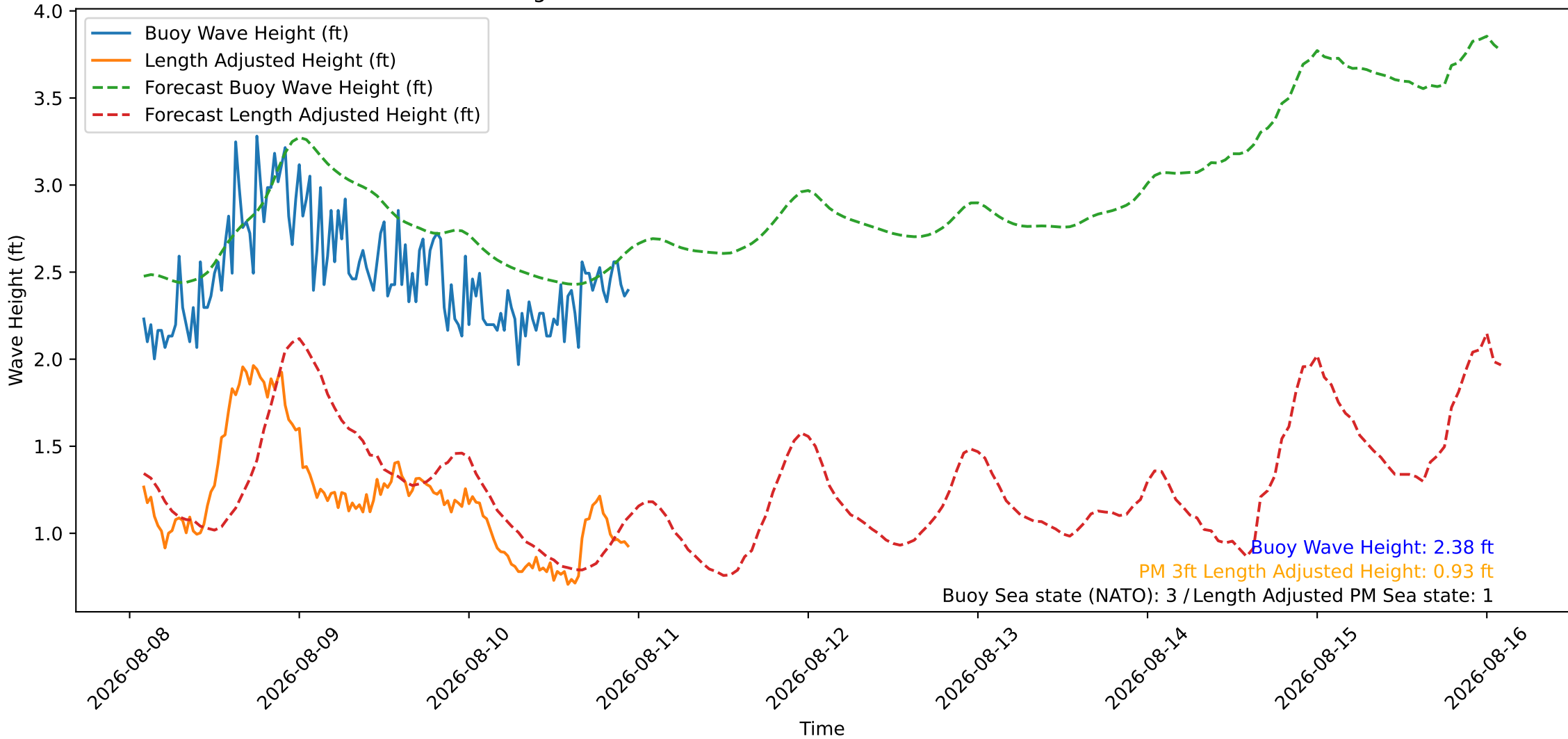
Wave Heights over Time for Oceanside Harbor at 2026-08-11 02:10:27
