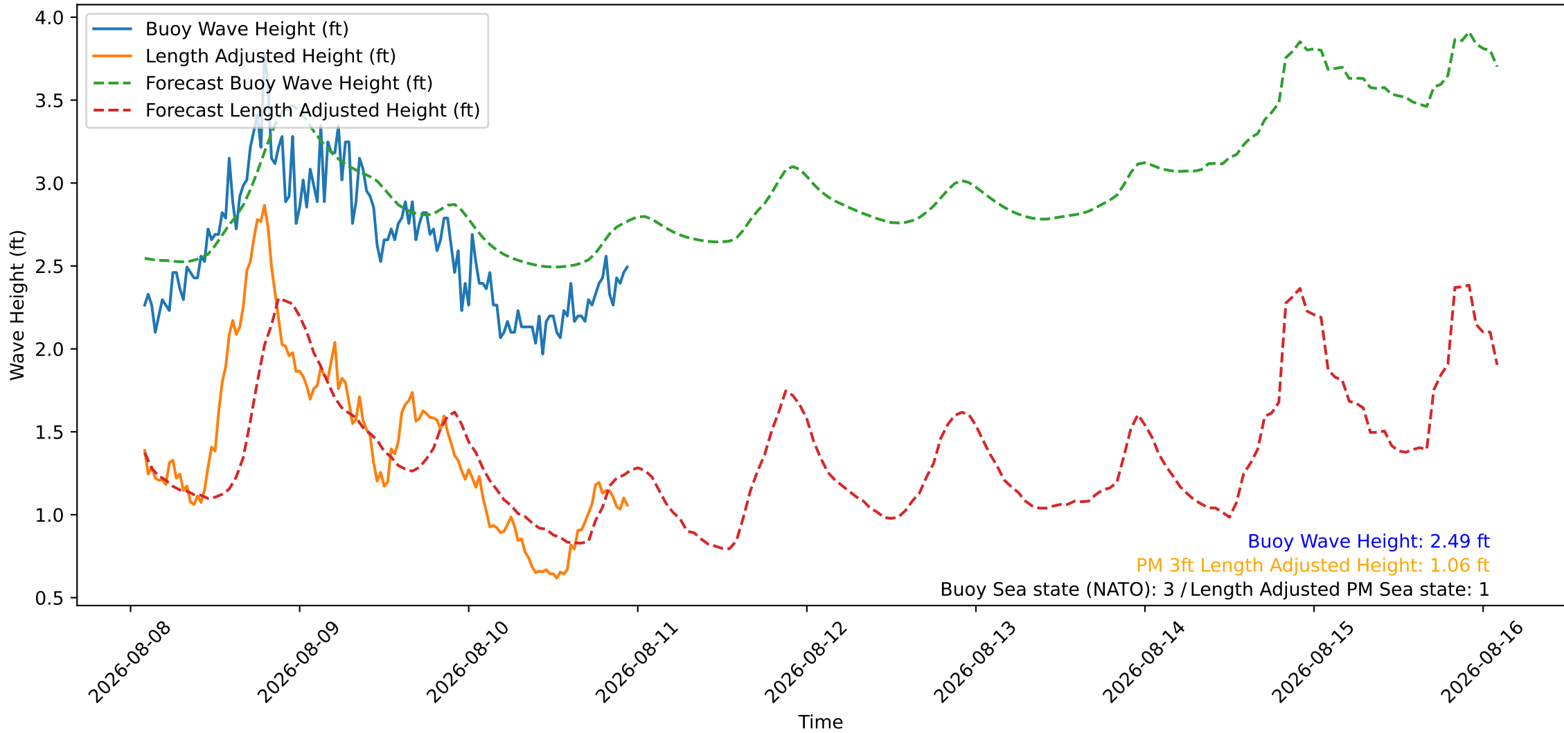
Wave Heights over Time for Green Beach at 2026-08-11 02:11:09
