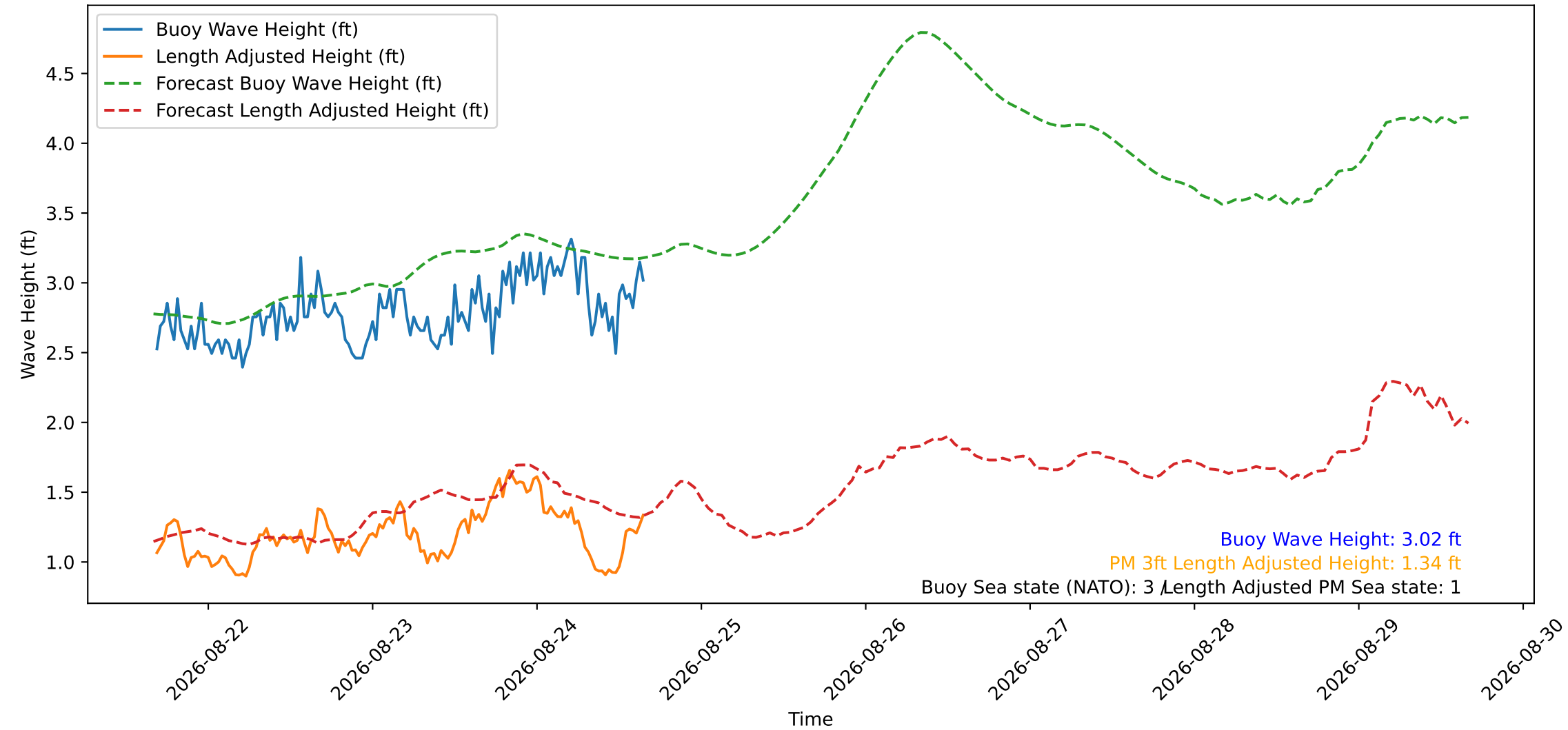
Wave Heights over Time for Green Beach at 2026-08-24 16:21:13
