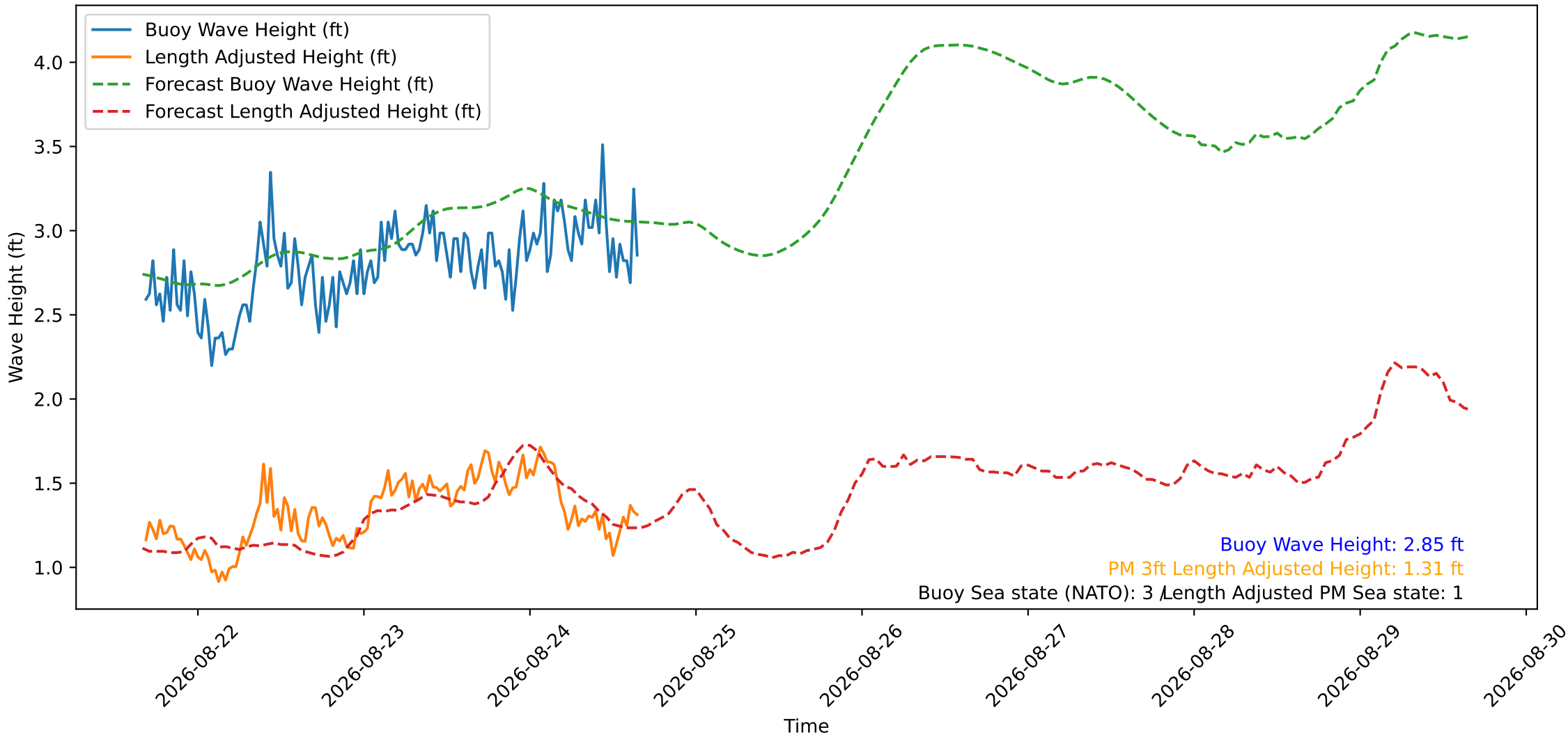
Wave Heights over Time for Oceanside Harbor at 2026-08-24 16:20:29
