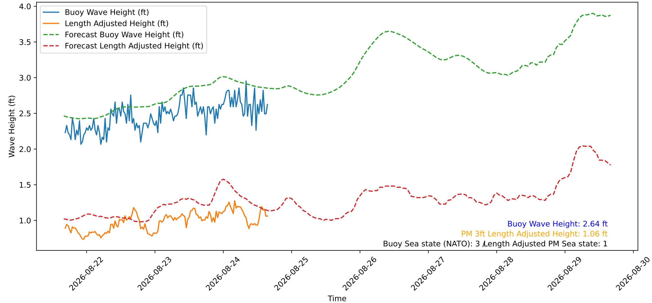
Wave Heights over Time for Red Beach at 2026-08-24 16:20:50
