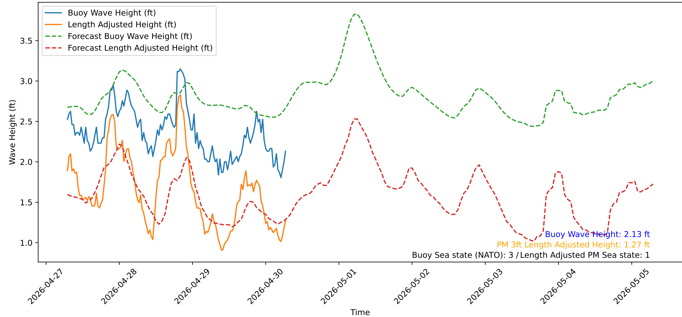
Wave Heights over Time for Green Beach at 2026-04-30 07:11:13
