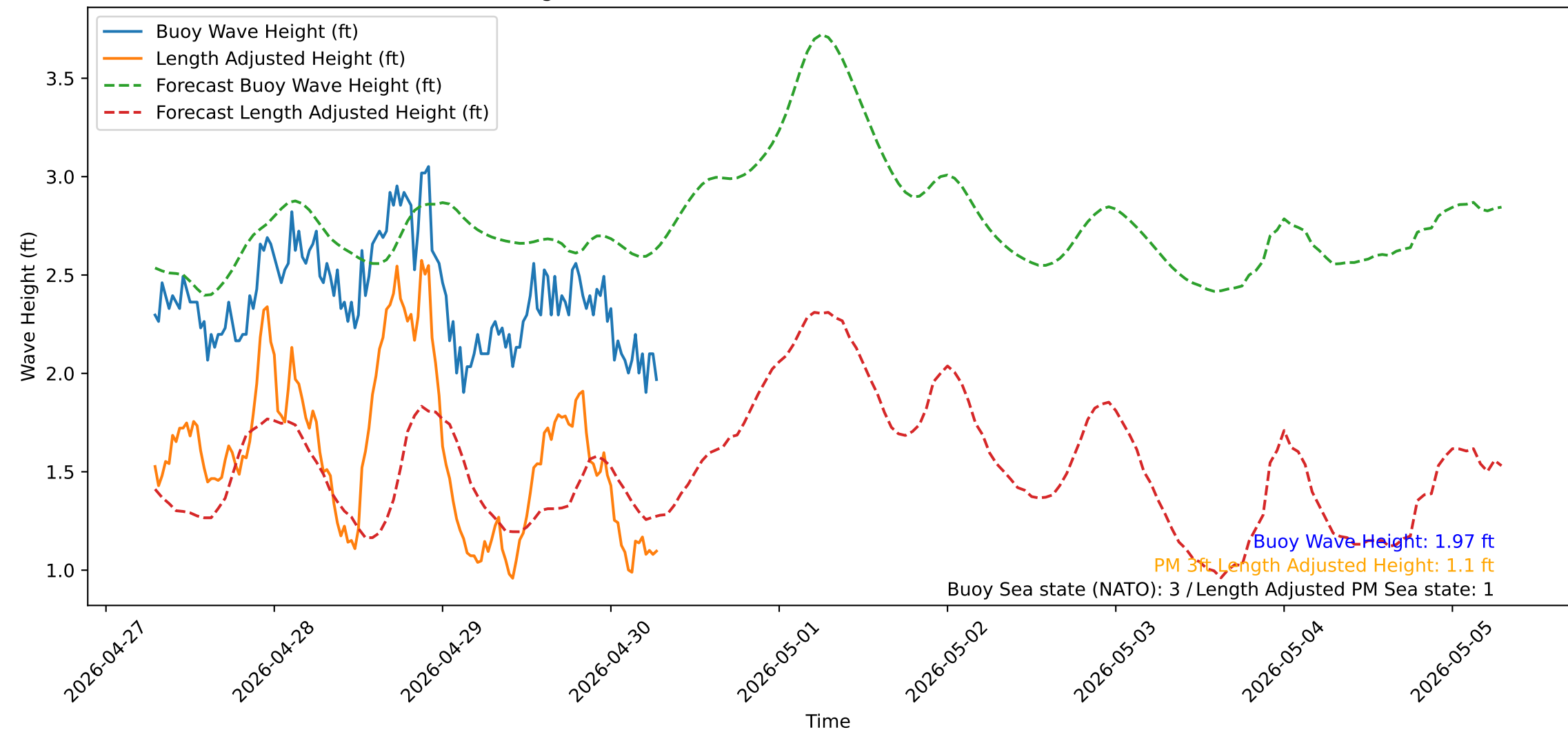
Wave Heights over Time for Oceanside Harbor at 2026-04-30 07:10:32
