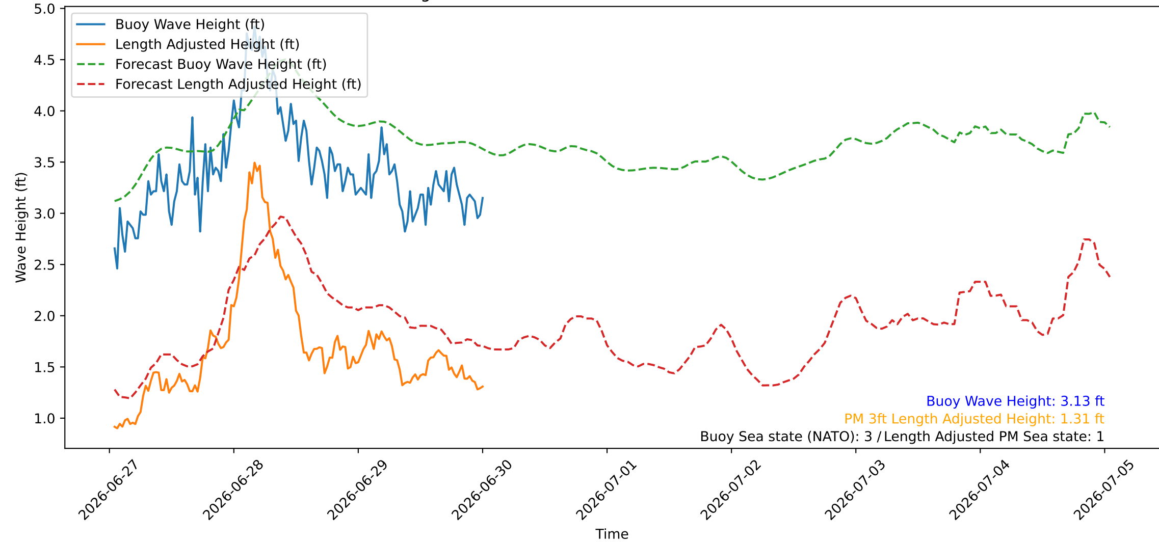
Wave Heights over Time for Green Beach at 2026-06-30 00:51:09
