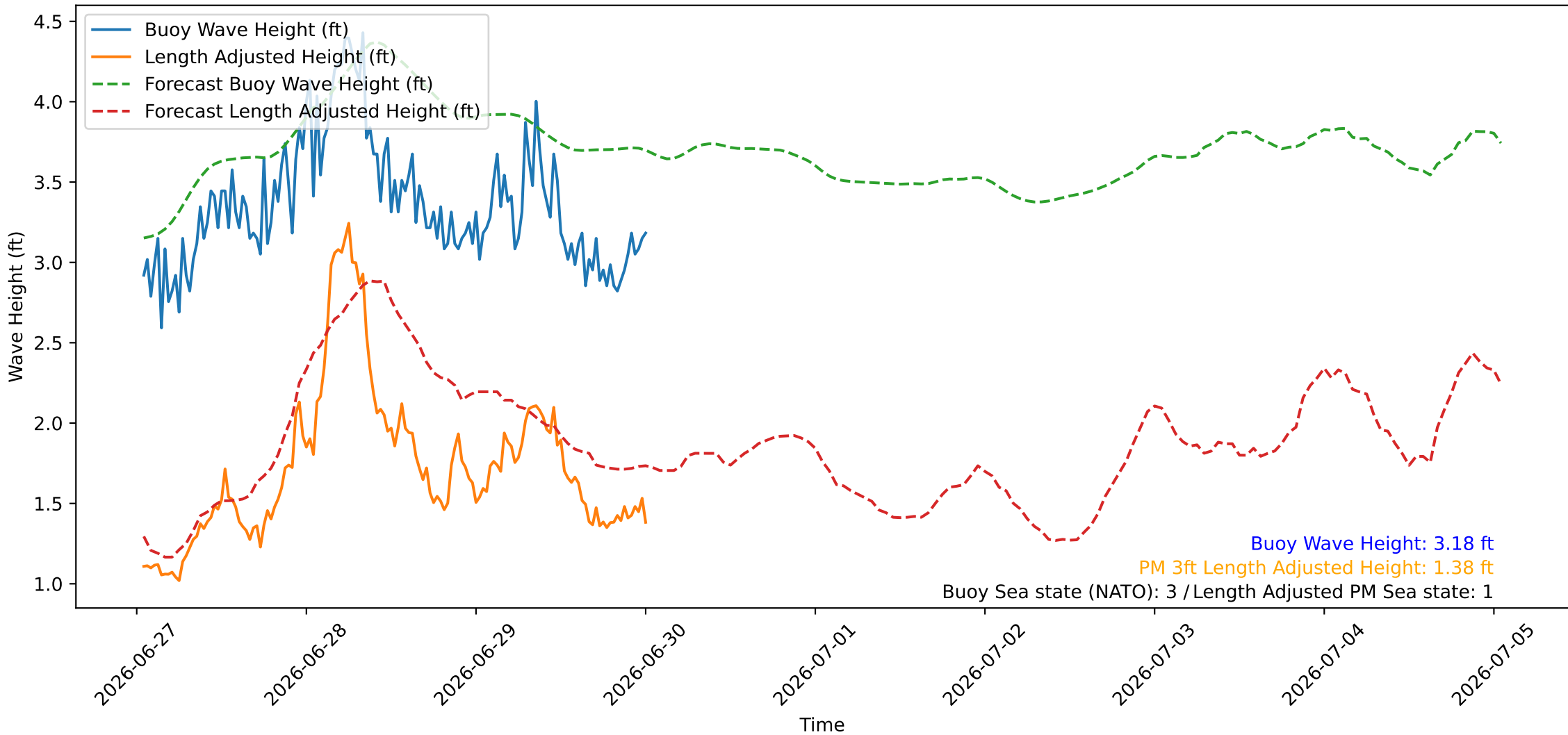
Wave Heights over Time for Oceanside Harbor at 2026-06-30 00:50:27
