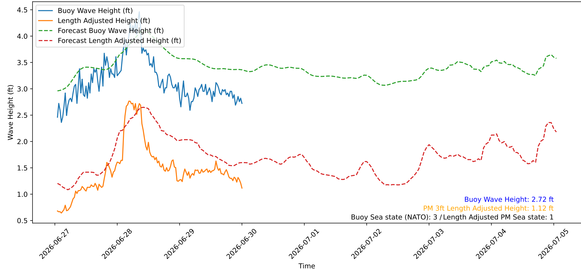
Wave Heights over Time for Red Beach at 2026-06-30 00:50:47
