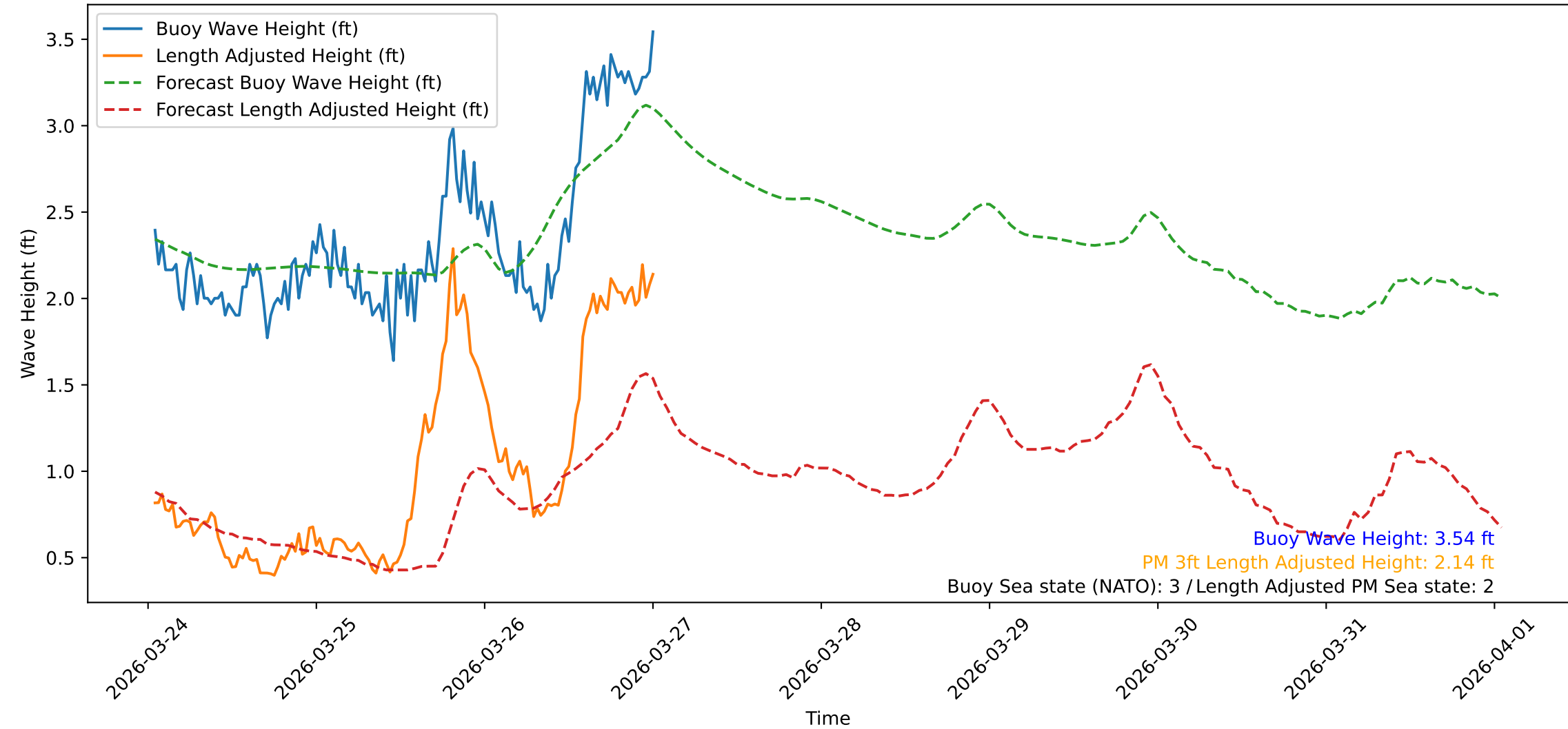
Wave Heights over Time for Green Beach at 2026-03-27 00:51:09
