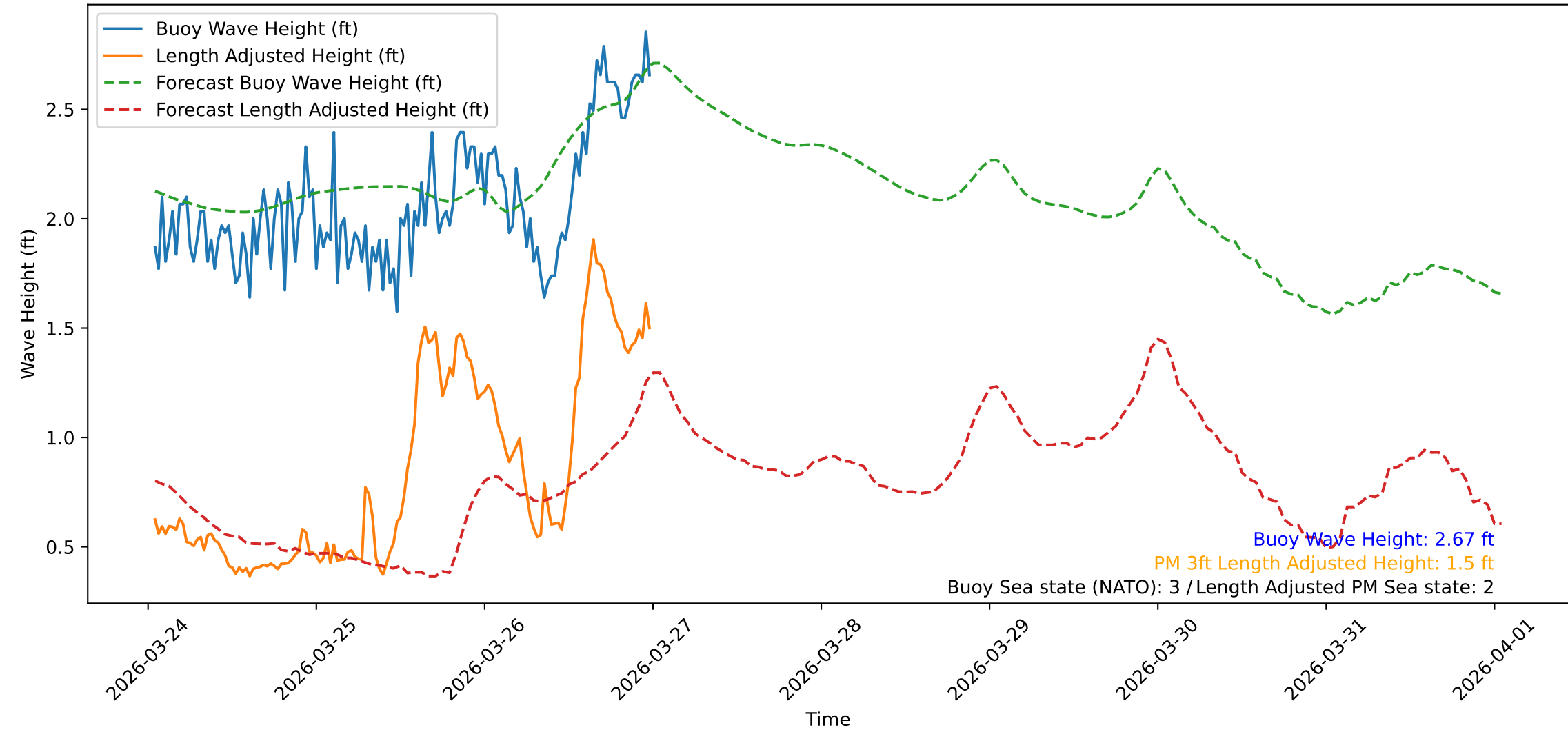
Wave Heights over Time for Red Beach at 2026-03-27 00:50:47
