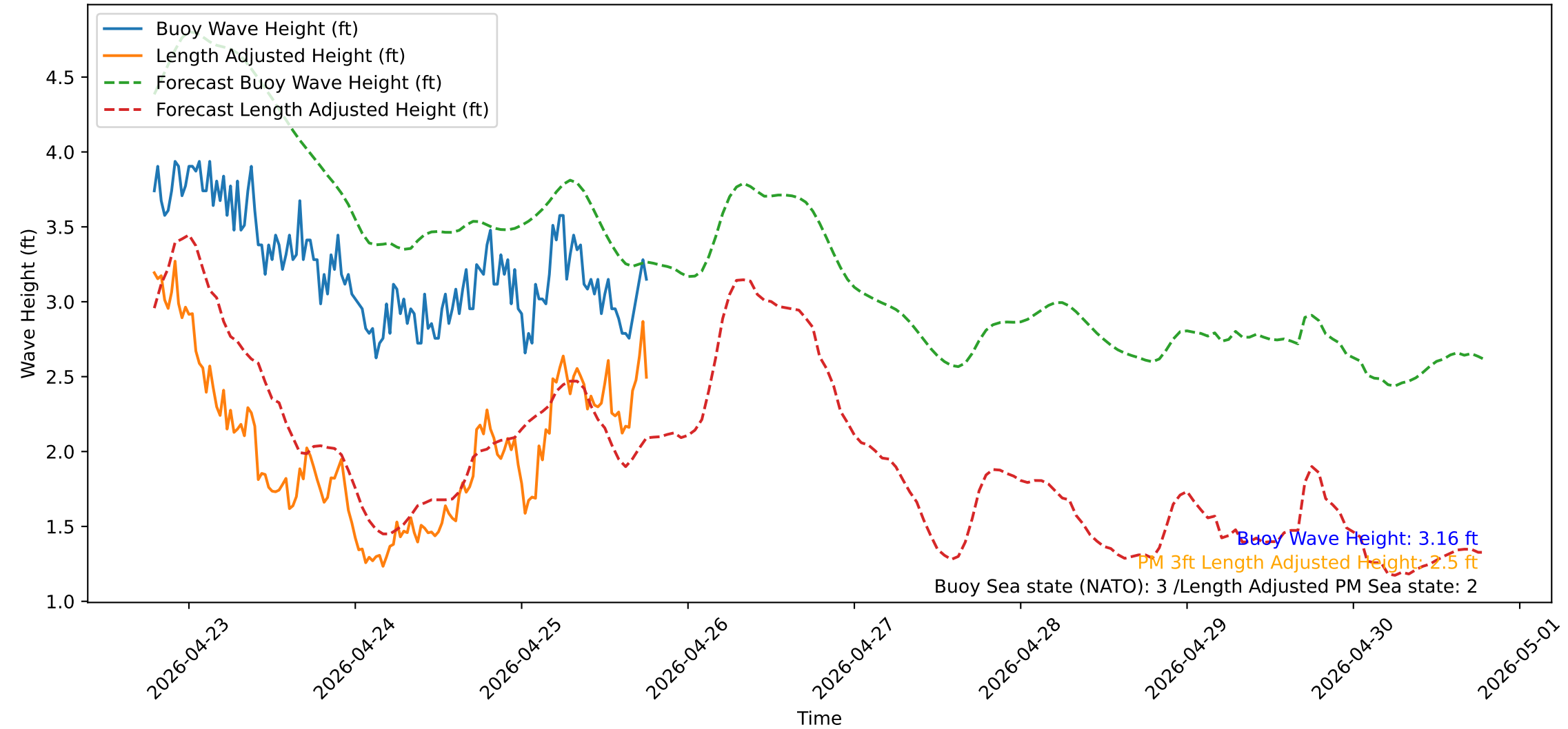
Wave Heights over Time for Green Beach at 2026-04-25 18:51:14
