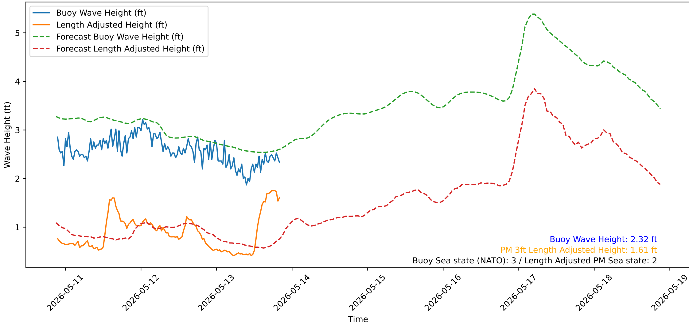
Wave Heights over Time for Red Beach at 2026-05-13 21:00:51
