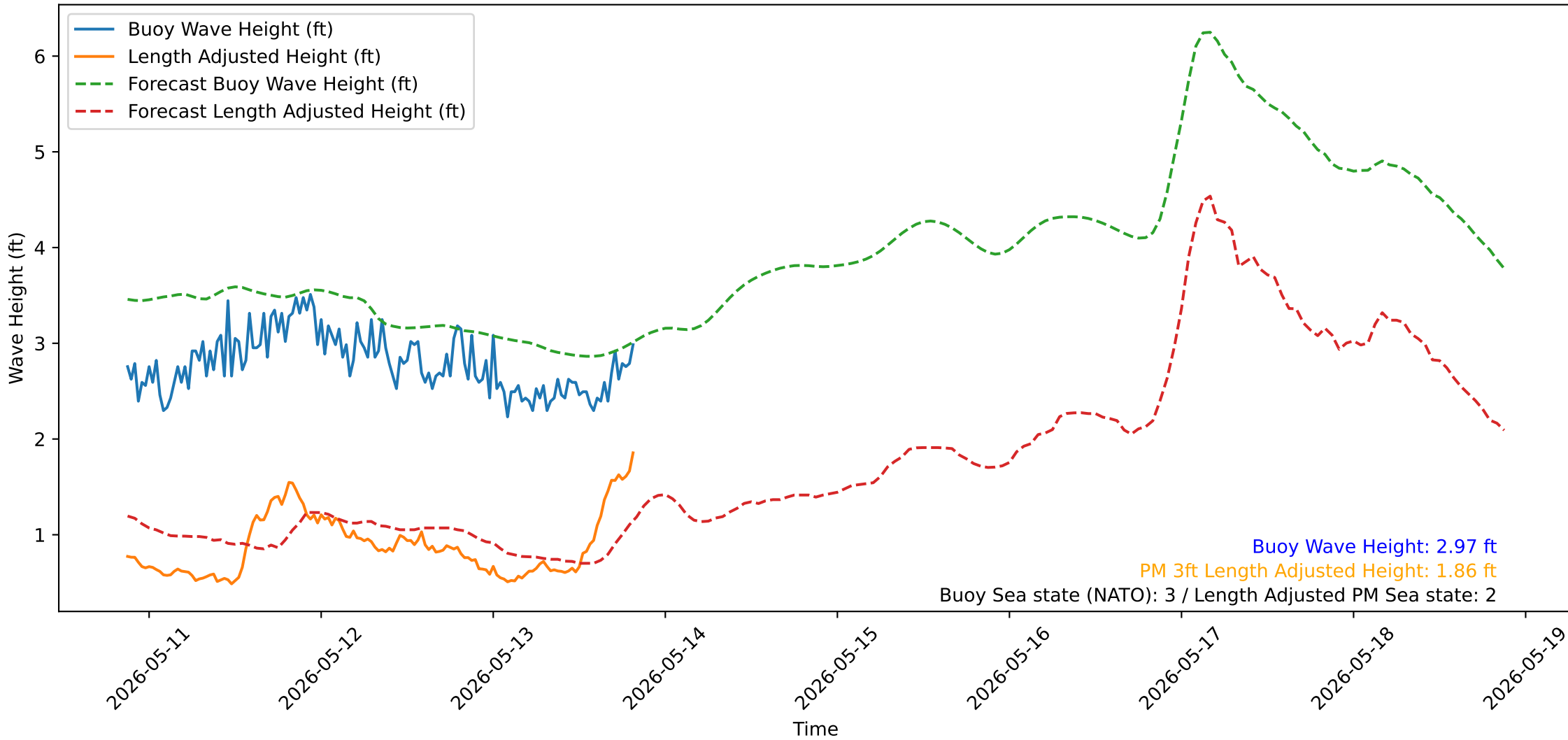
Wave Heights over Time for Green Beach at 2026-05-13 21:01:13
