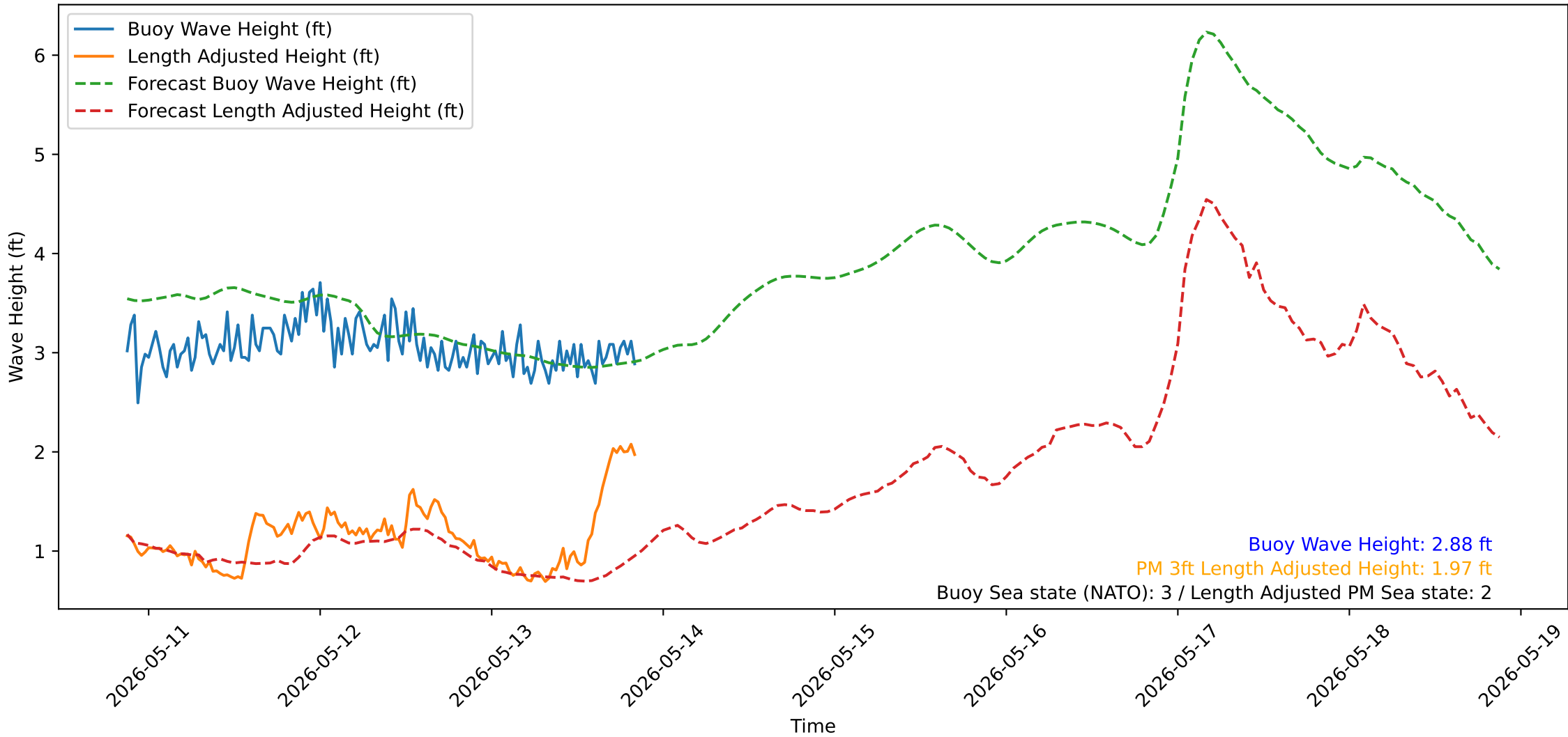
Wave Heights over Time for Oceanside Harbor at 2026-05-13 21:00:32
