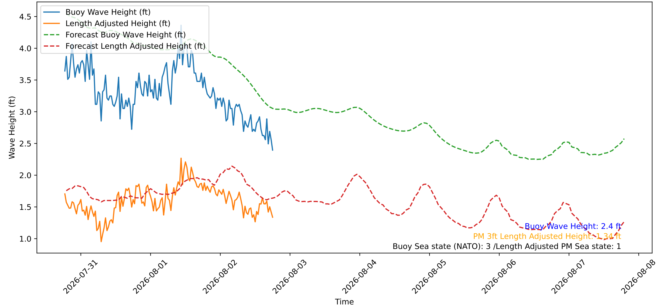
Wave Heights over Time for Oceanside Harbor at 2026-08-02 18:40:26
