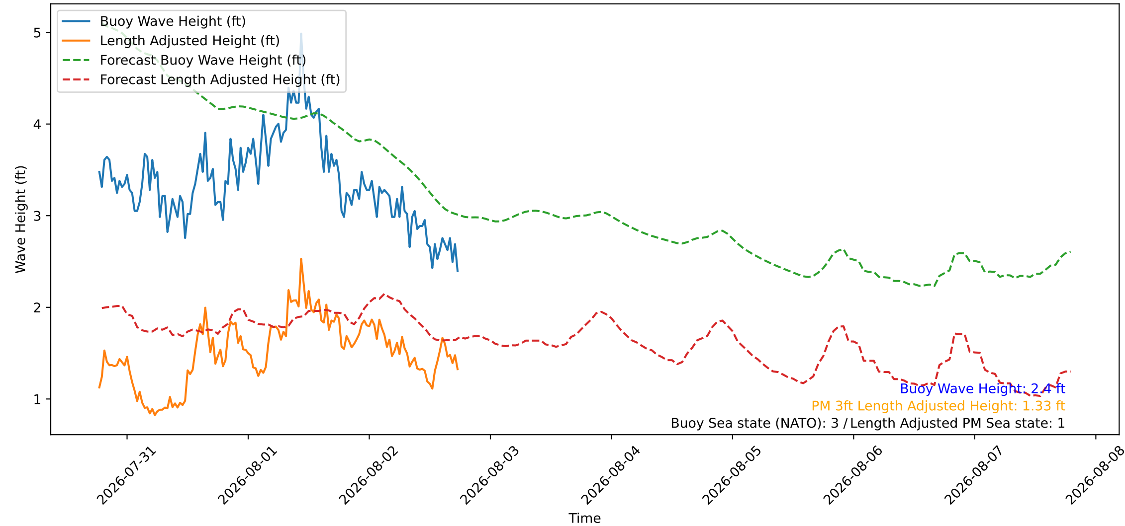
Wave Heights over Time for Green Beach at 2026-08-02 18:41:09
