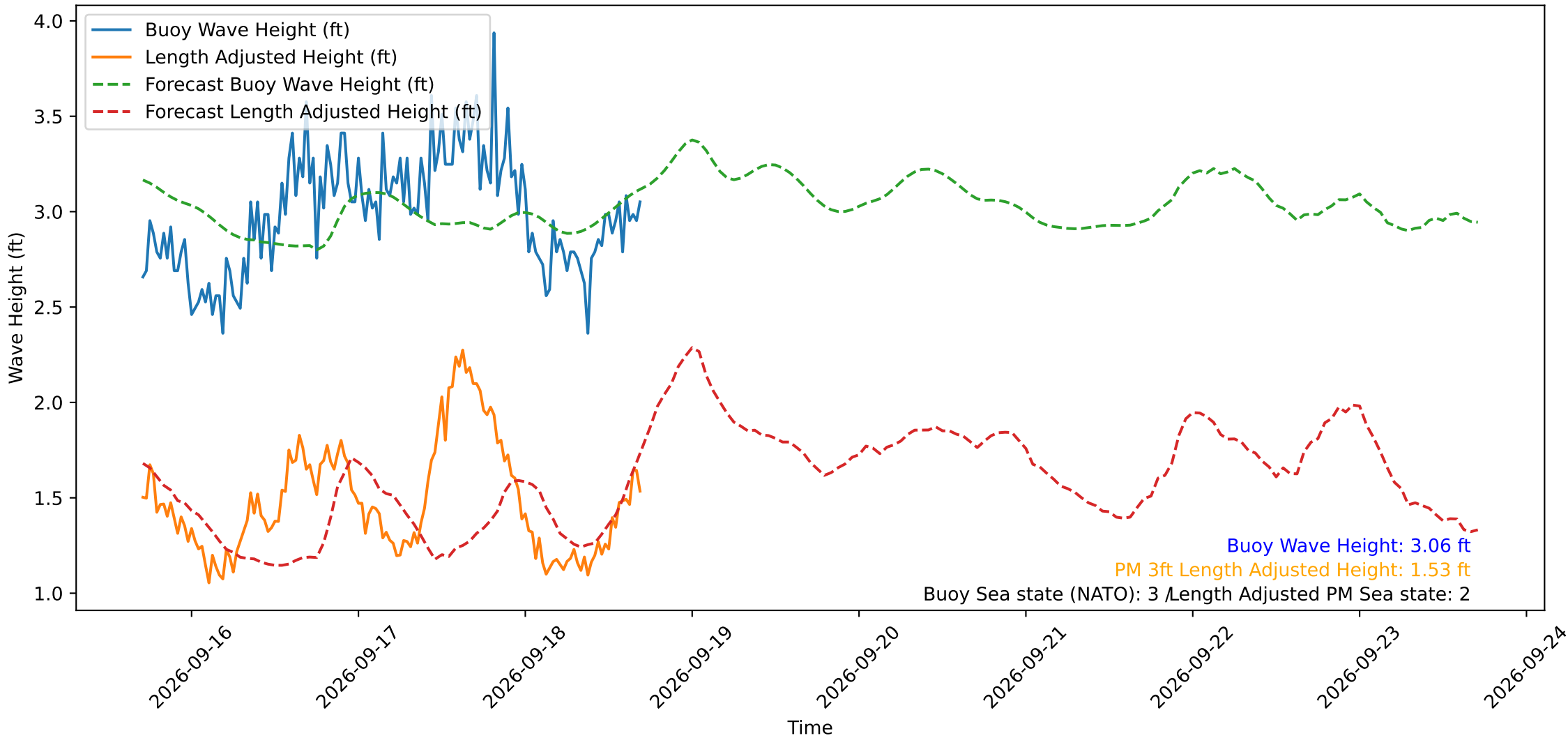
Wave Heights over Time for Oceanside Harbor at 2026-09-18 17:10:31
