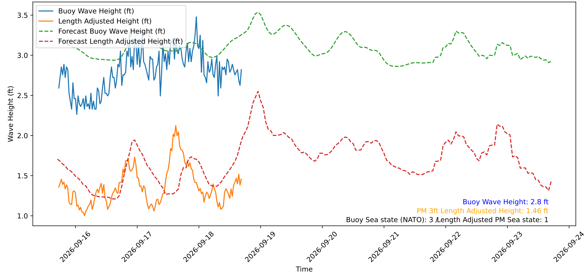
Wave Heights over Time for Green Beach at 2026-09-18 17:11:17
