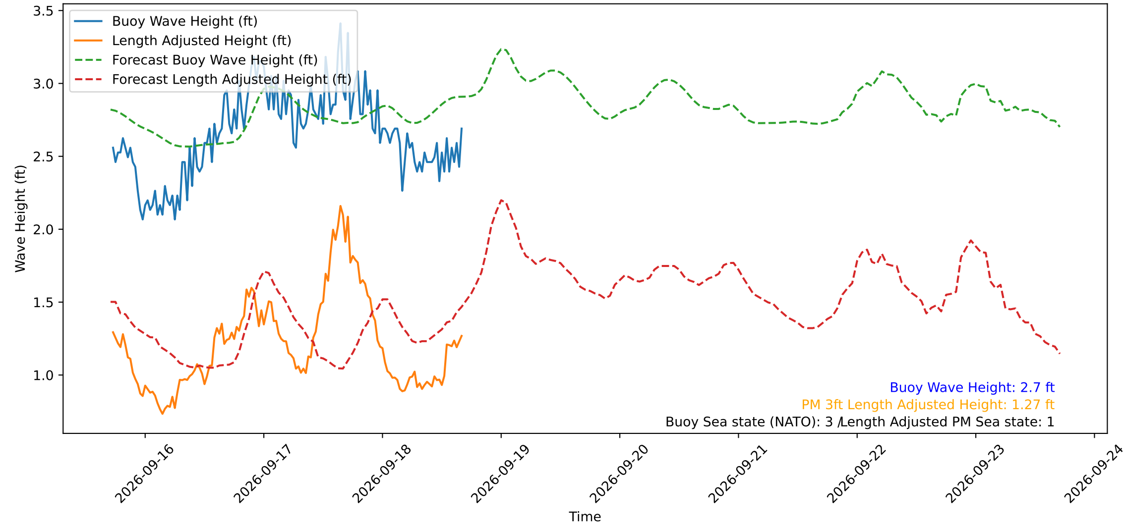
Wave Heights over Time for Red Beach at 2026-09-18 17:10:52
