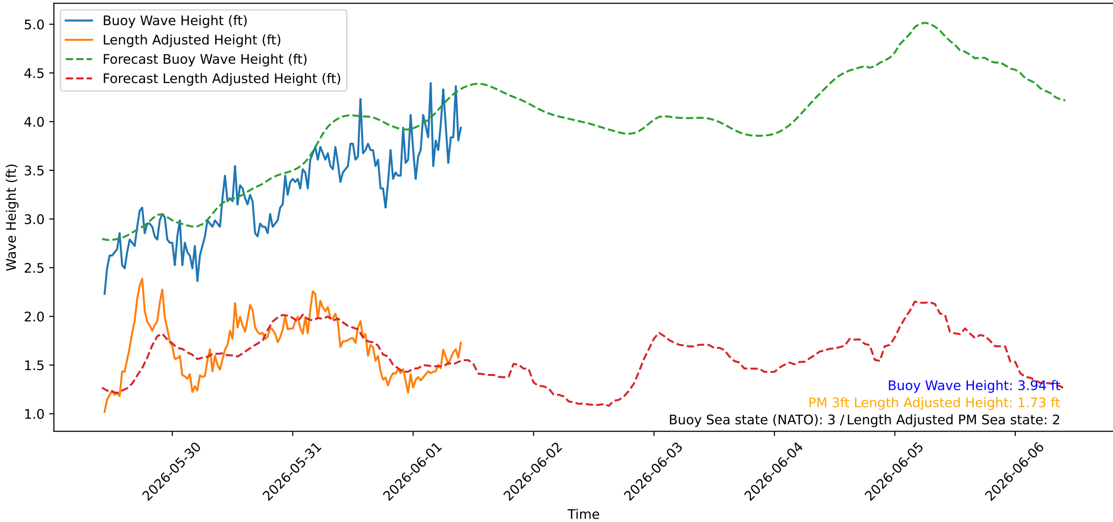
Wave Heights over Time for Oceanside Harbor at 2026-06-01 10:20:26
