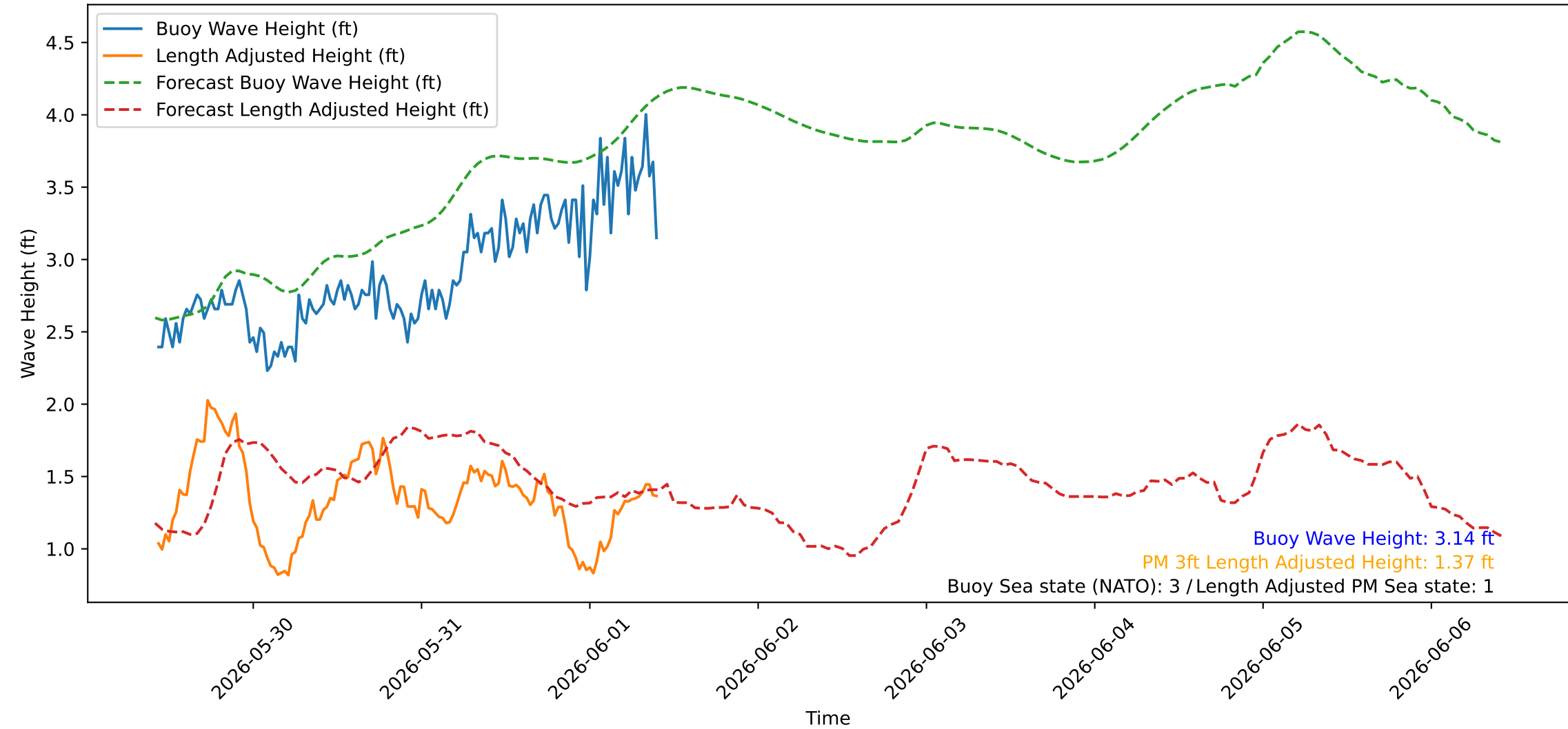
Wave Heights over Time for Red Beach at 2026-06-01 10:20:46
