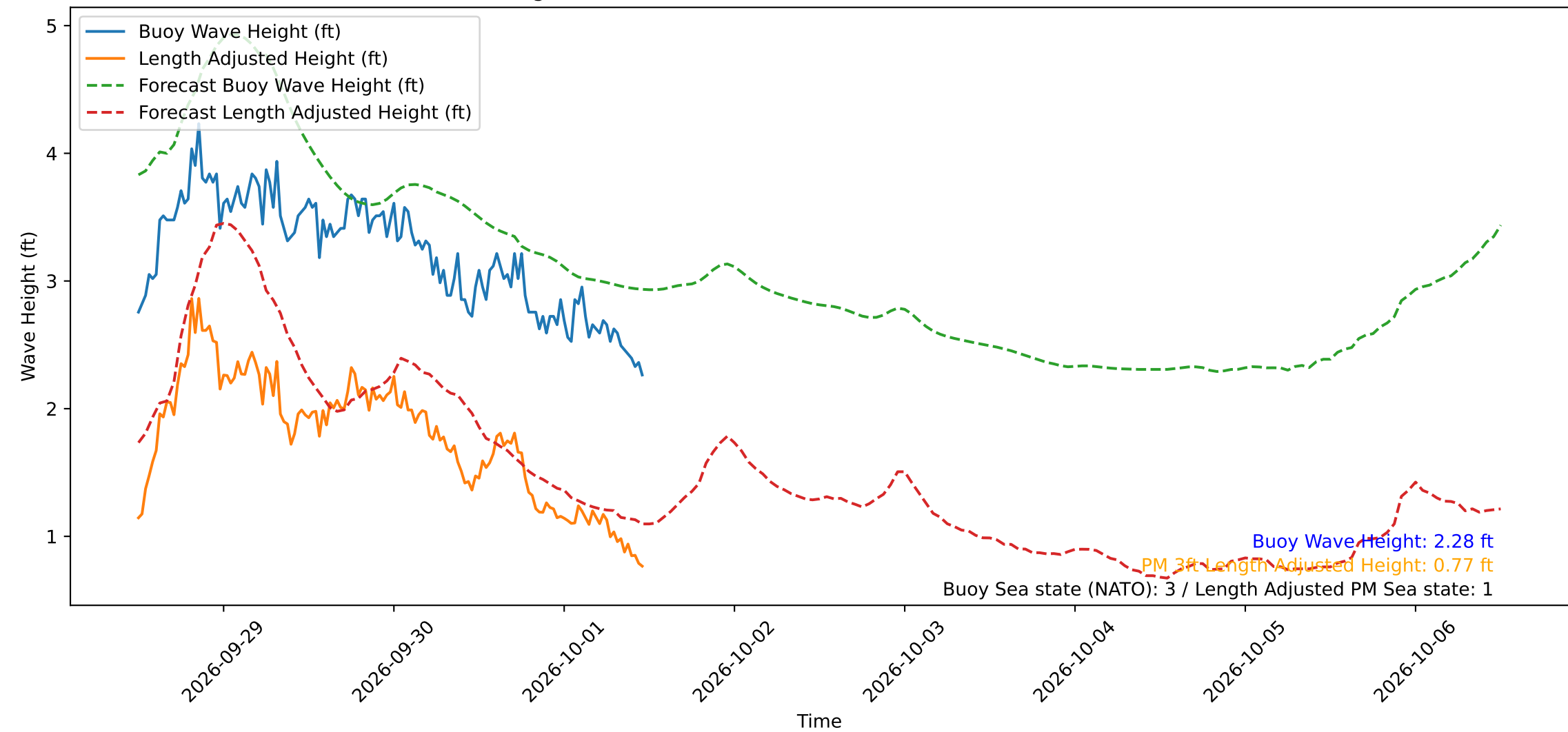
Wave Heights over Time for Oceanside Harbor at 2026-10-01 11:50:29
