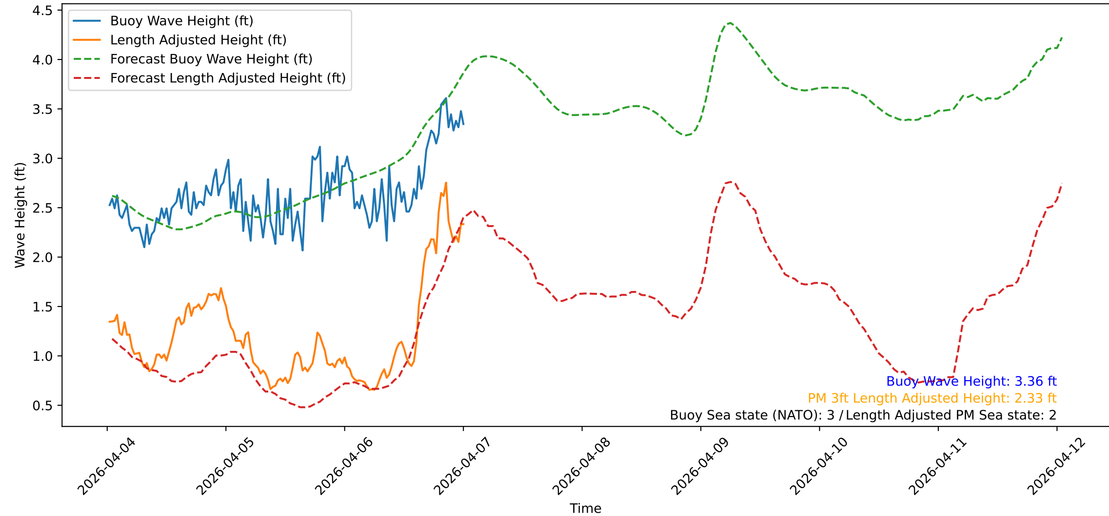
Wave Heights over Time for Oceanside Harbor at 2026-04-07 00:30:30
