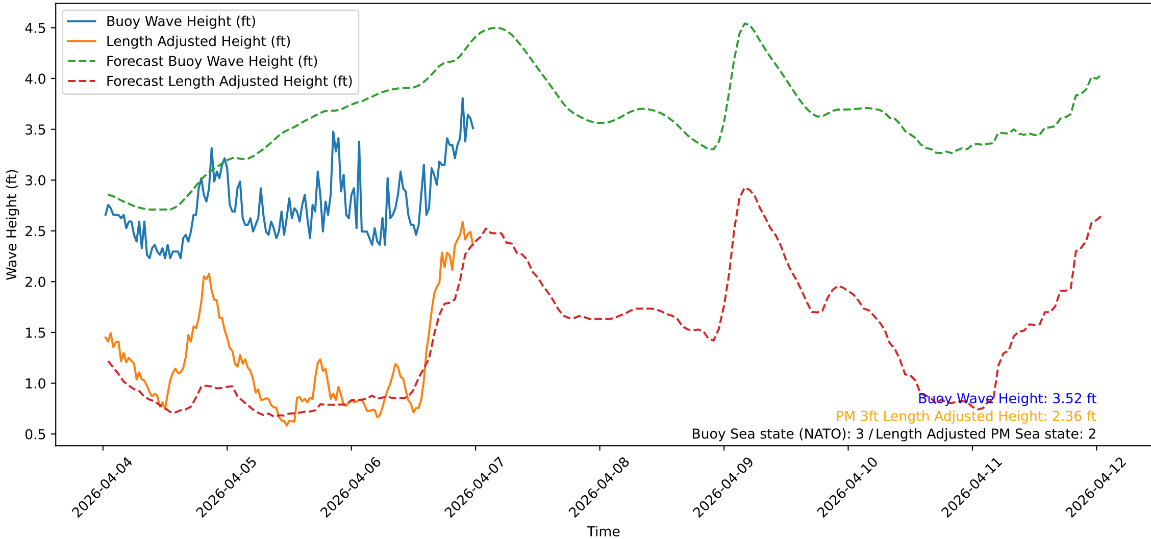
Wave Heights over Time for Green Beach at 2026-04-07 00:31:08
