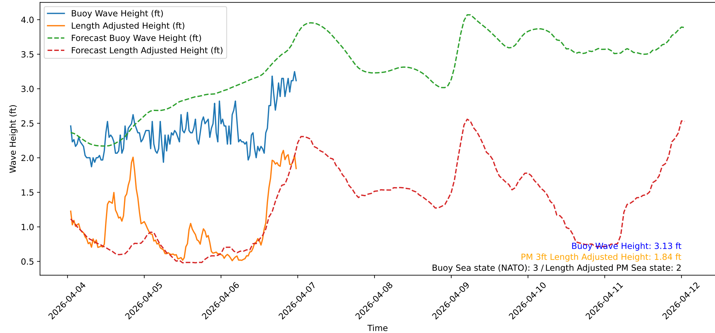
Wave Heights over Time for Red Beach at 2026-04-07 00:30:46
