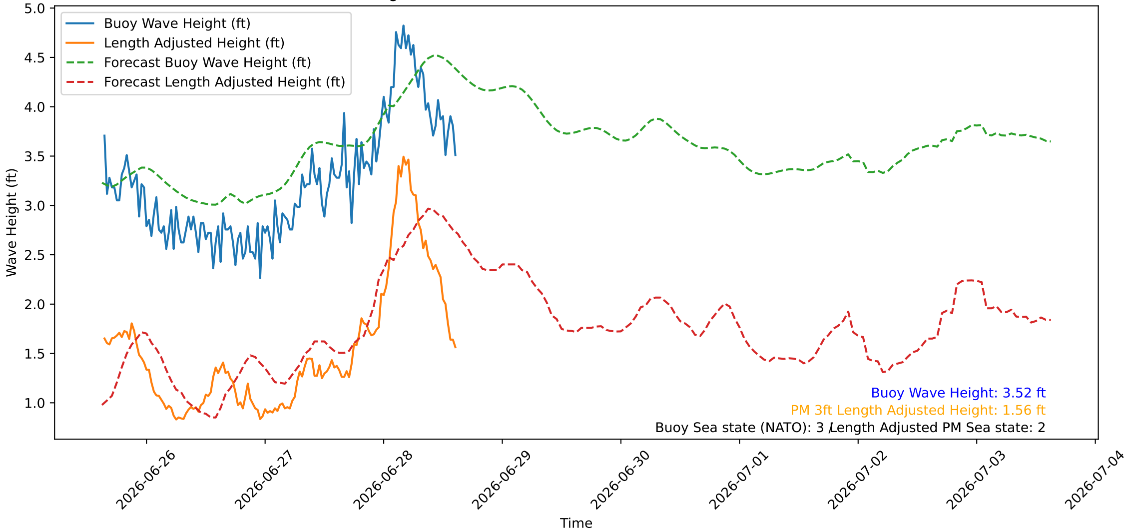
Wave Heights over Time for Green Beach at 2026-06-28 15:21:10
