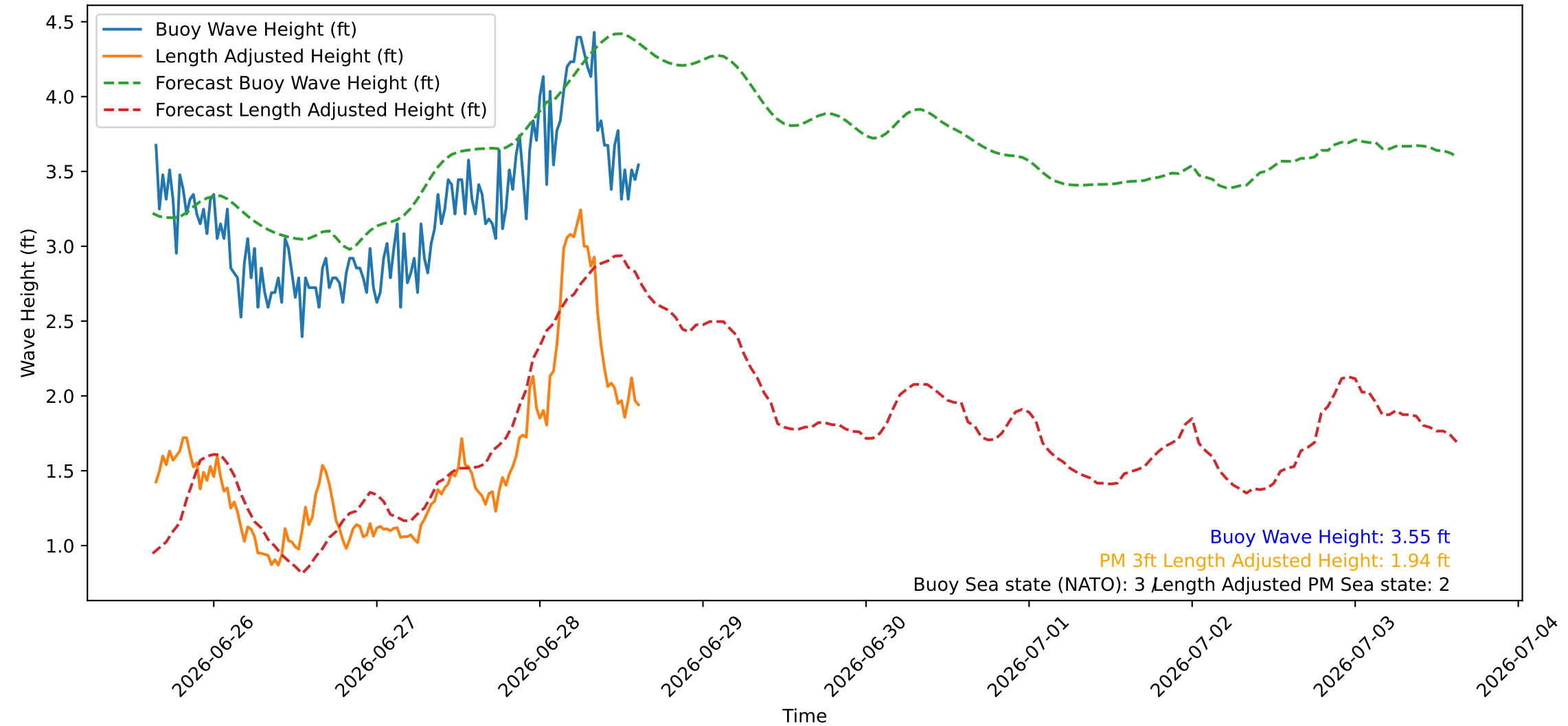
Wave Heights over Time for Oceanside Harbor at 2026-06-28 15:20:26
