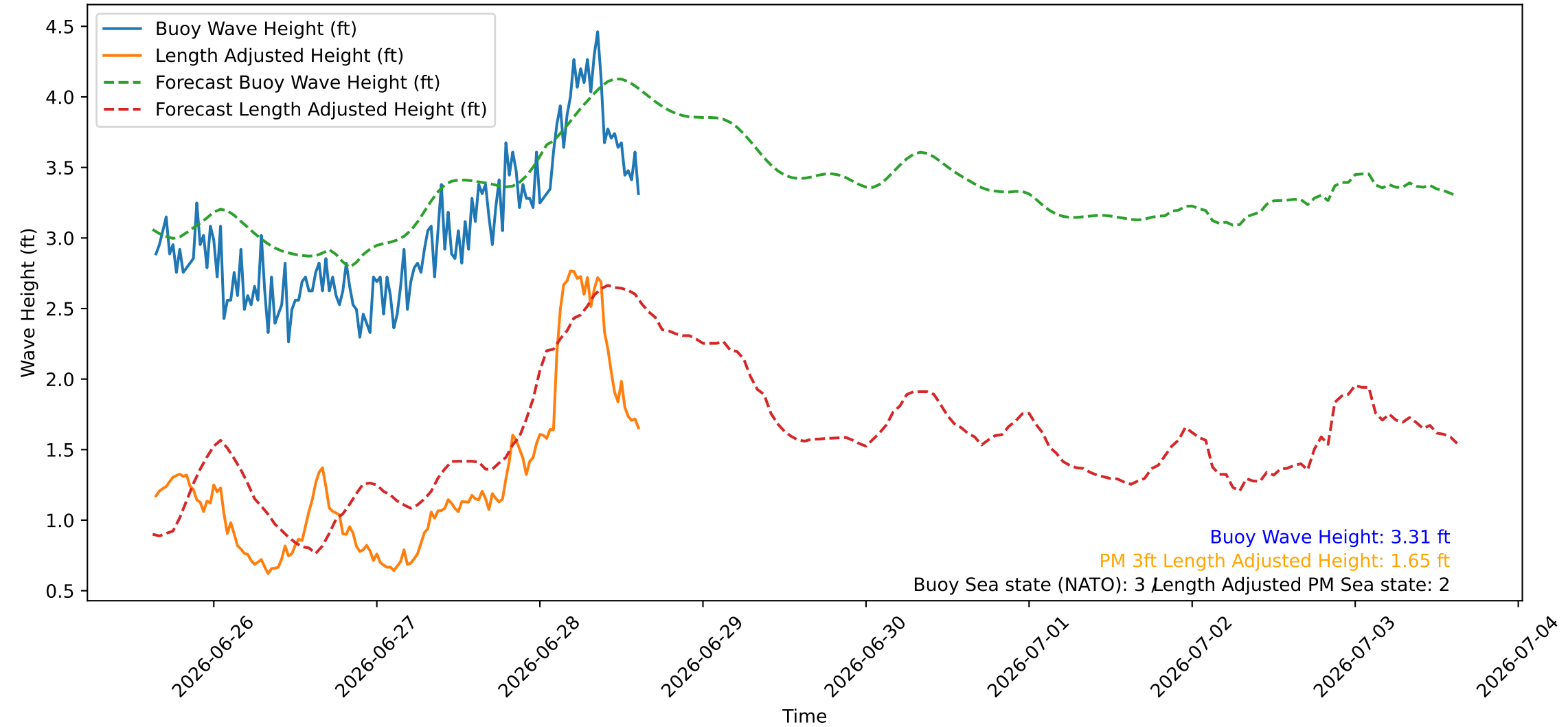
Wave Heights over Time for Red Beach at 2026-06-28 15:20:47
