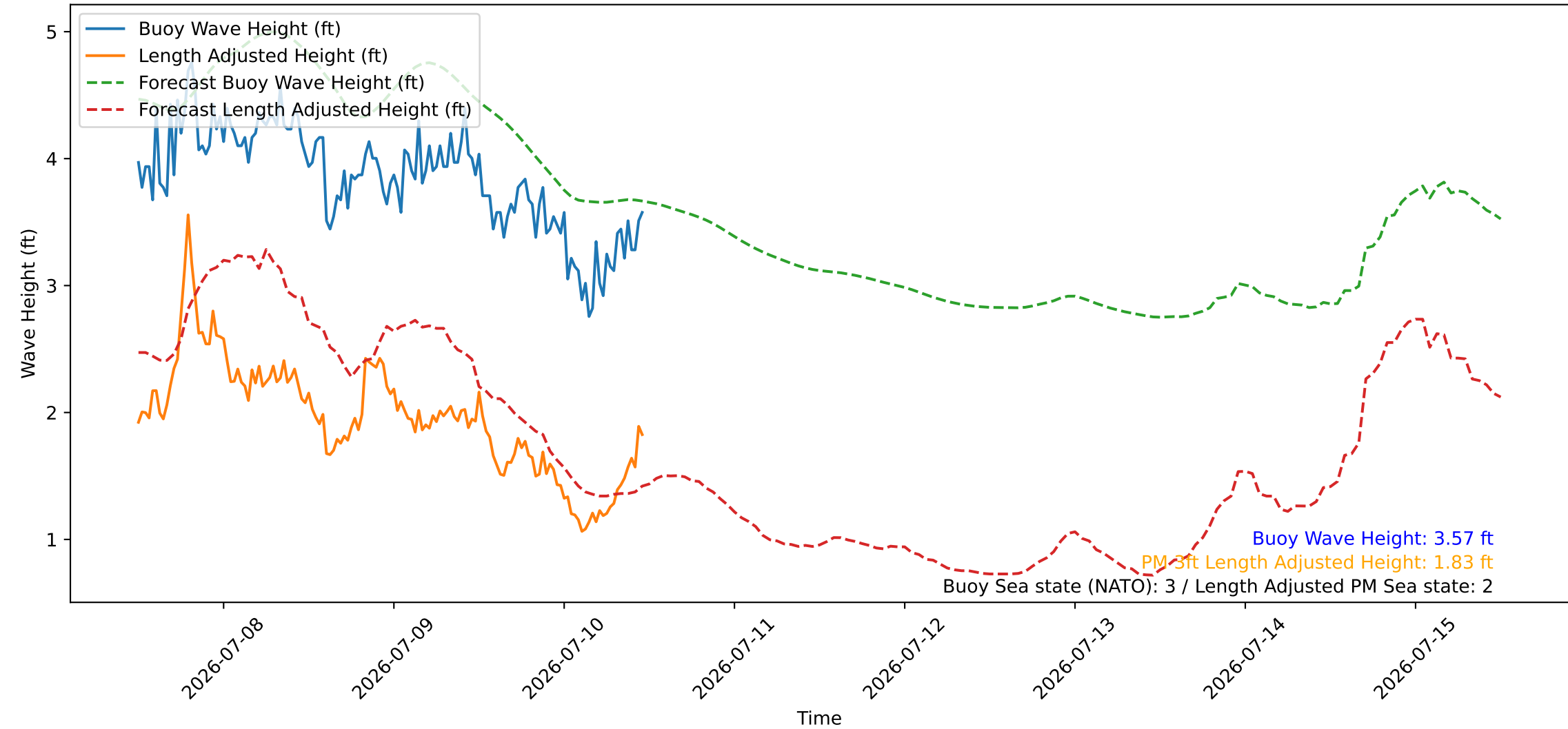
Wave Heights over Time for Green Beach at 2026-07-10 12:01:08
