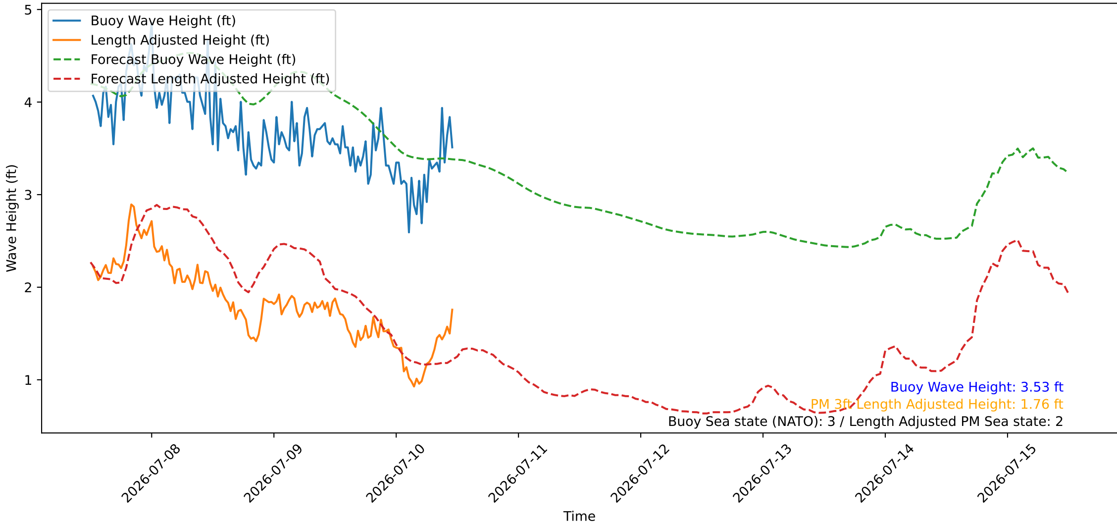
Wave Heights over Time for Red Beach at 2026-07-10 12:00:46
