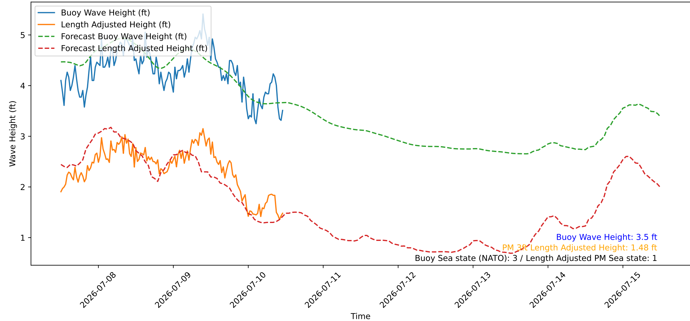
Wave Heights over Time for Oceanside Harbor at 2026-07-10 12:00:26
