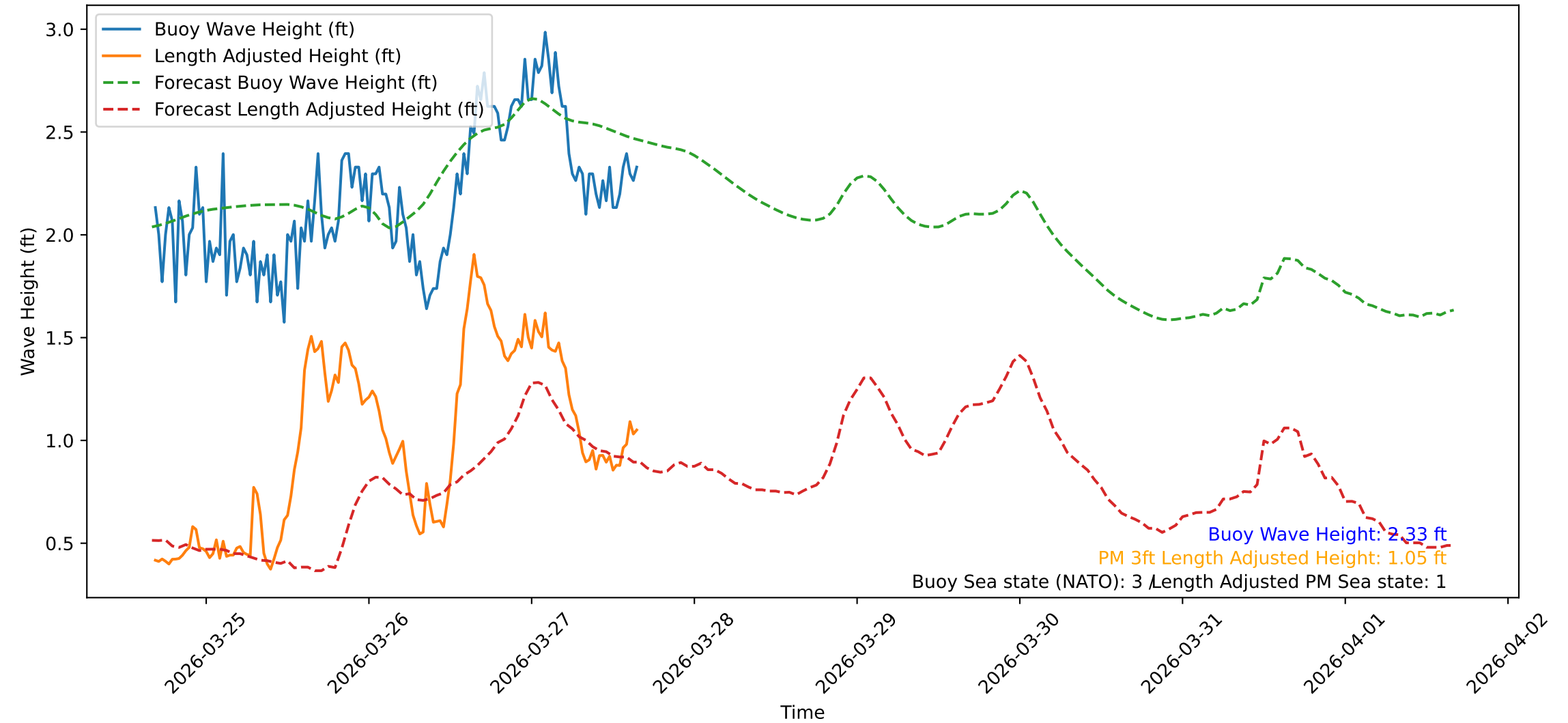
Wave Heights over Time for Red Beach at 2026-03-27 16:10:47
