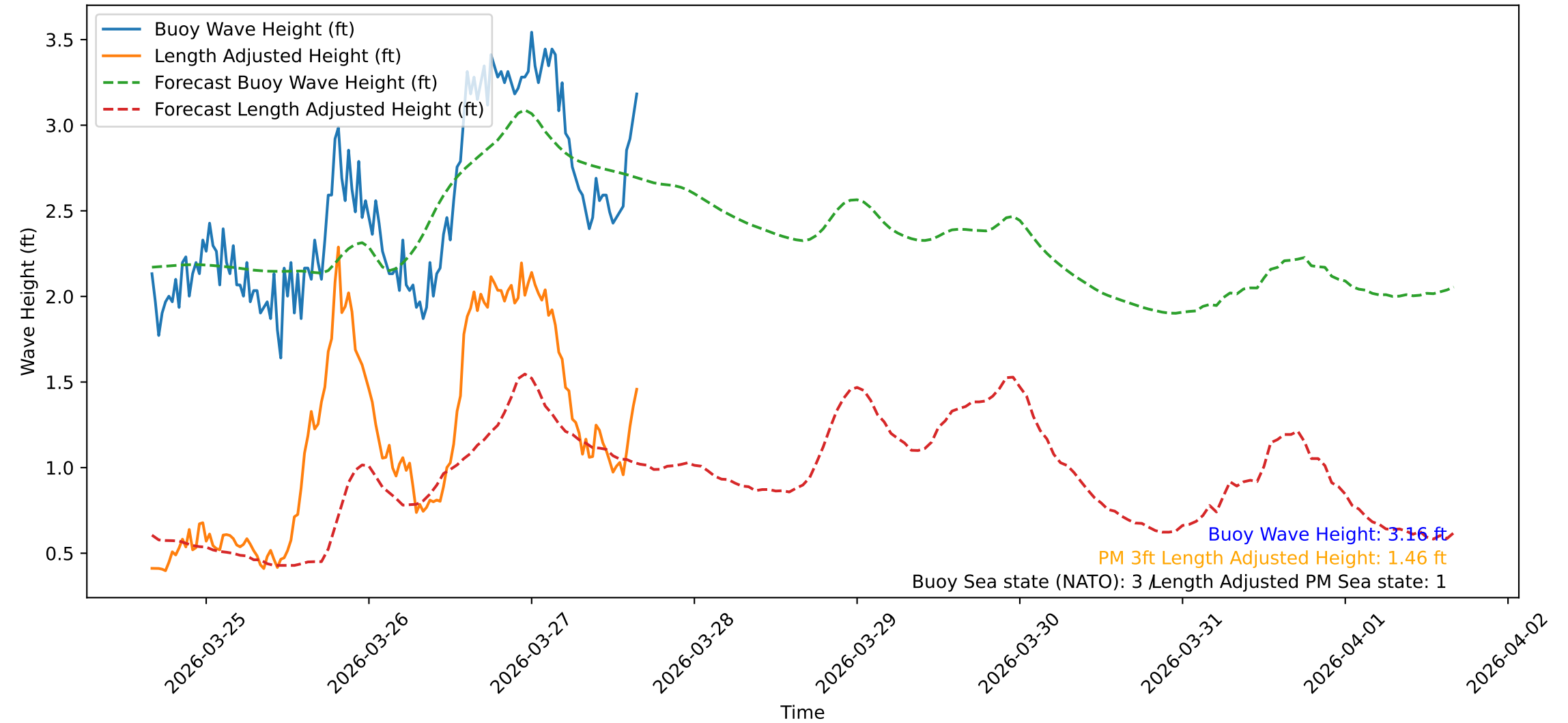
Wave Heights over Time for Green Beach at 2026-03-27 16:11:09
