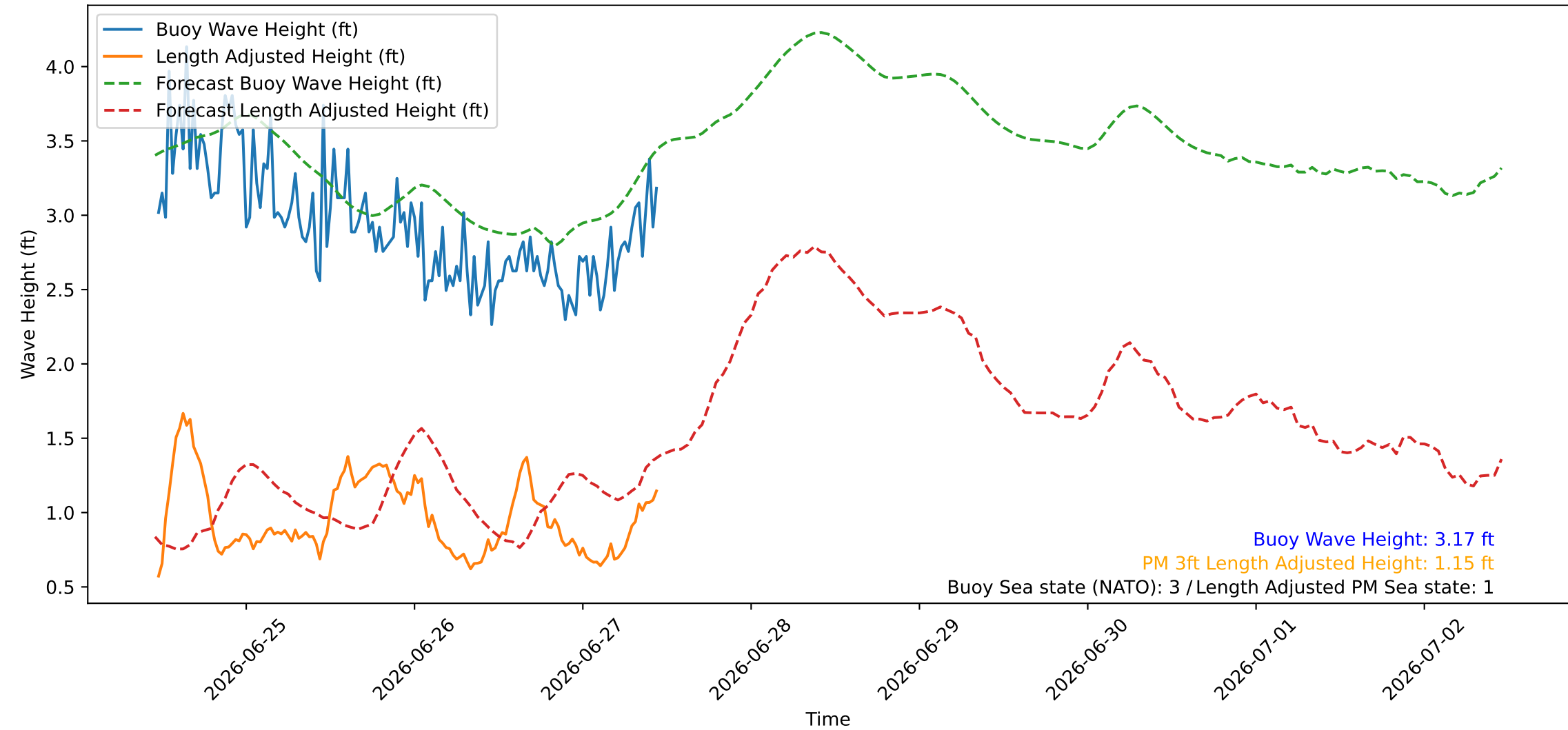
Wave Heights over Time for Red Beach at 2026-06-27 11:10:45
