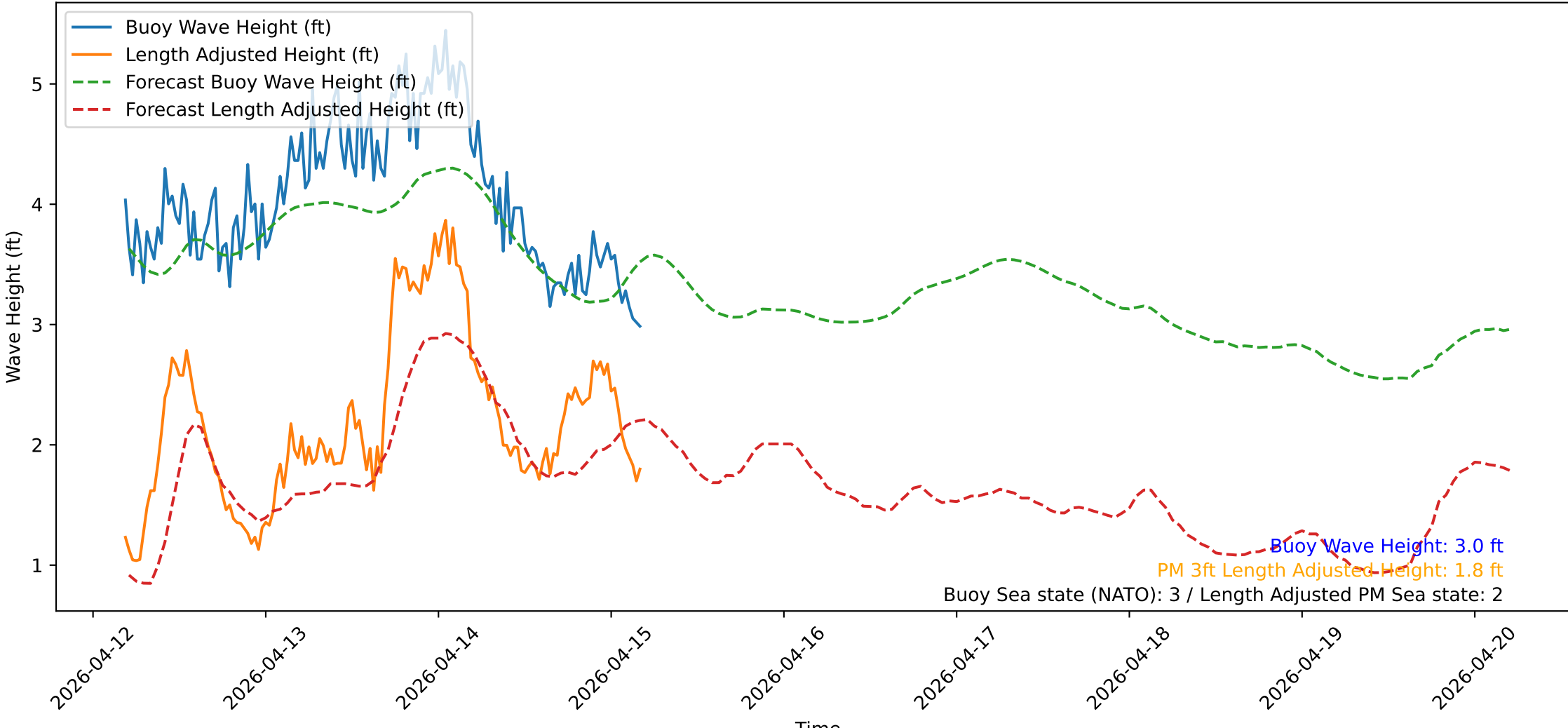
Wave Heights over Time for Oceanside Harbor at 2026-04-15 04:40:31
