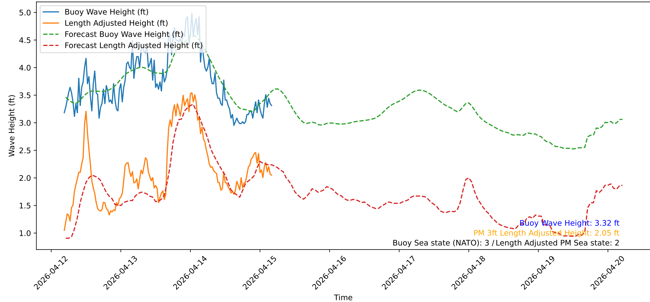
Wave Heights over Time for Green Beach at 2026-04-15 04:41:12
