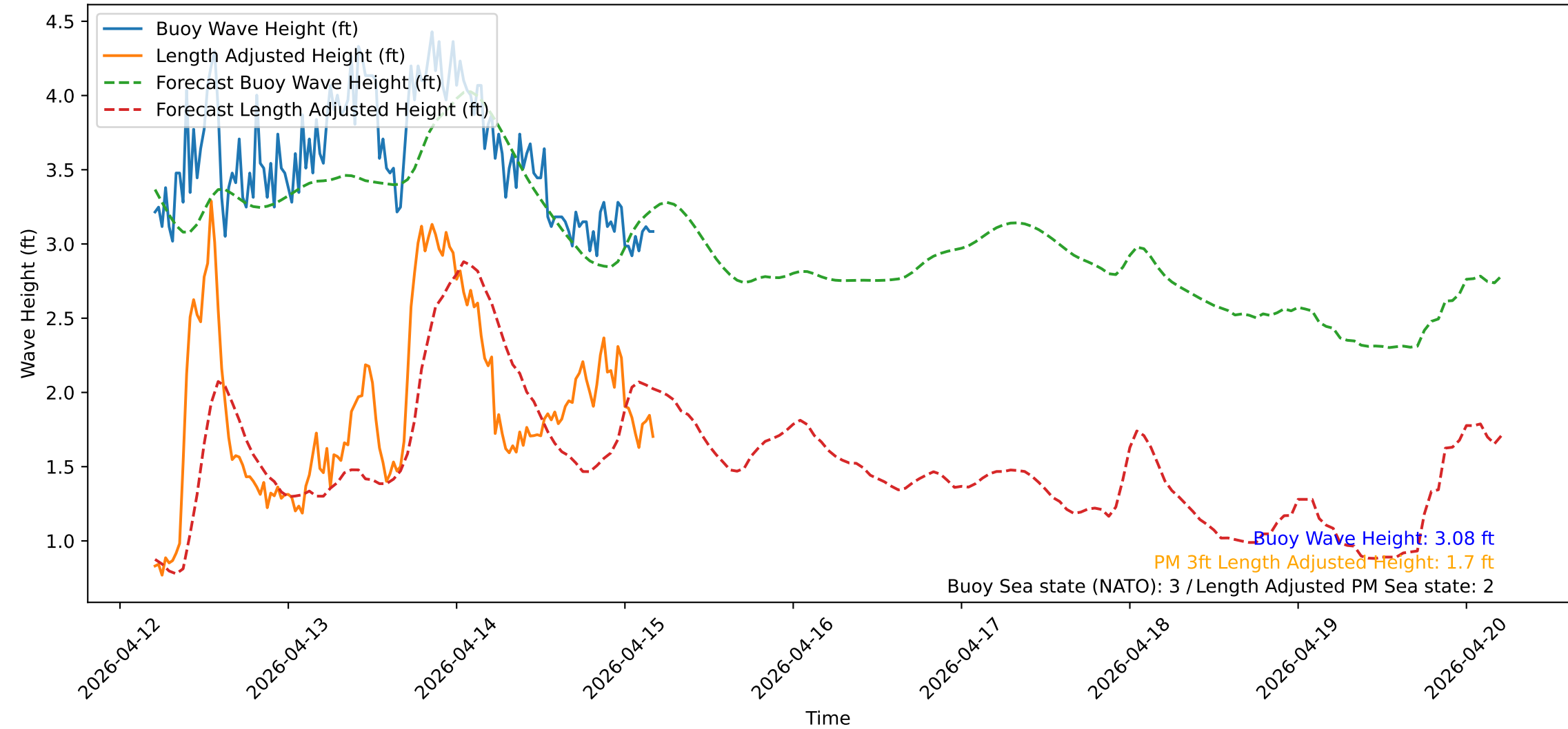
Wave Heights over Time for Red Beach at 2026-04-15 04:40:49
