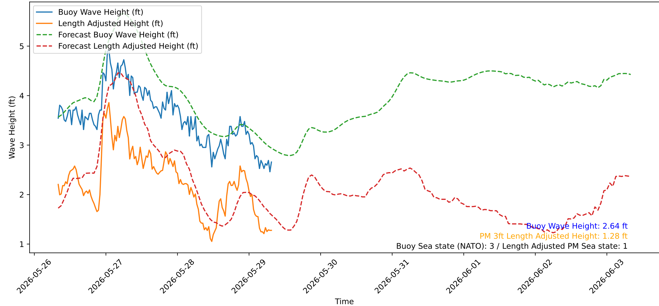
Wave Heights over Time for Green Beach at 2026-05-29 08:11:03
