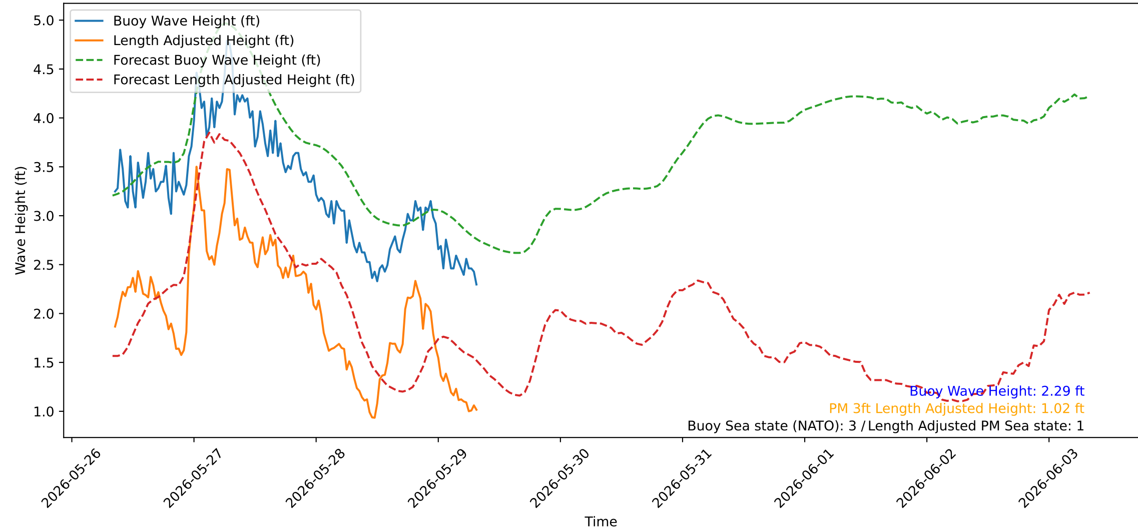
Wave Heights over Time for Red Beach at 2026-05-29 08:10:40
