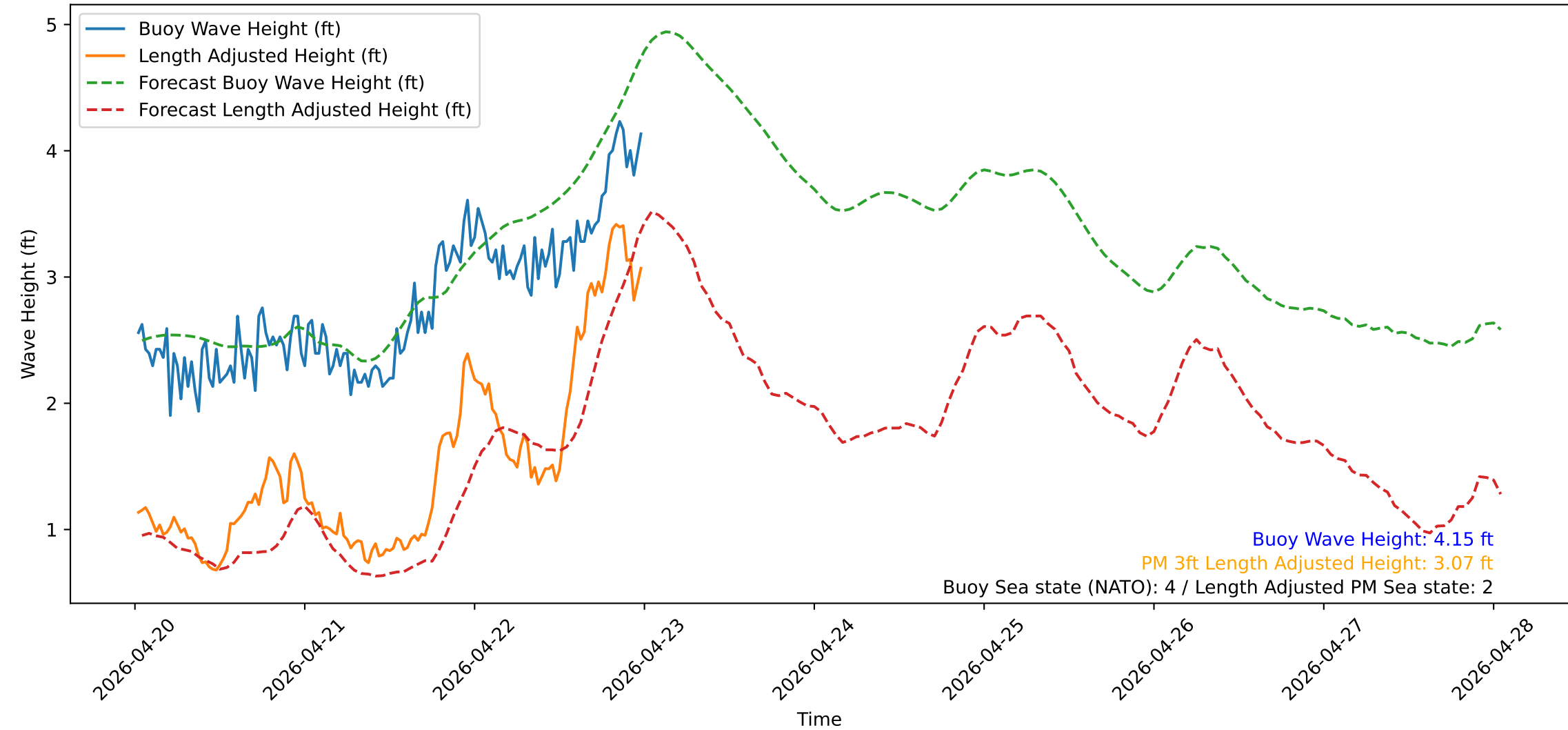
Wave Heights over Time for Oceanside Harbor at 2026-04-23 00:30:31
