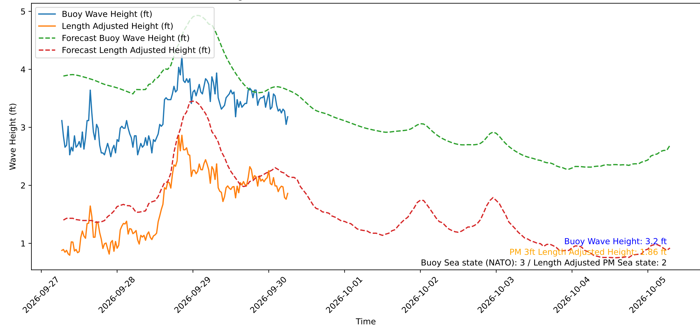
Wave Heights over Time for Oceanside Harbor at 2026-09-30 06:40:30
