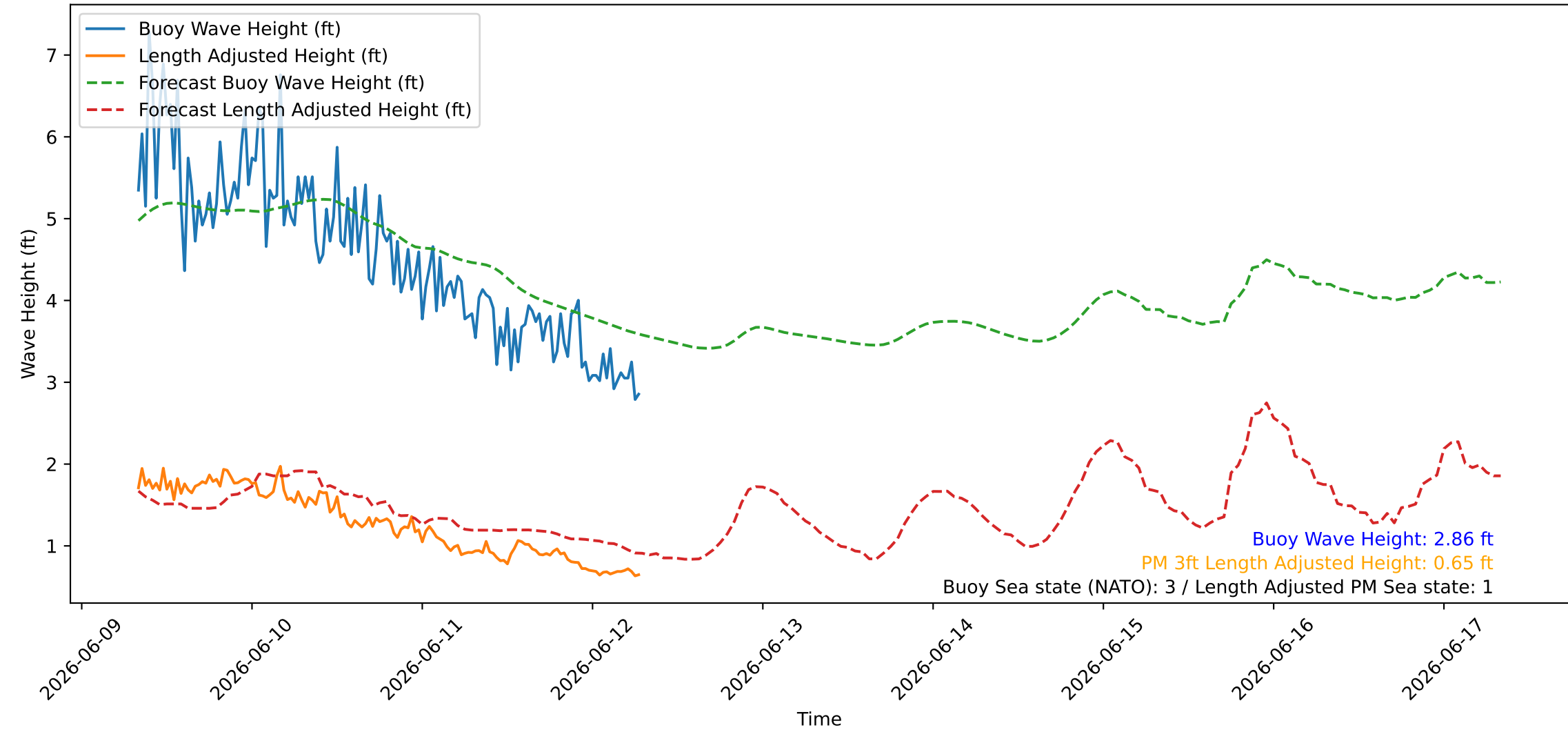
Wave Heights over Time for Red Beach at 2026-06-12 07:30:46
