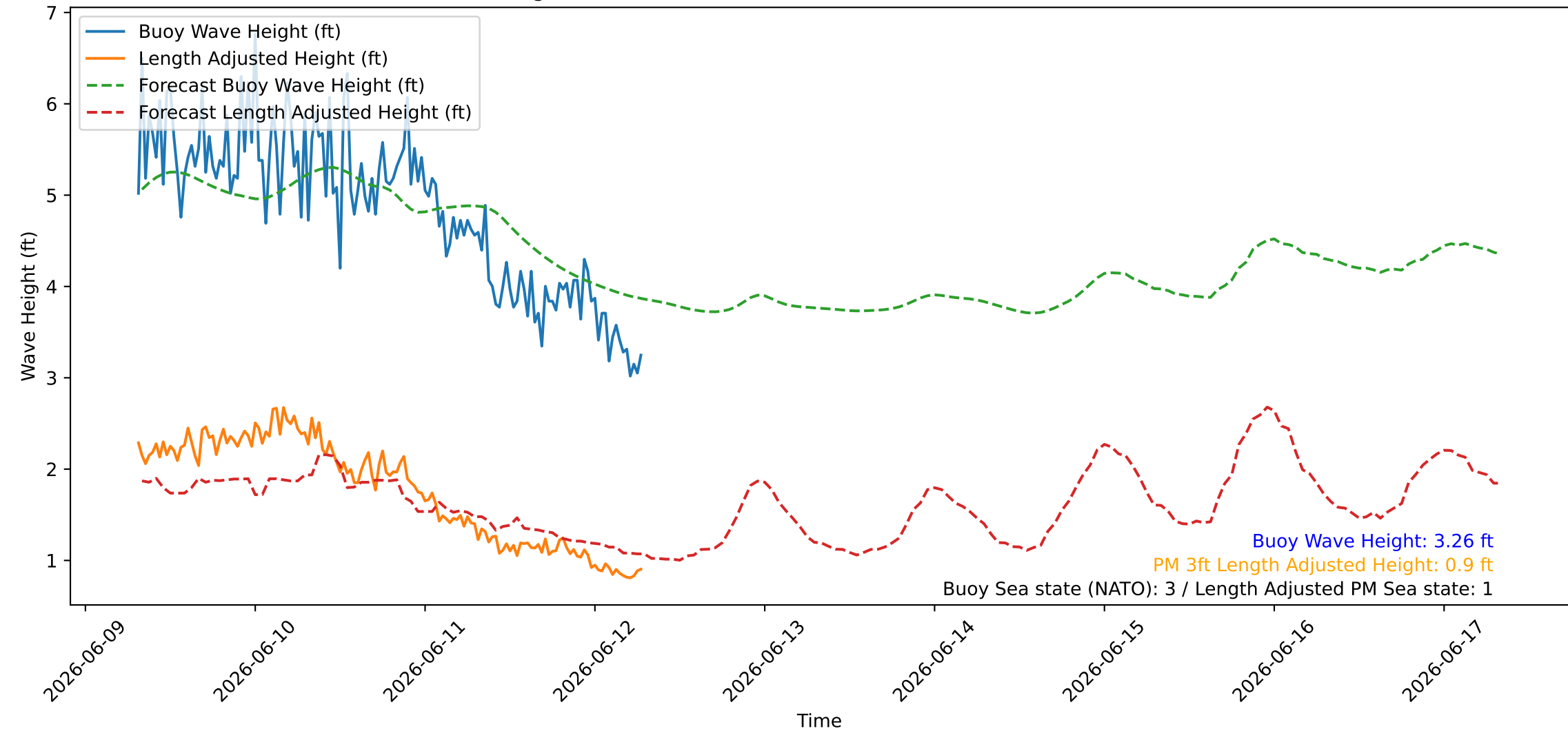
Wave Heights over Time for Oceanside Harbor at 2026-06-12 07:30:27
