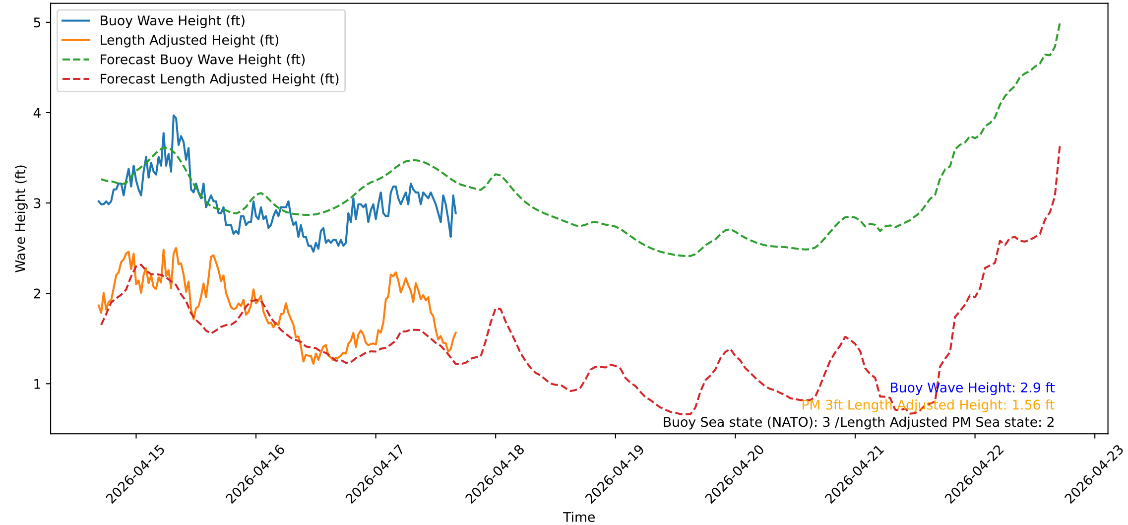
Wave Heights over Time for Green Beach at 2026-04-17 16:41:14
