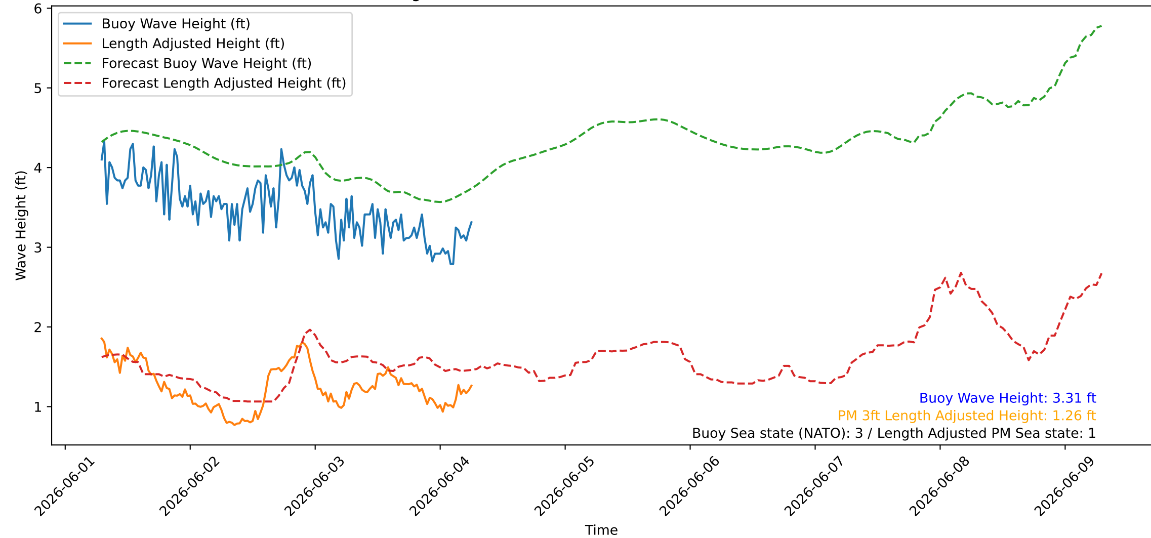
Wave Heights over Time for Green Beach at 2026-06-04 07:01:08
