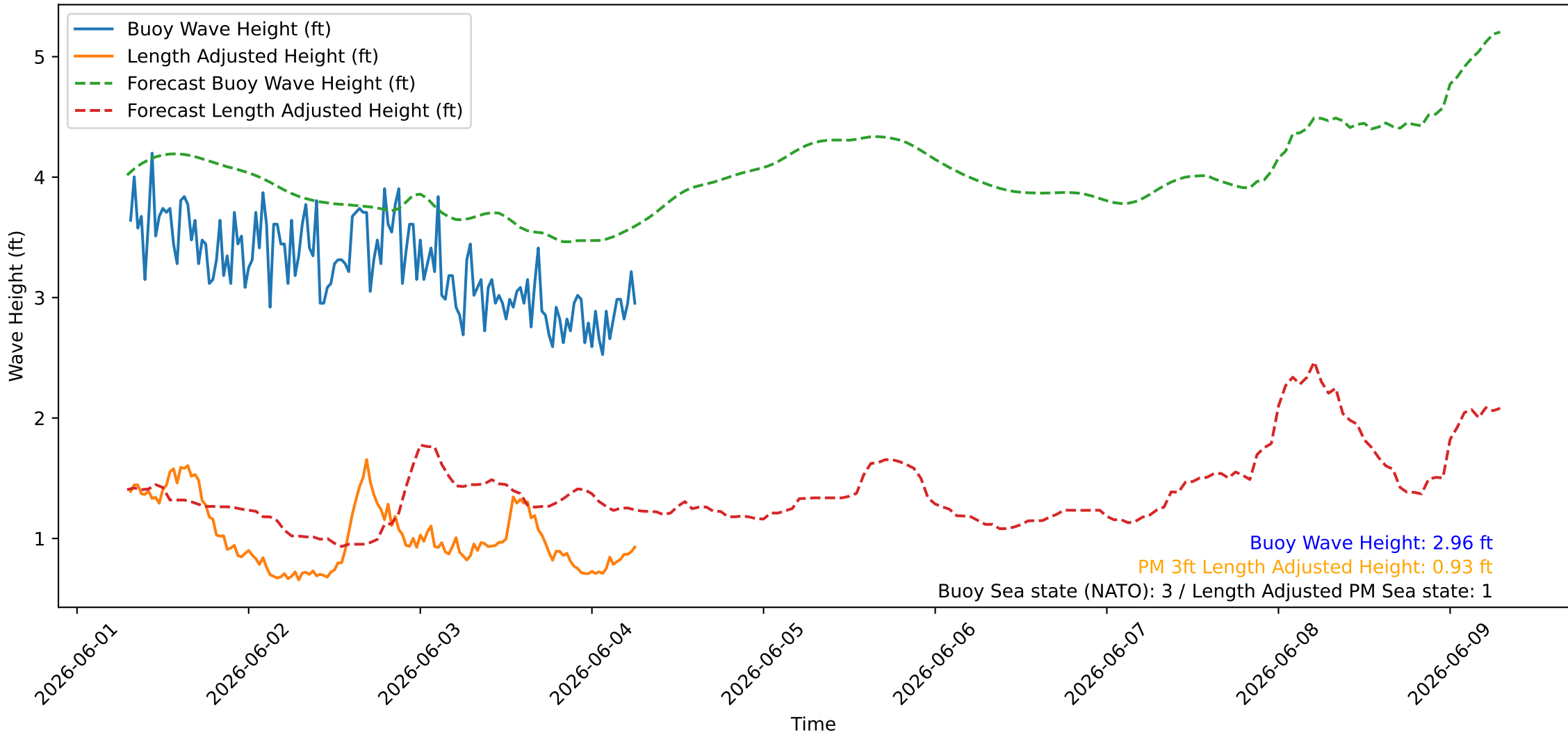
Wave Heights over Time for Red Beach at 2026-06-04 07:00:46
