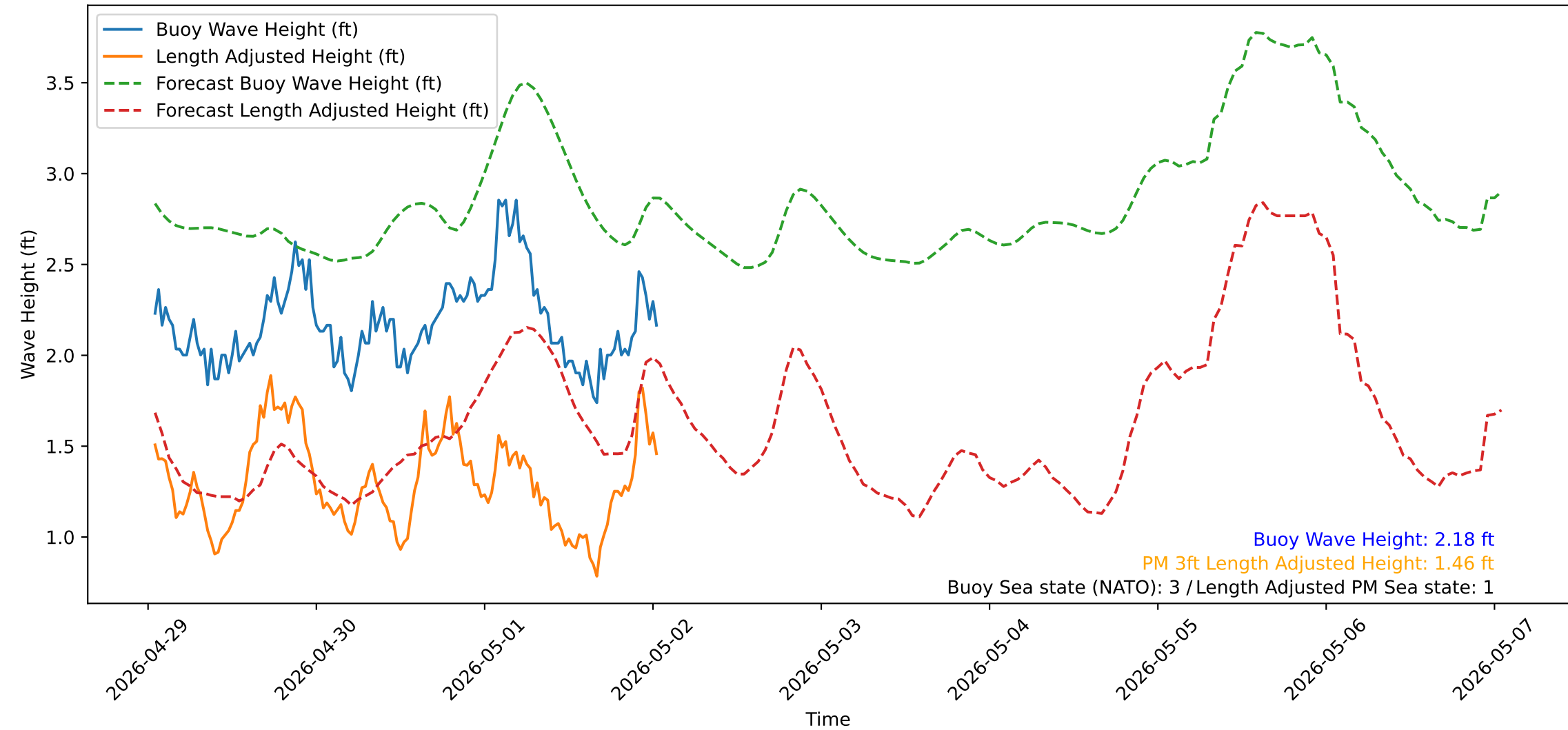
Wave Heights over Time for Green Beach at 2026-05-02 01:11:13
