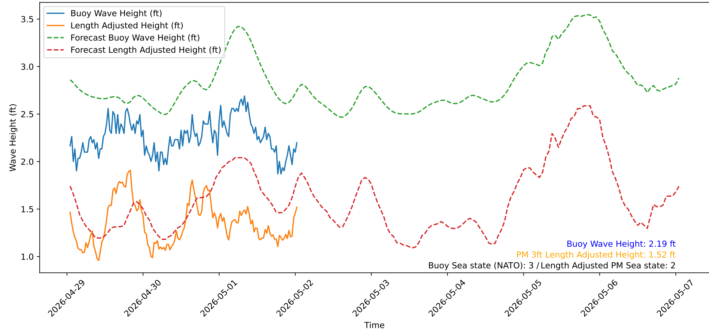
Wave Heights over Time for Oceanside Harbor at 2026-05-02 01:10:32
