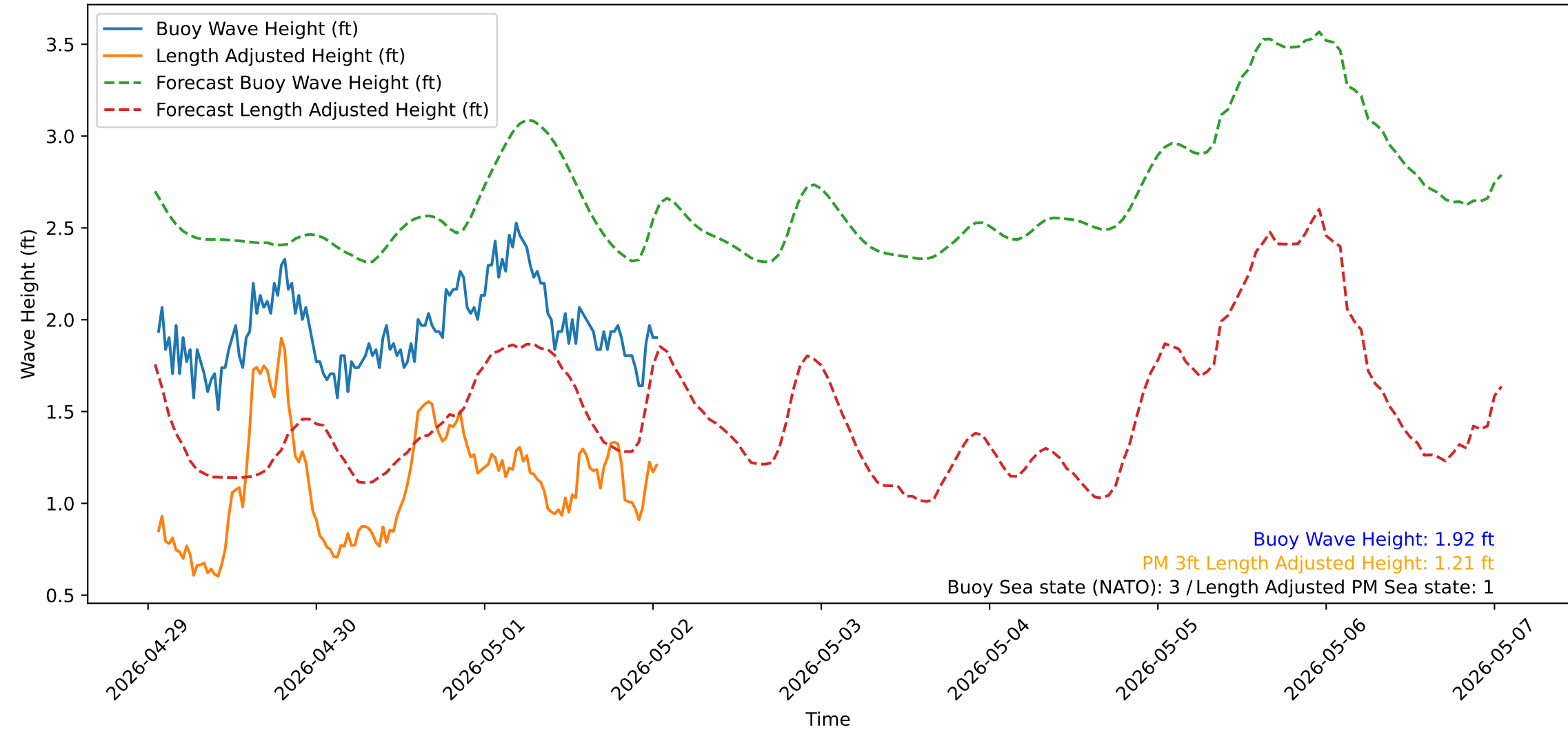
Wave Heights over Time for Red Beach at 2026-05-02 01:10:51
