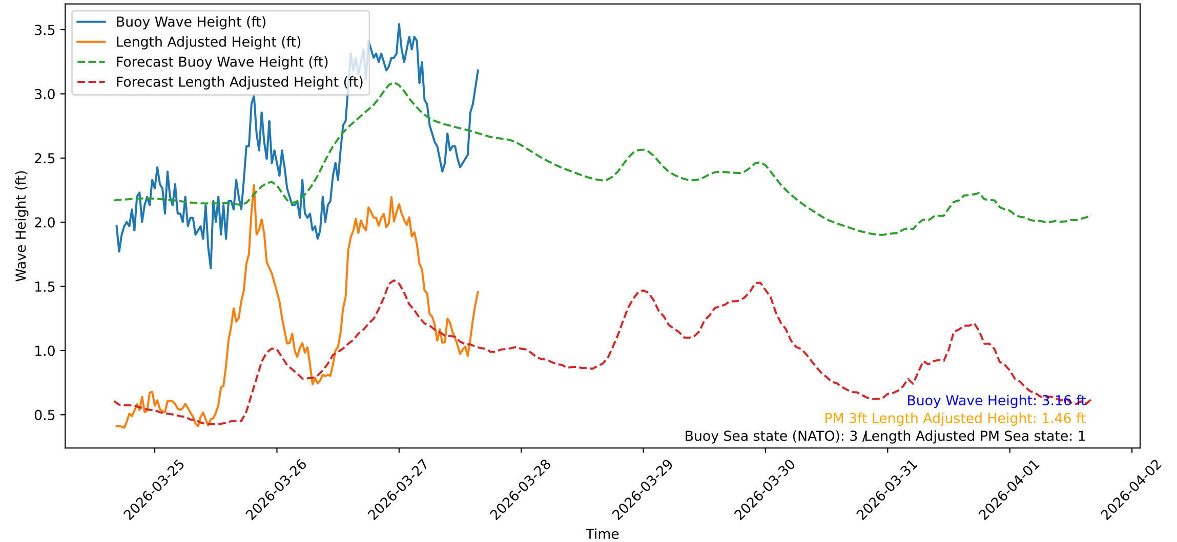
Wave Heights over Time for Green Beach at 2026-03-27 16:21:09
