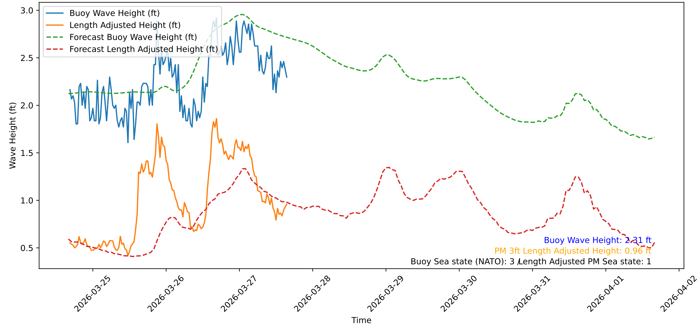
Wave Heights over Time for Oceanside Harbor at 2026-03-27 16:20:31
