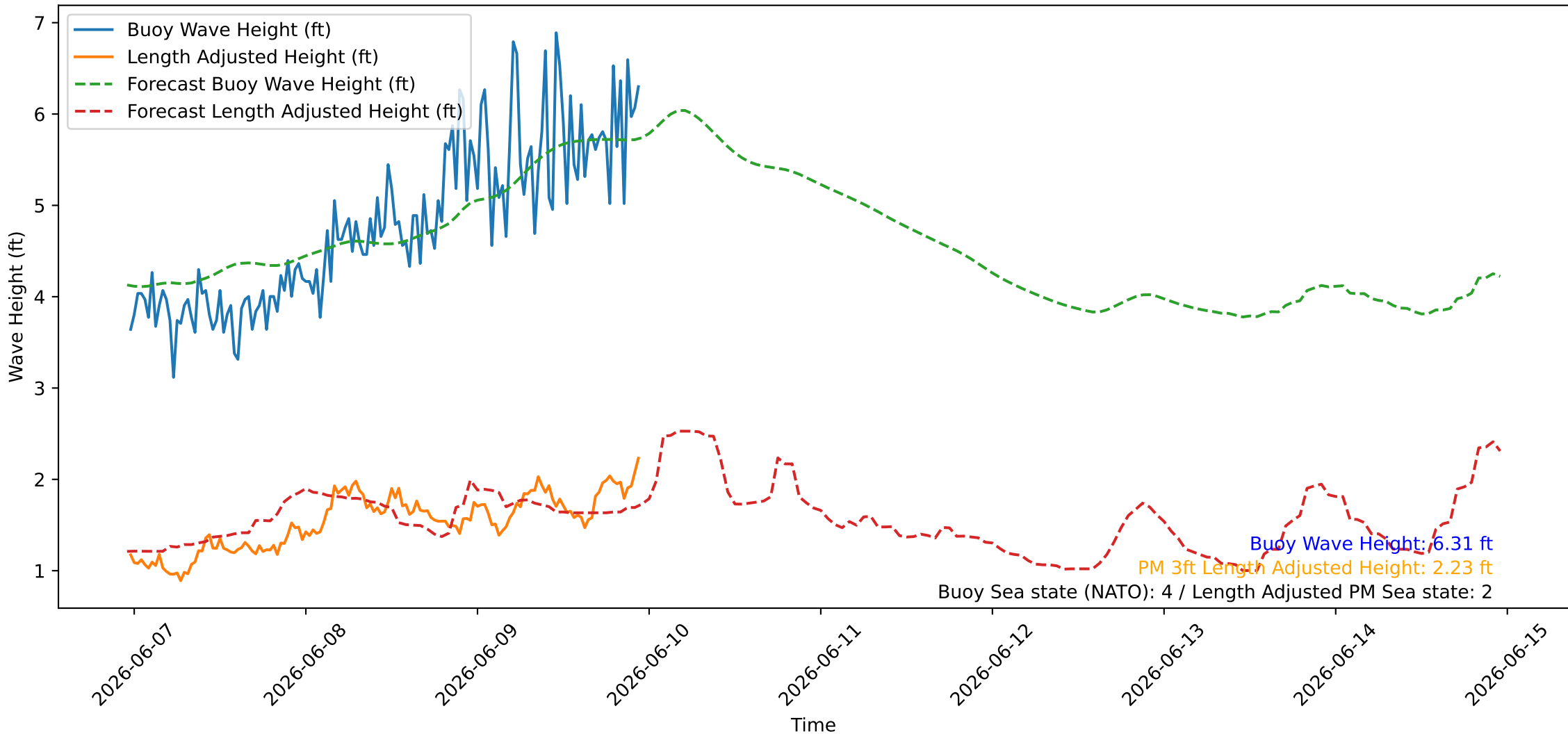
Wave Heights over Time for Green Beach at 2026-06-09 23:21:11
