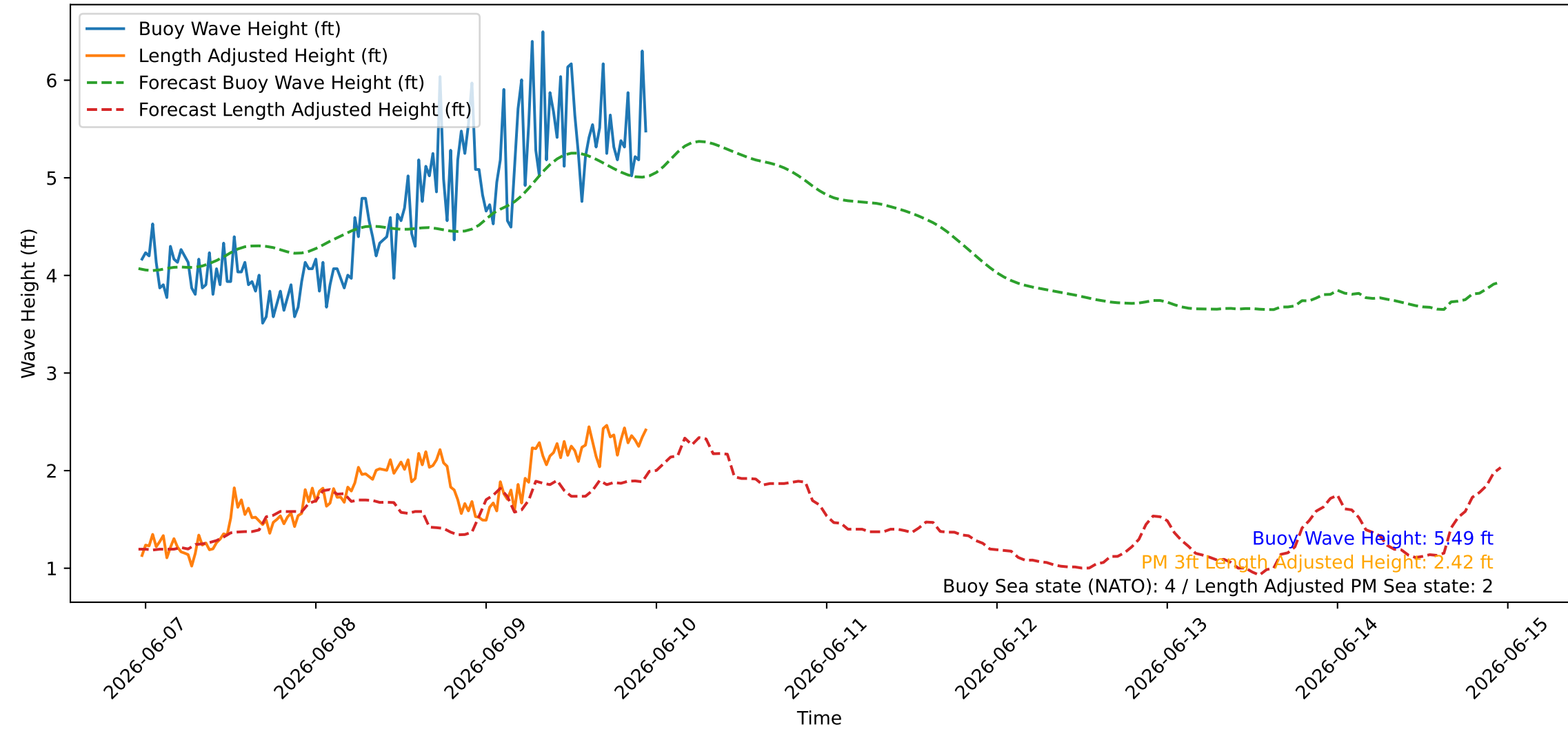
Wave Heights over Time for Oceanside Harbor at 2026-06-09 23:20:27
