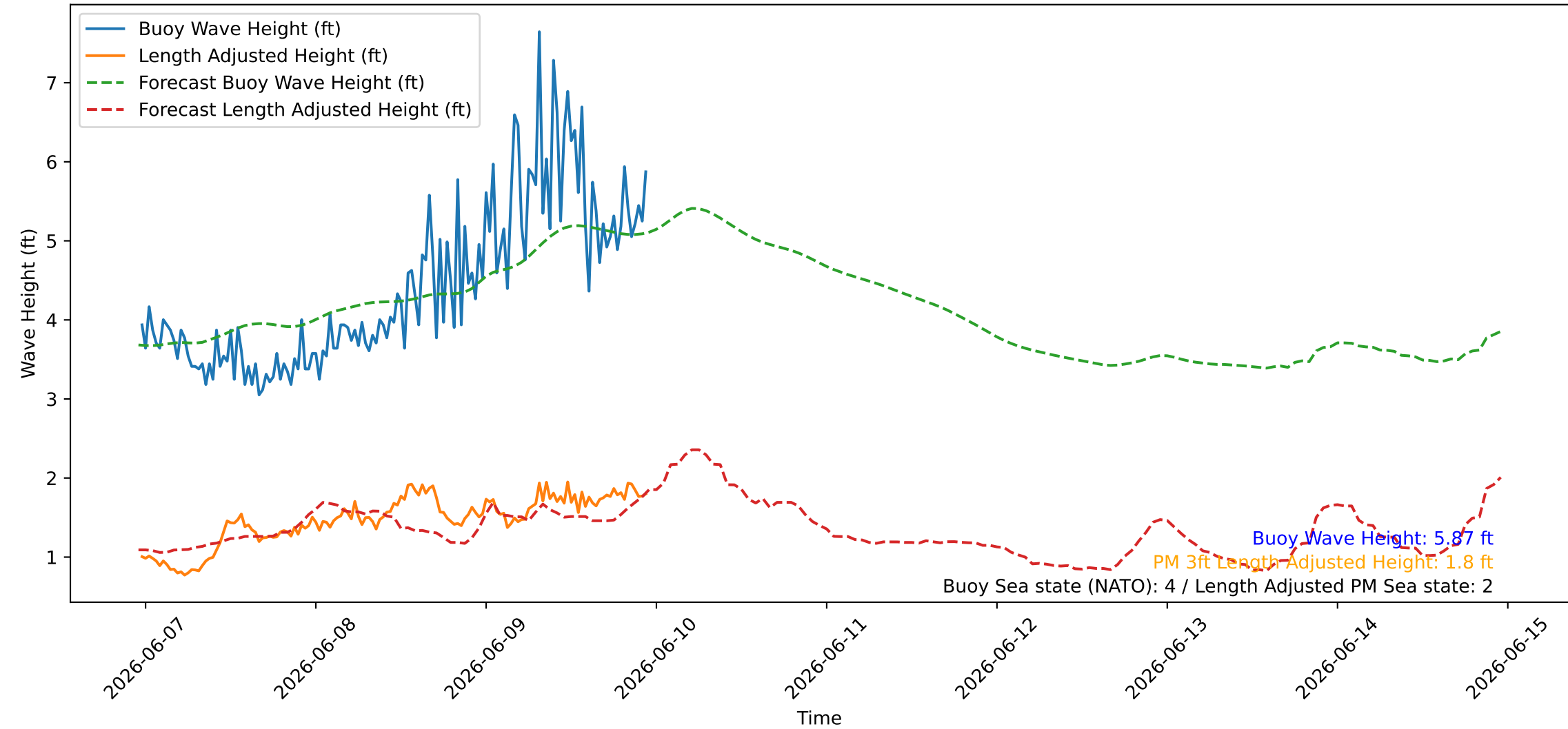
Wave Heights over Time for Red Beach at 2026-06-09 23:20:48
