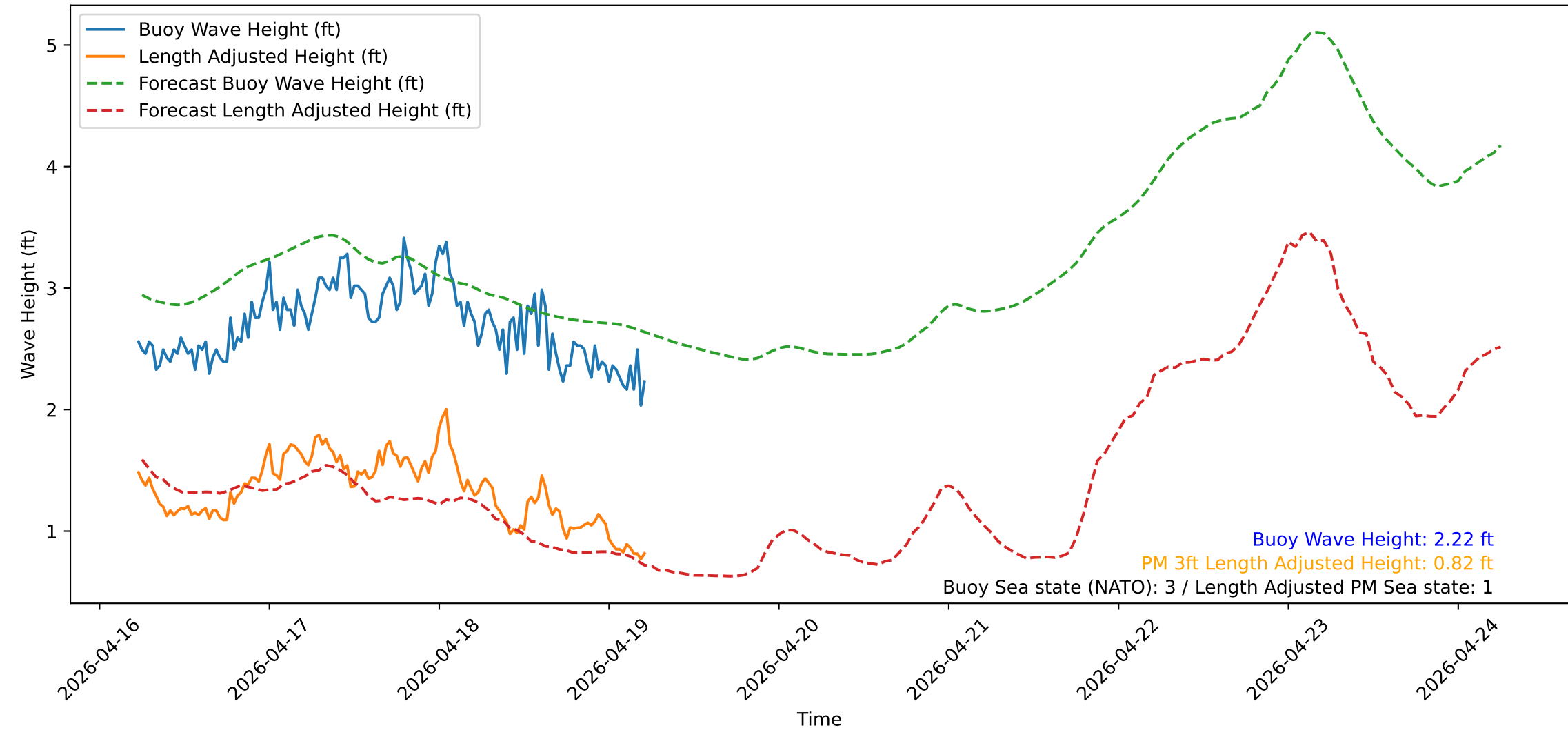
Wave Heights over Time for Oceanside Harbor at 2026-04-19 05:40:31
