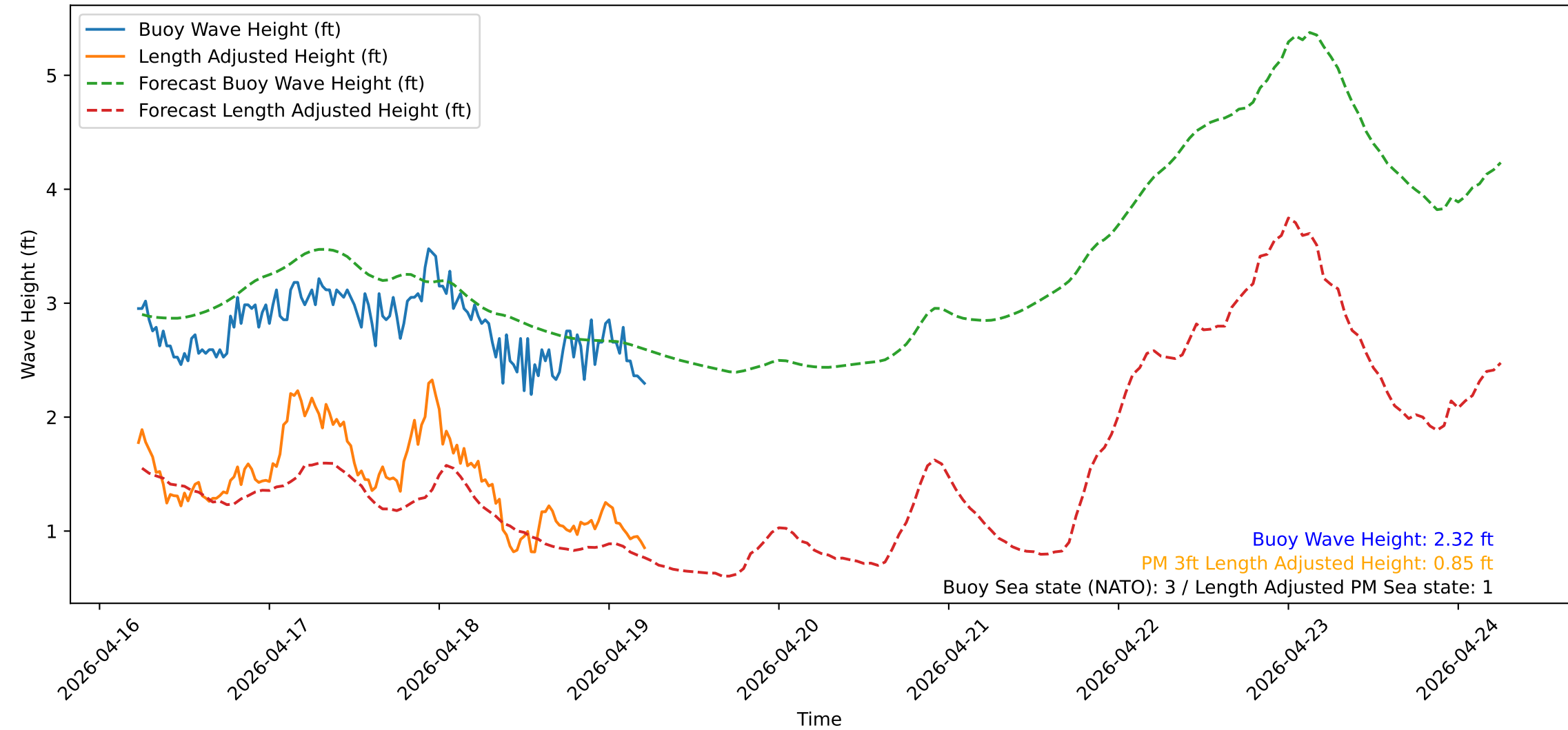
Wave Heights over Time for Green Beach at 2026-04-19 05:41:13
