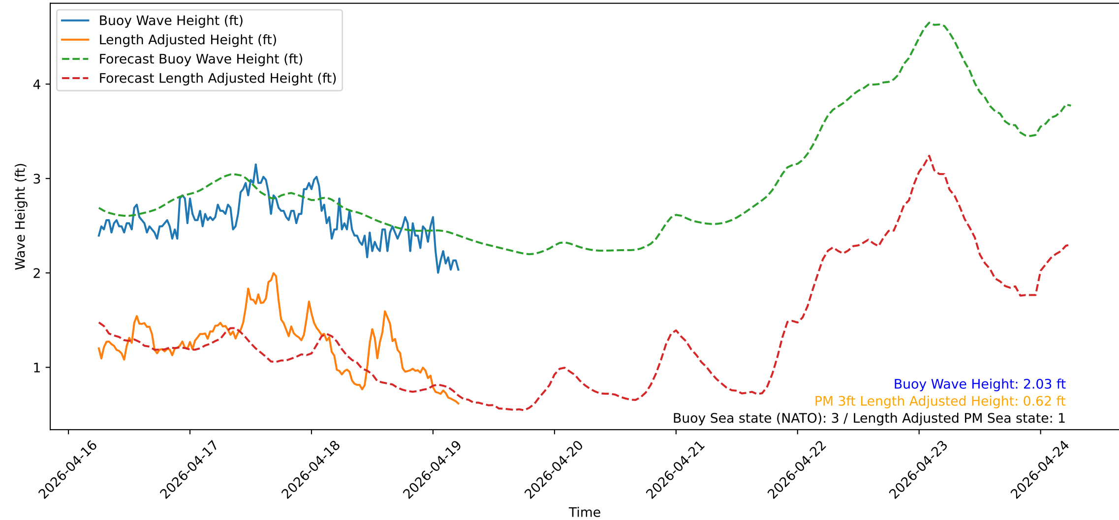
Wave Heights over Time for Red Beach at 2026-04-19 05:40:51
