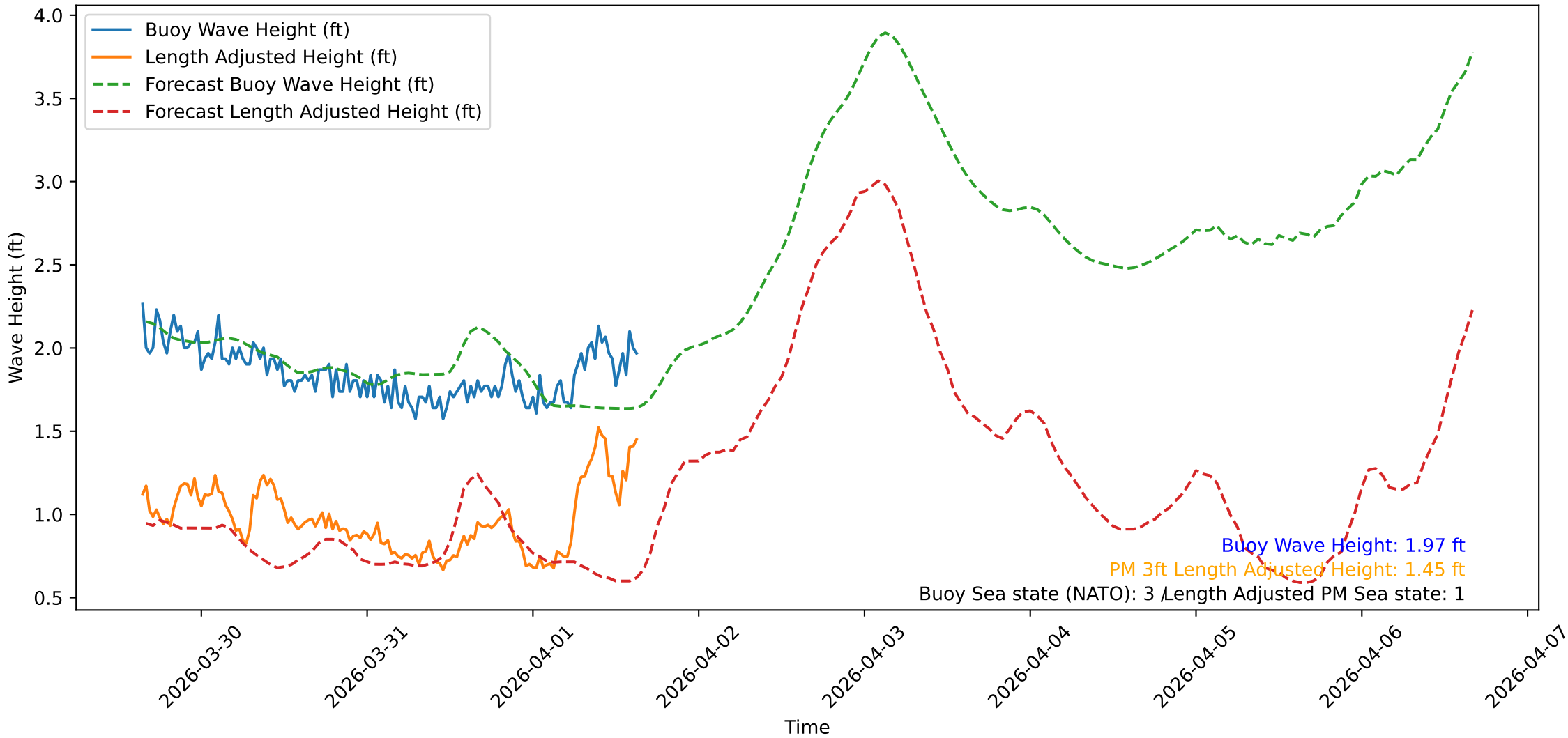
Wave Heights over Time for Oceanside Harbor at 2026-04-01 15:30:32
