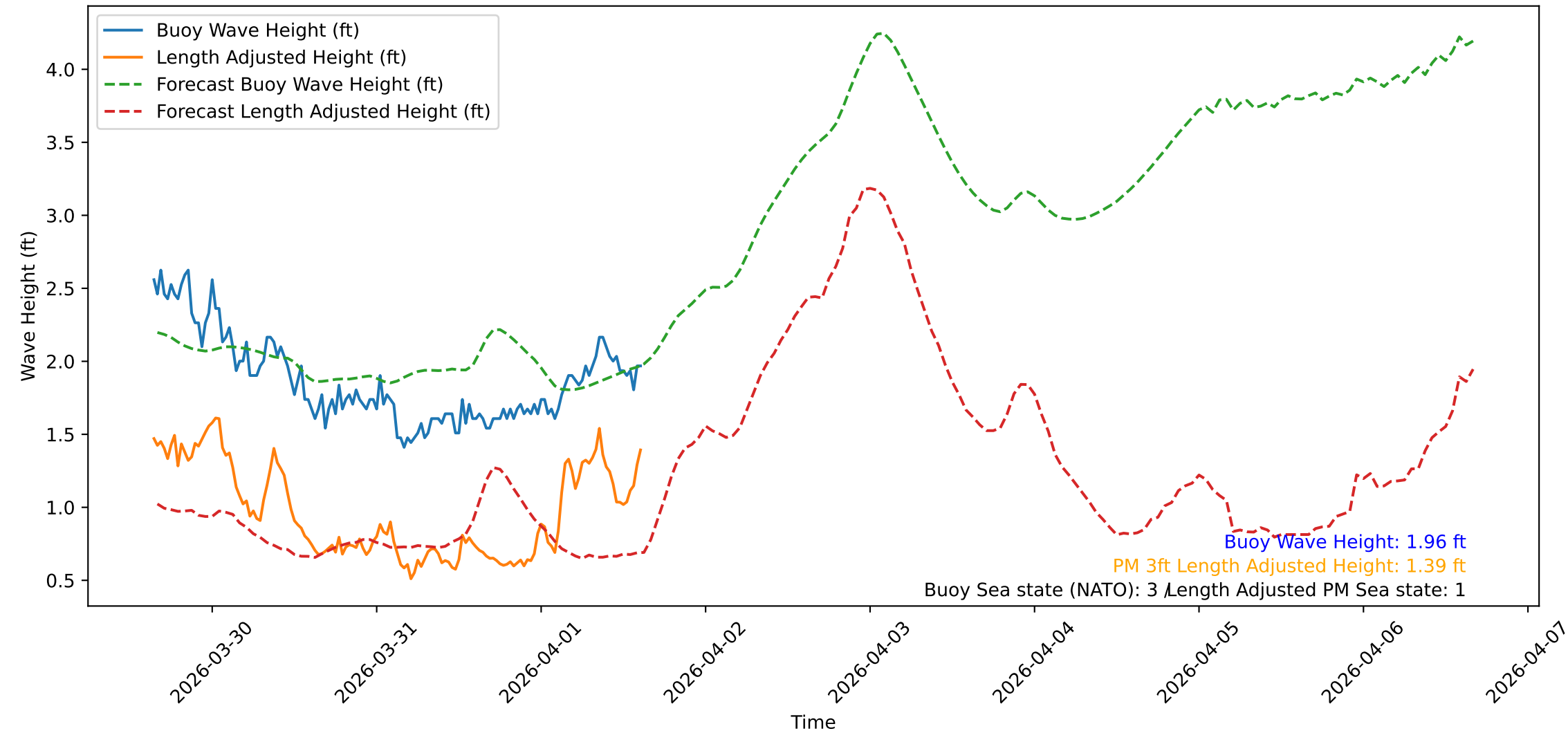
Wave Heights over Time for Green Beach at 2026-04-01 15:31:10
