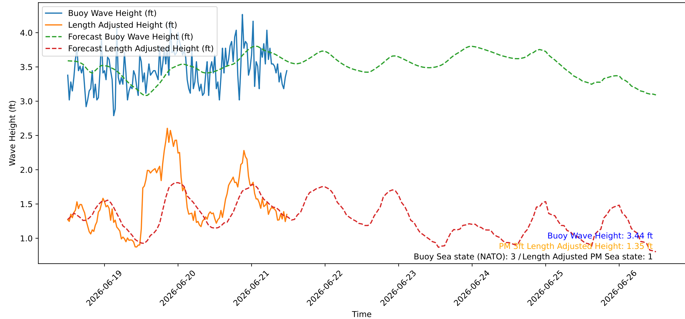
Wave Heights over Time for Oceanside Harbor at 2026-06-21 12:10:26
