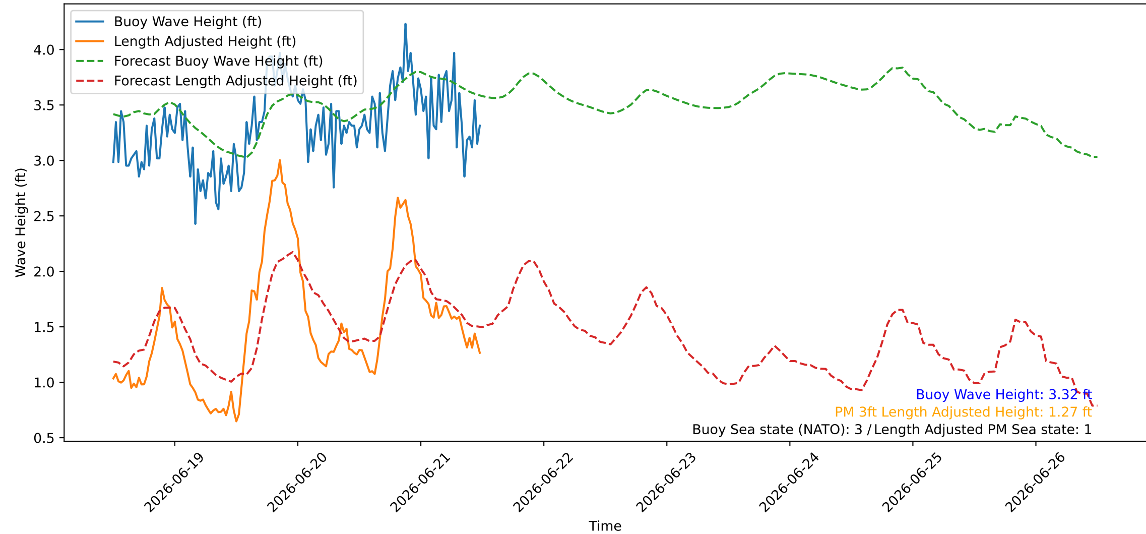
Wave Heights over Time for Green Beach at 2026-06-21 12:11:07
