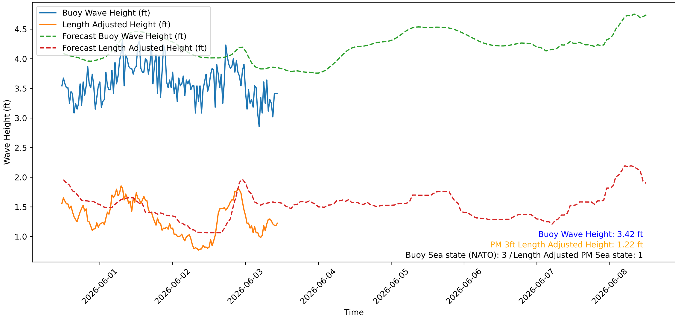
Wave Heights over Time for Green Beach at 2026-06-03 11:31:07
