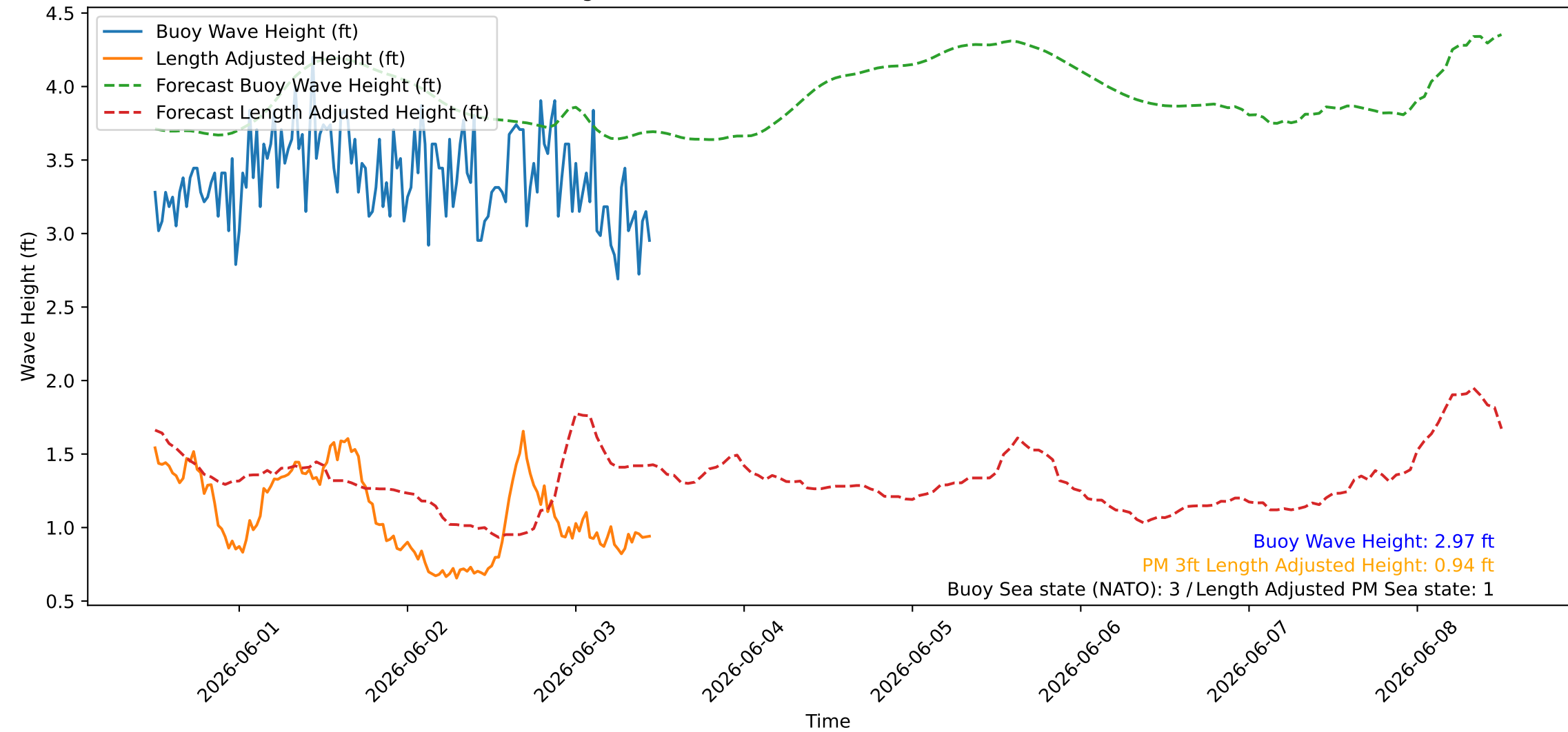
Wave Heights over Time for Red Beach at 2026-06-03 11:30:45
