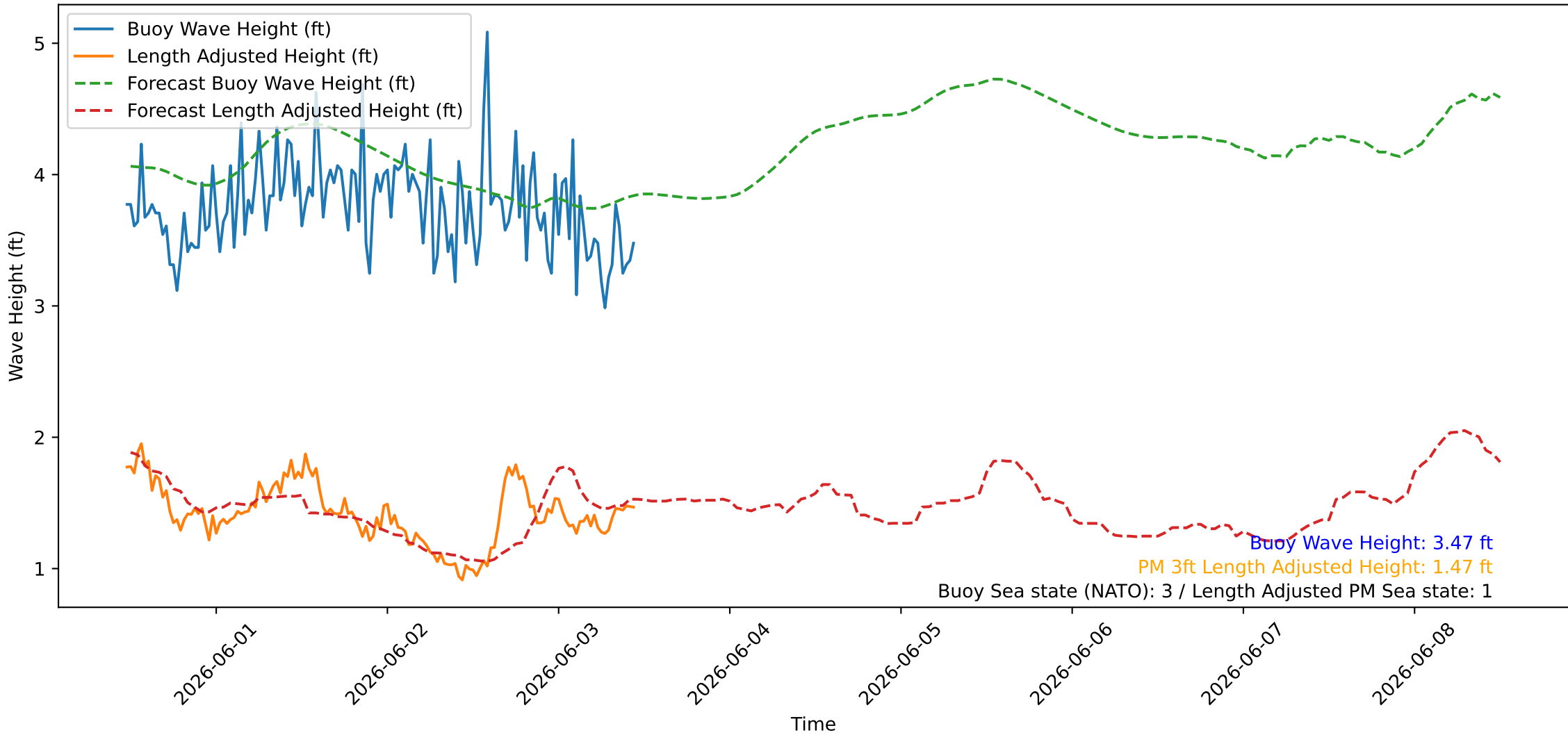
Wave Heights over Time for Oceanside Harbor at 2026-06-03 11:30:26
