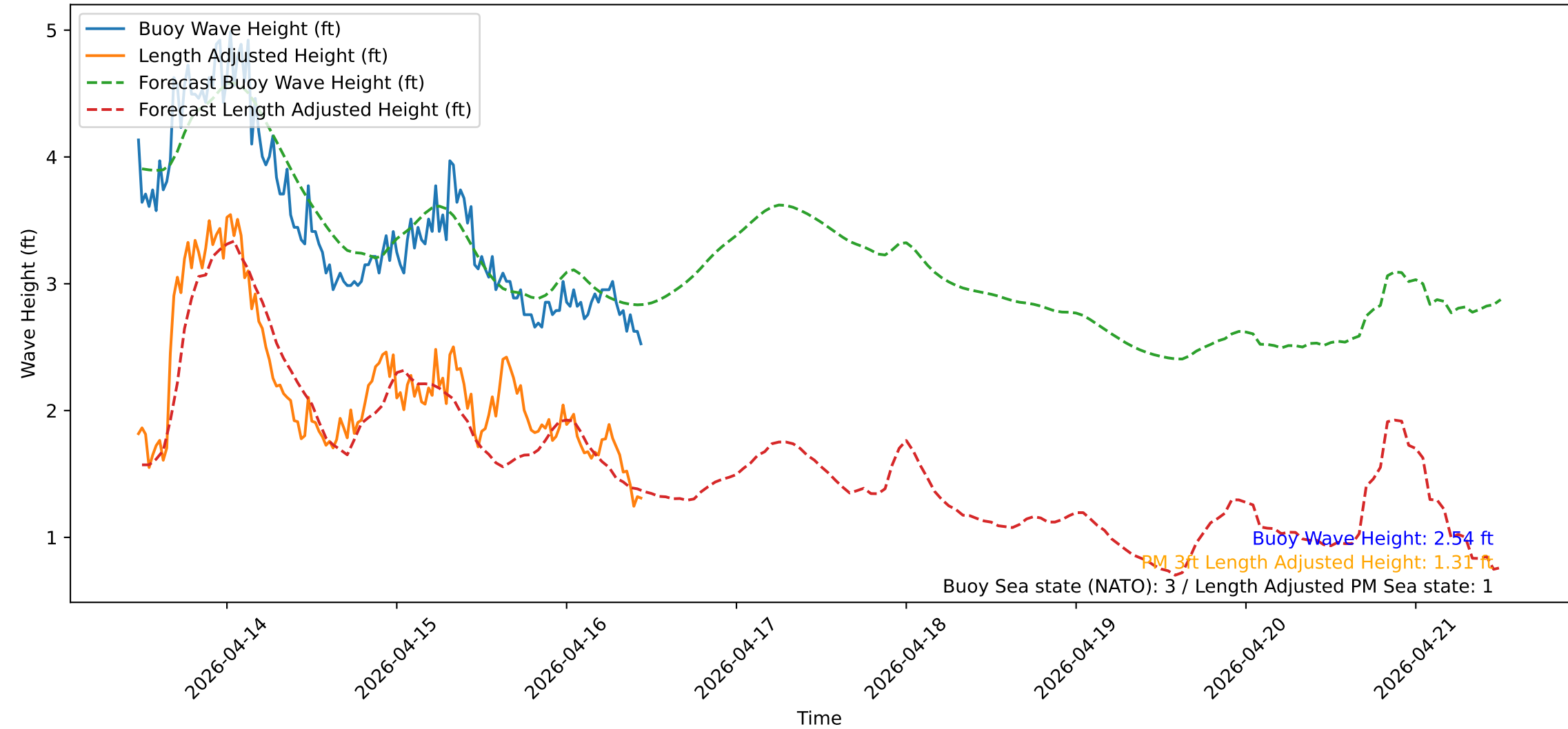
Wave Heights over Time for Green Beach at 2026-04-16 11:31:13
