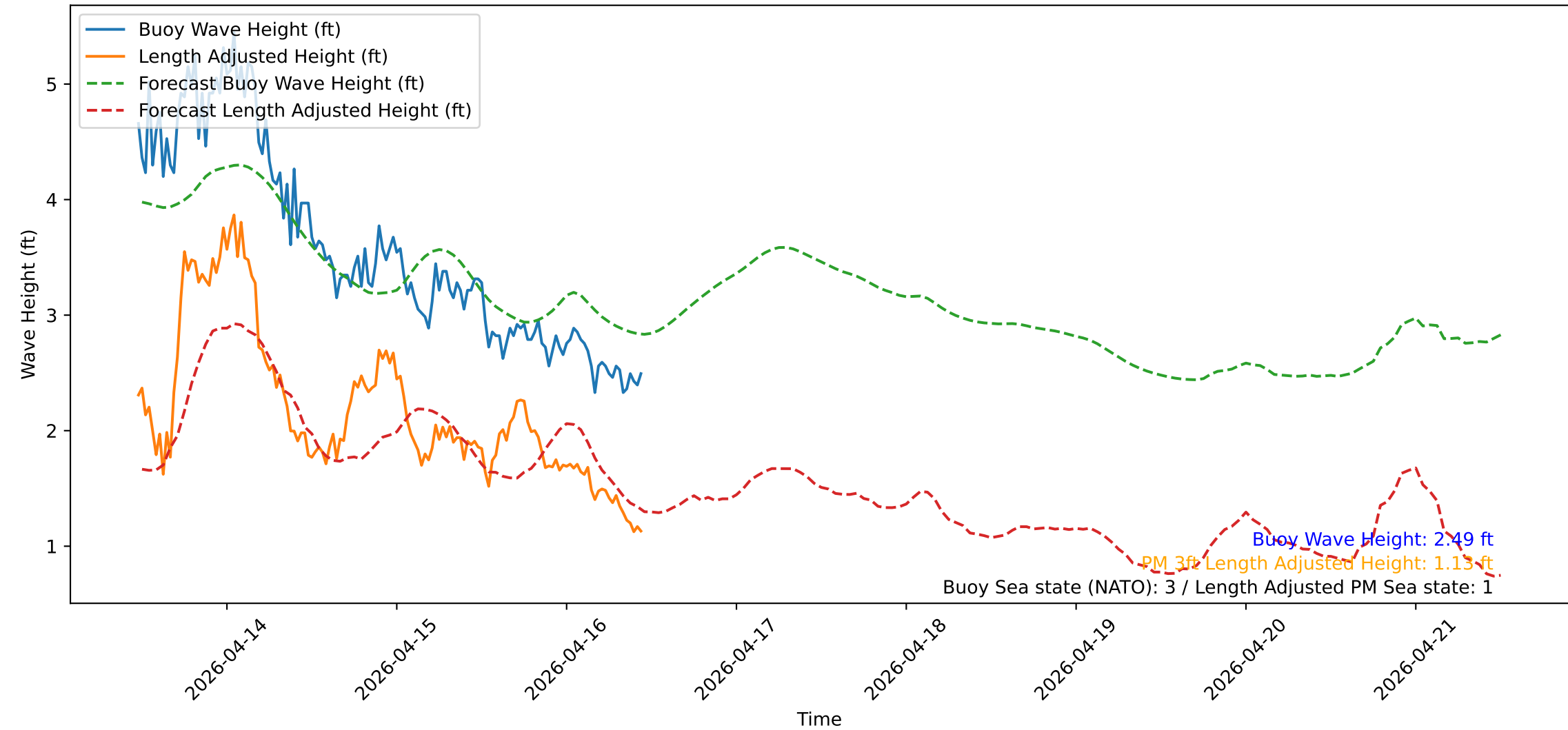
Wave Heights over Time for Oceanside Harbor at 2026-04-16 11:30:31
