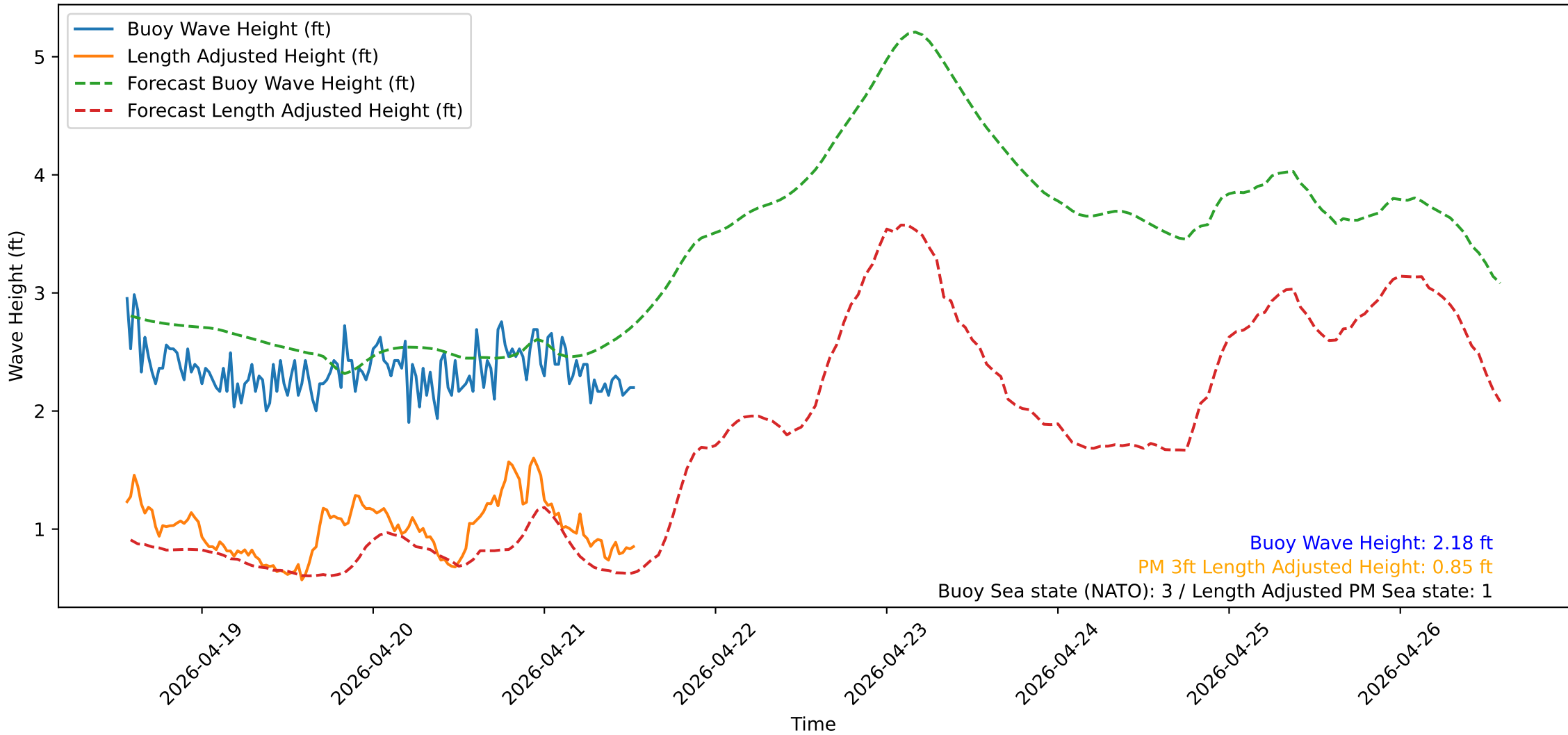
Wave Heights over Time for Oceanside Harbor at 2026-04-21 13:30:32
