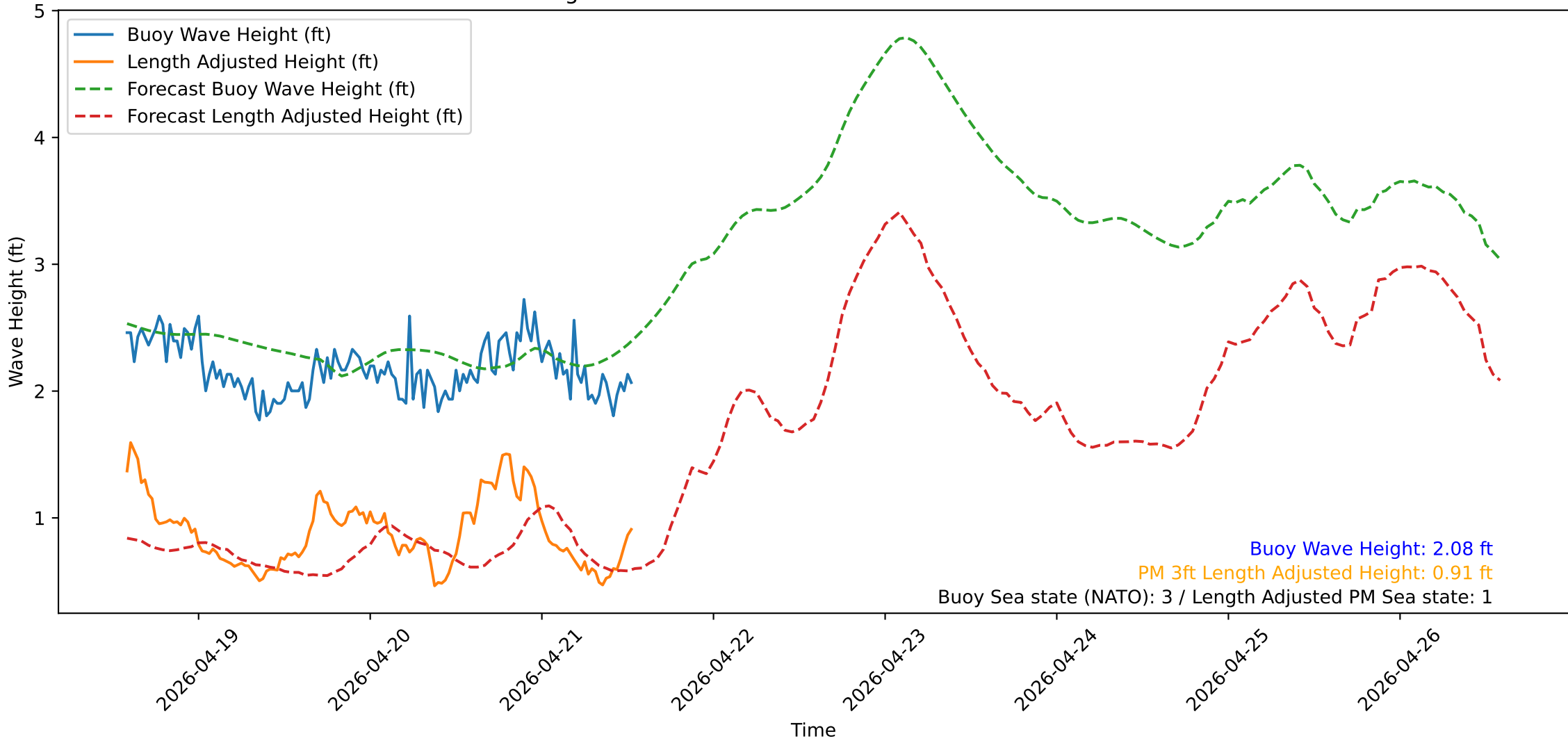
Wave Heights over Time for Red Beach at 2026-04-21 13:30:51
