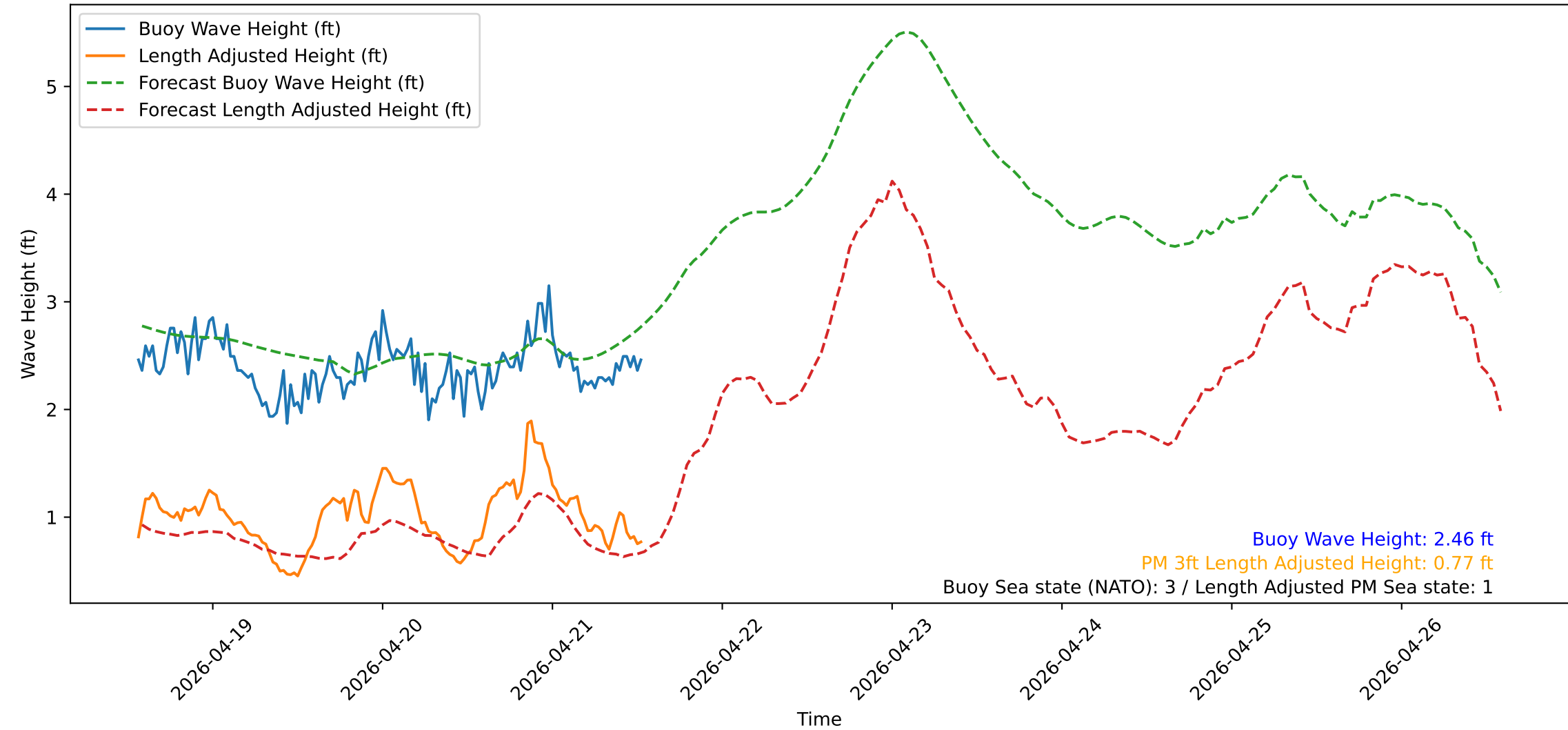
Wave Heights over Time for Green Beach at 2026-04-21 13:31:13
