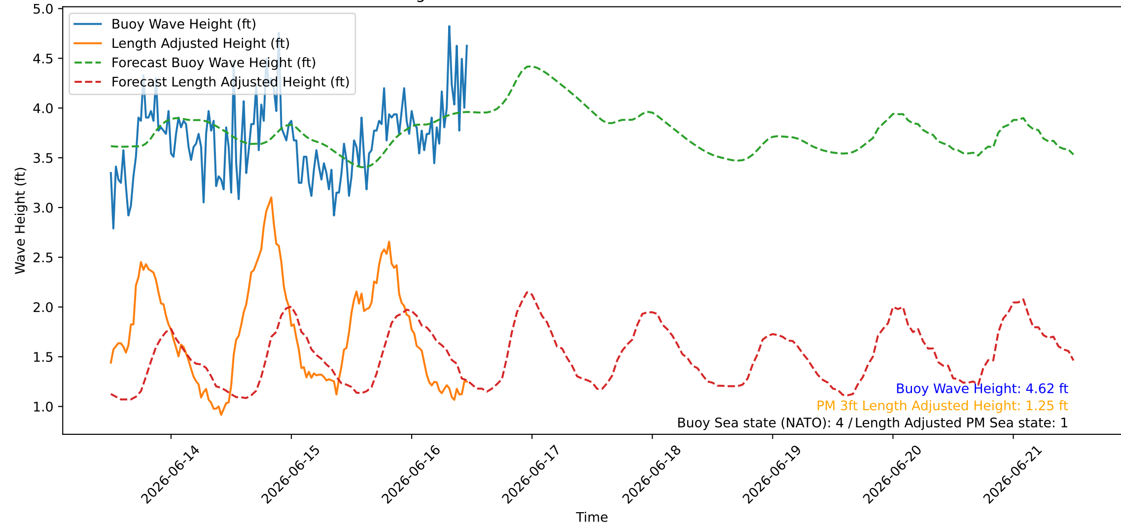
Wave Heights over Time for Red Beach at 2026-06-16 11:40:46
