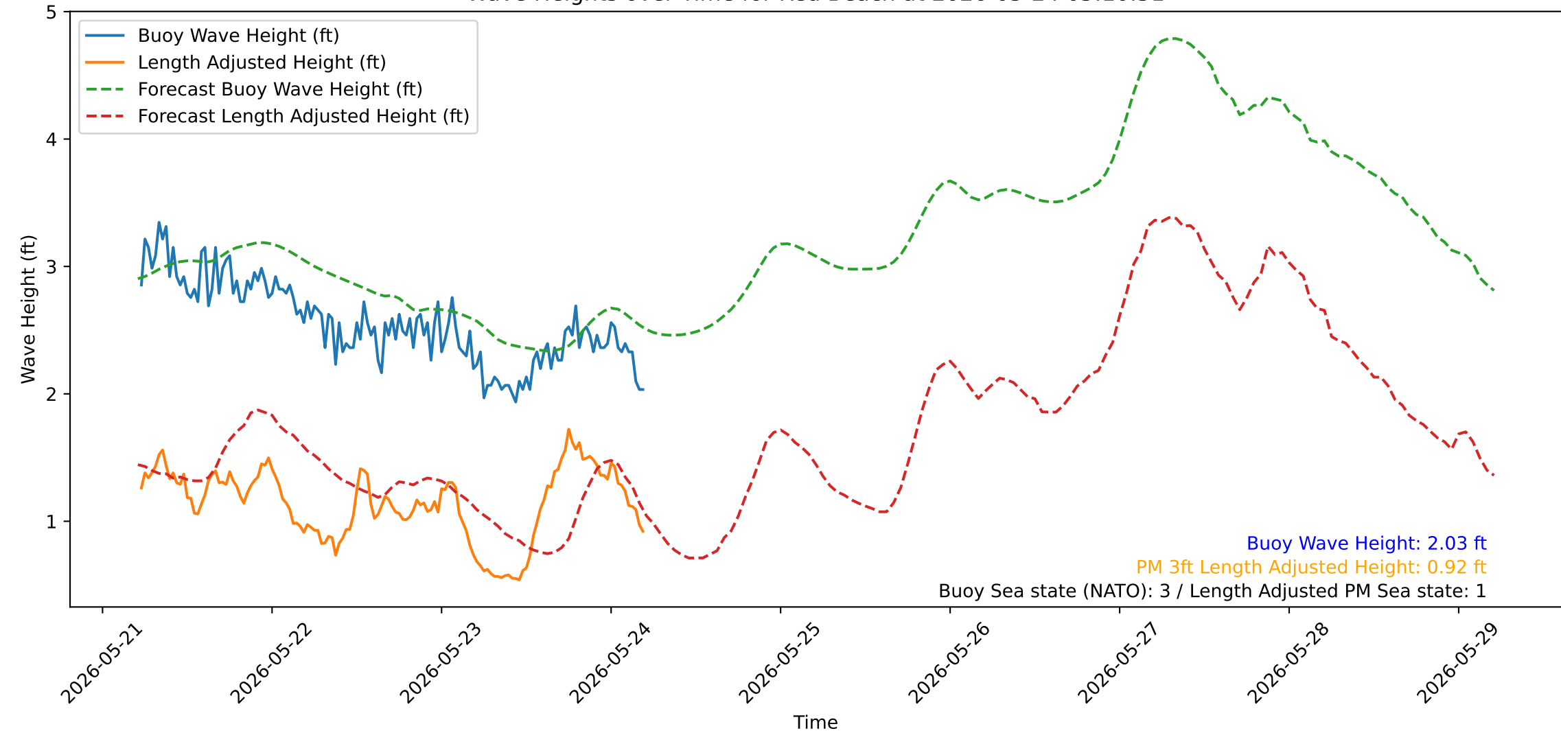
Wave Heights over Time for Red Beach at 2026-05-24 05:10:51
