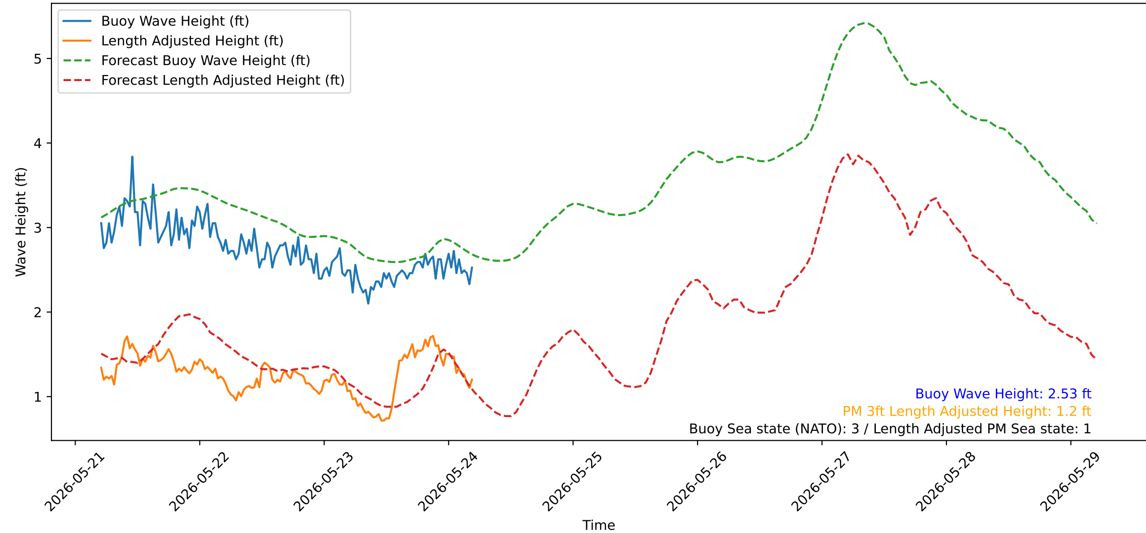
Wave Heights over Time for Oceanside Harbor at 2026-05-24 05:10:31
