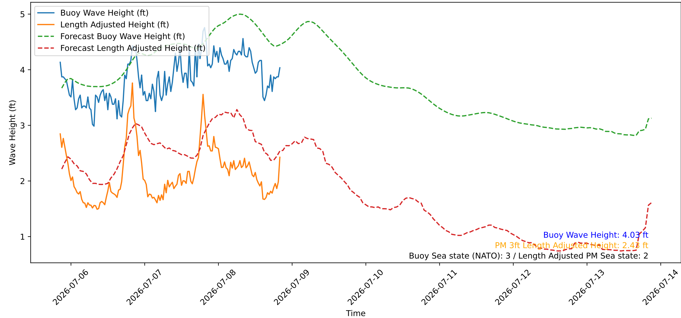
Wave Heights over Time for Green Beach at 2026-07-08 20:41:08
