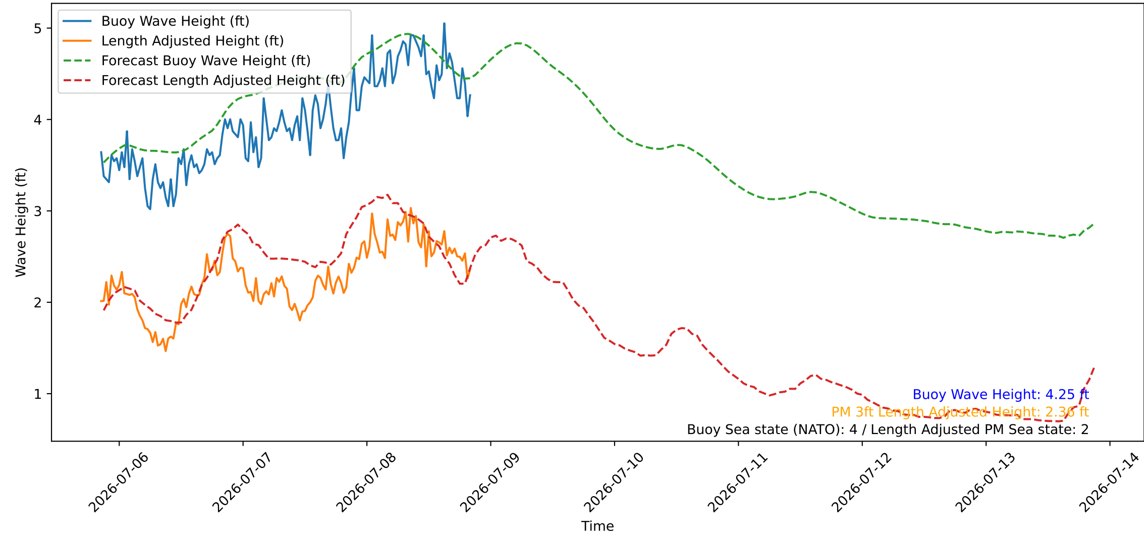
Wave Heights over Time for Oceanside Harbor at 2026-07-08 20:40:26
