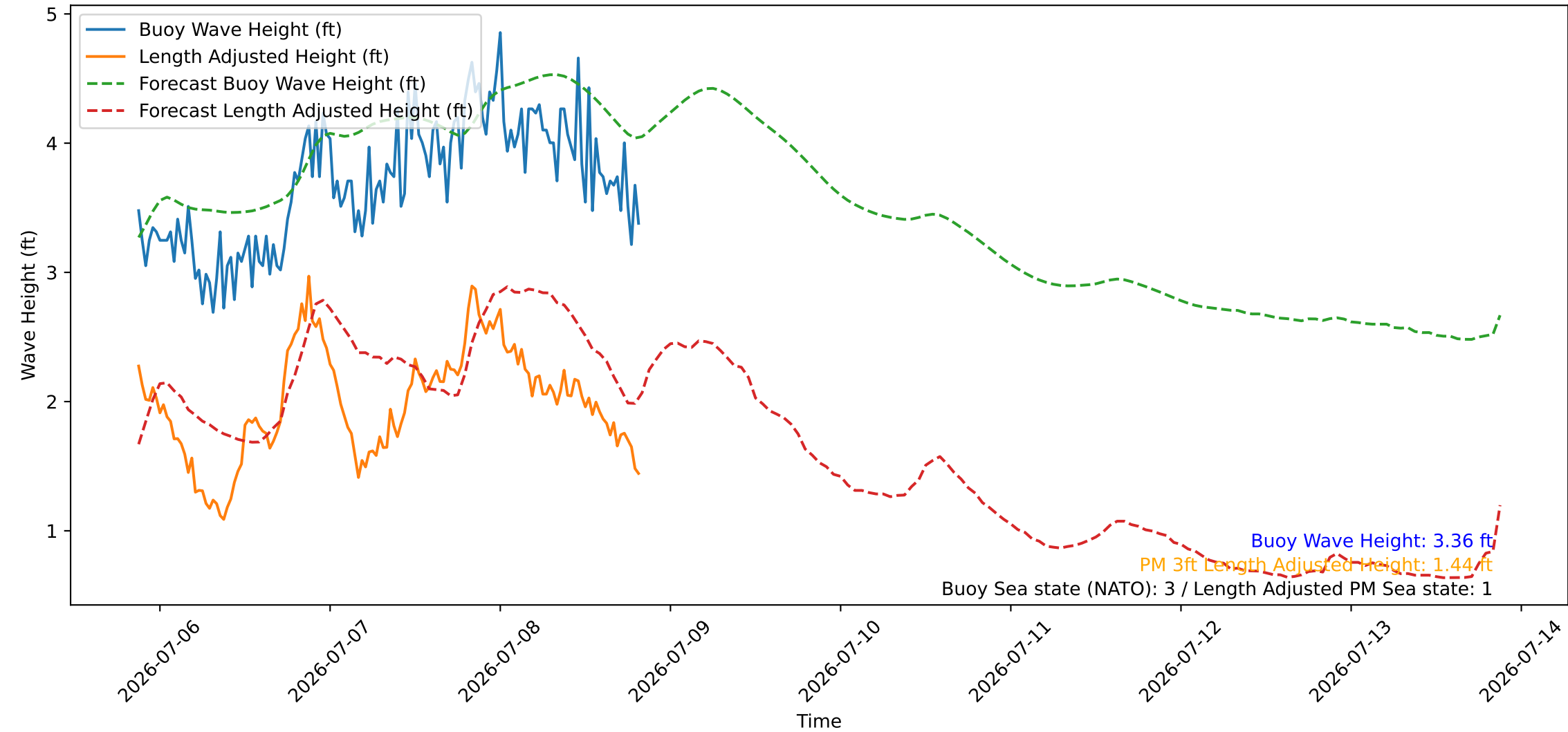
Wave Heights over Time for Red Beach at 2026-07-08 20:40:45
