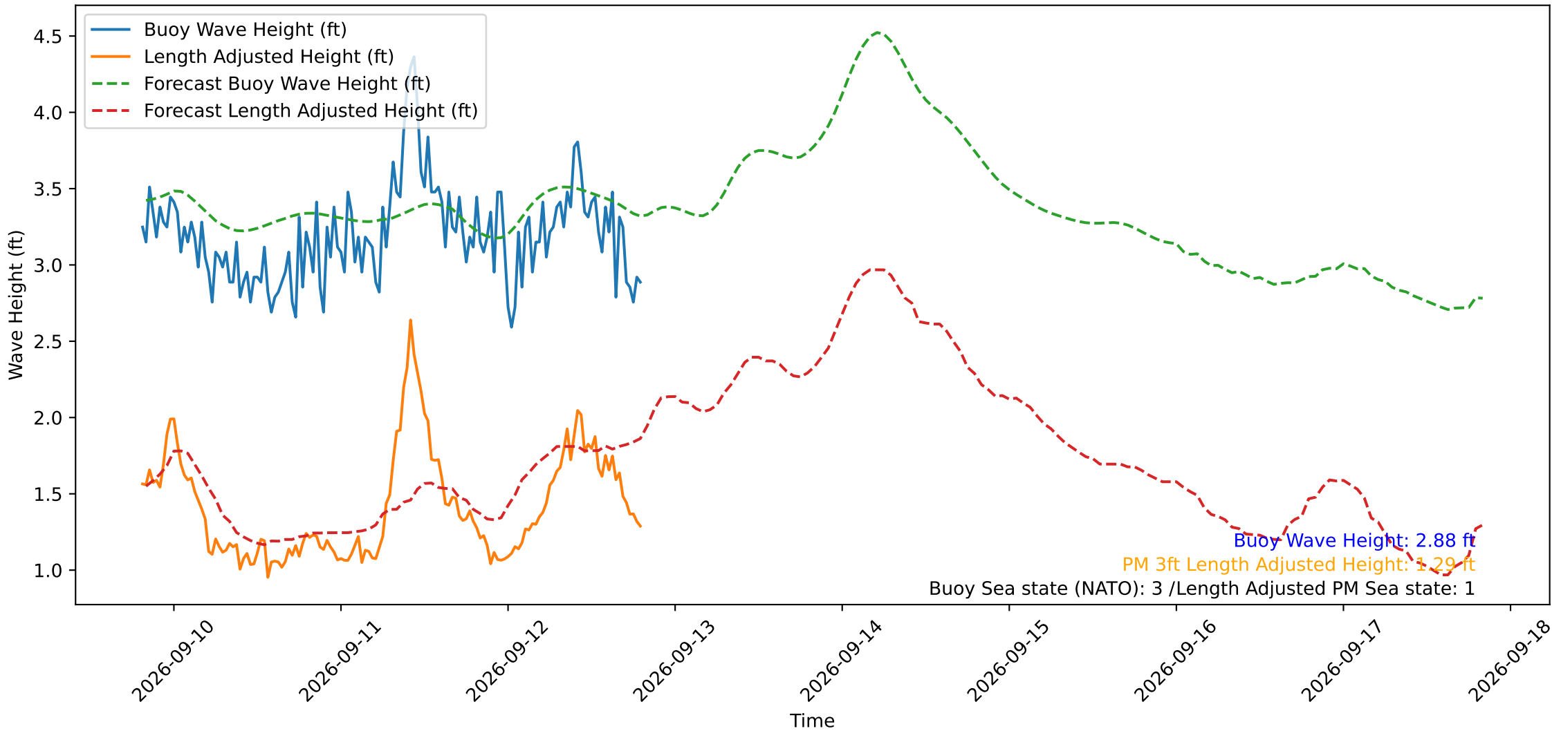
Wave Heights over Time for Oceanside Harbor at 2026-09-12 19:40:30
