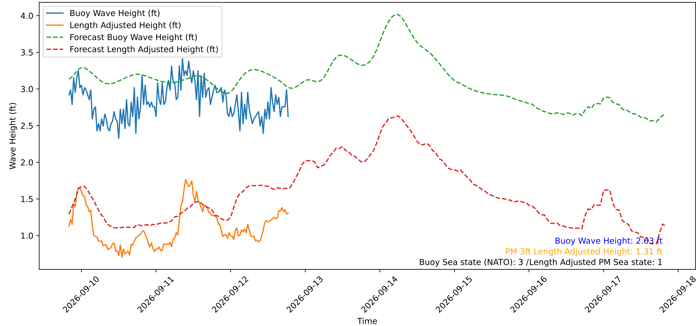
Wave Heights over Time for Red Beach at 2026-09-12 19:40:50
