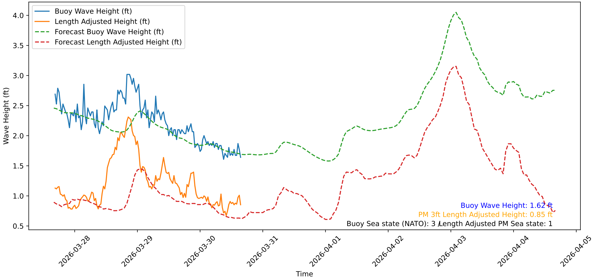
Wave Heights over Time for Red Beach at 2026-03-30 16:20:47
