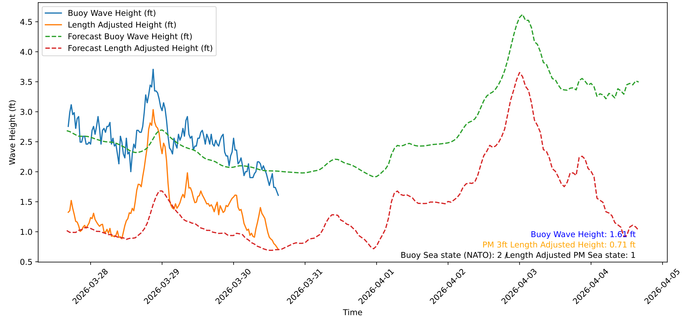
Wave Heights over Time for Green Beach at 2026-03-30 16:21:10
