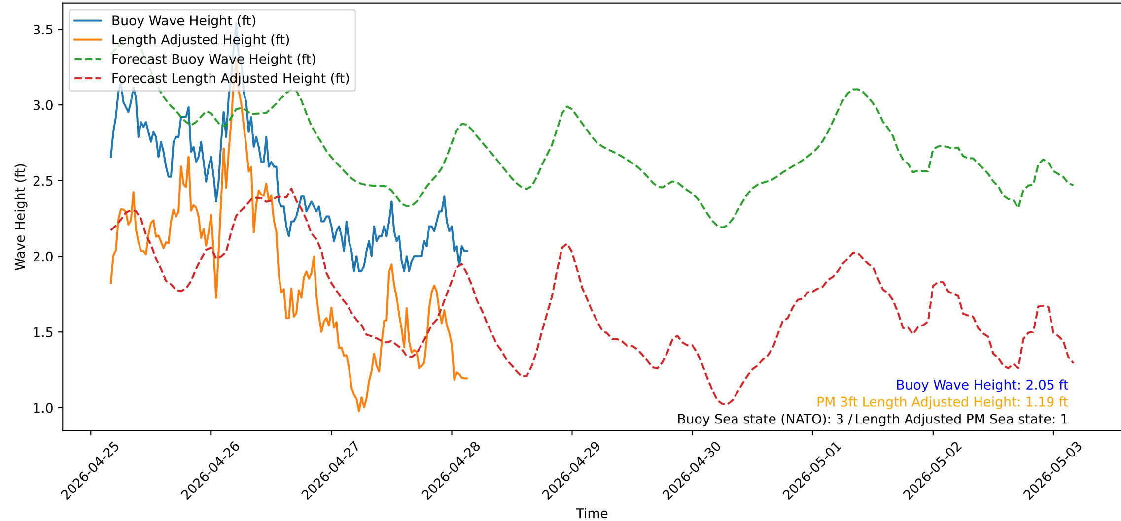
Wave Heights over Time for Red Beach at 2026-04-28 03:50:51
