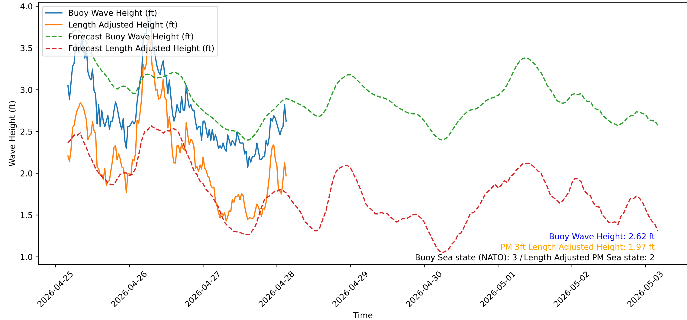
Wave Heights over Time for Oceanside Harbor at 2026-04-28 03:50:31
