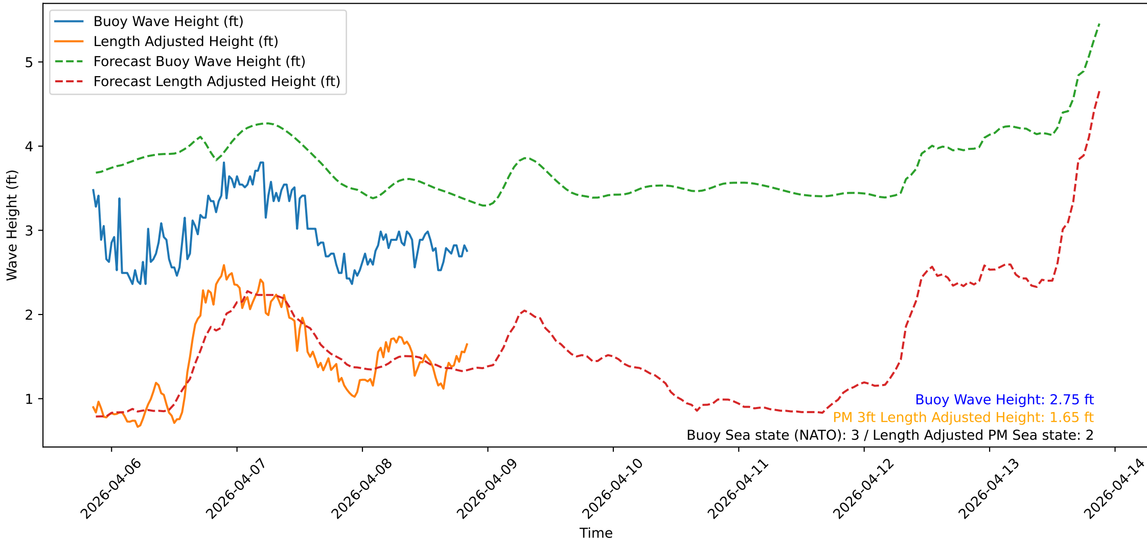
Wave Heights over Time for Green Beach at 2026-04-08 20:41:11
