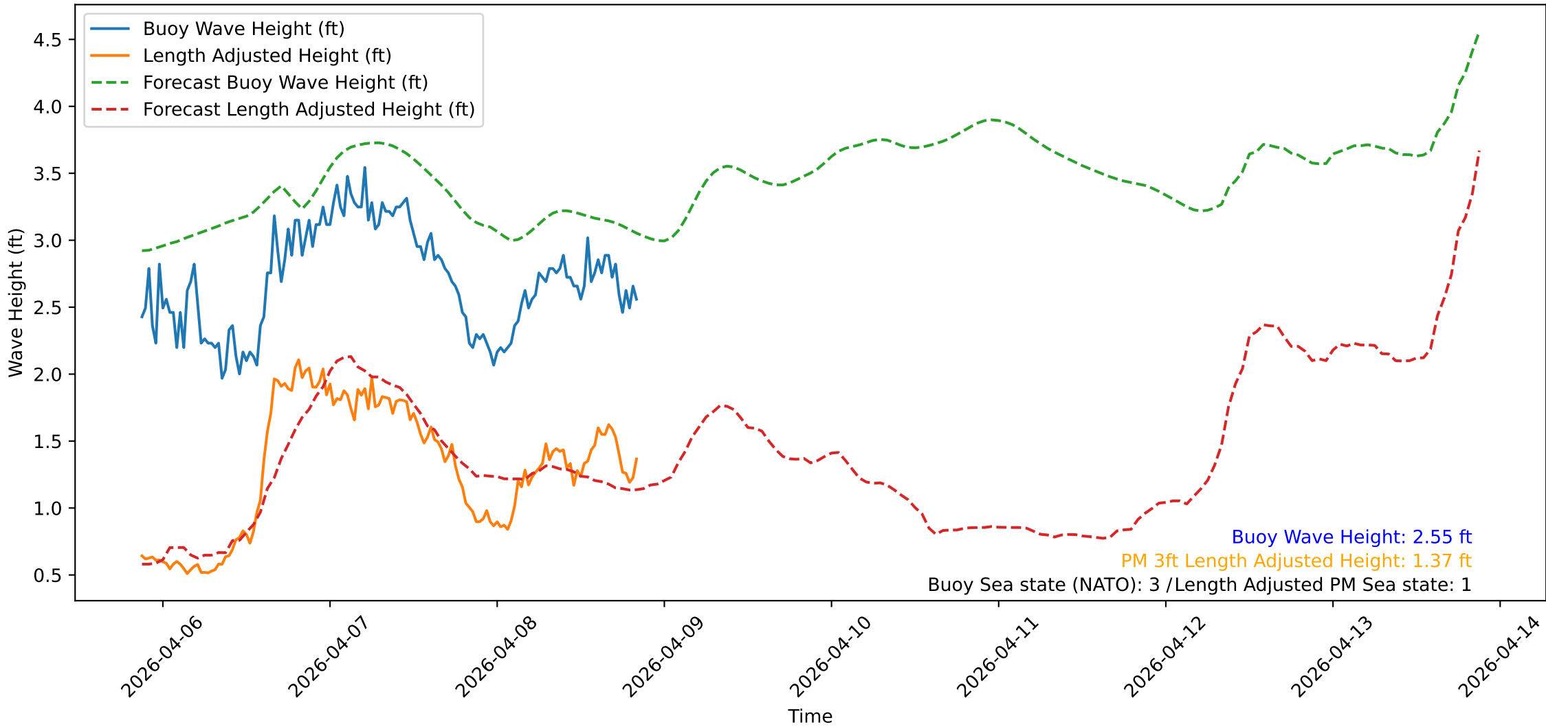
Wave Heights over Time for Red Beach at 2026-04-08 20:40:48
