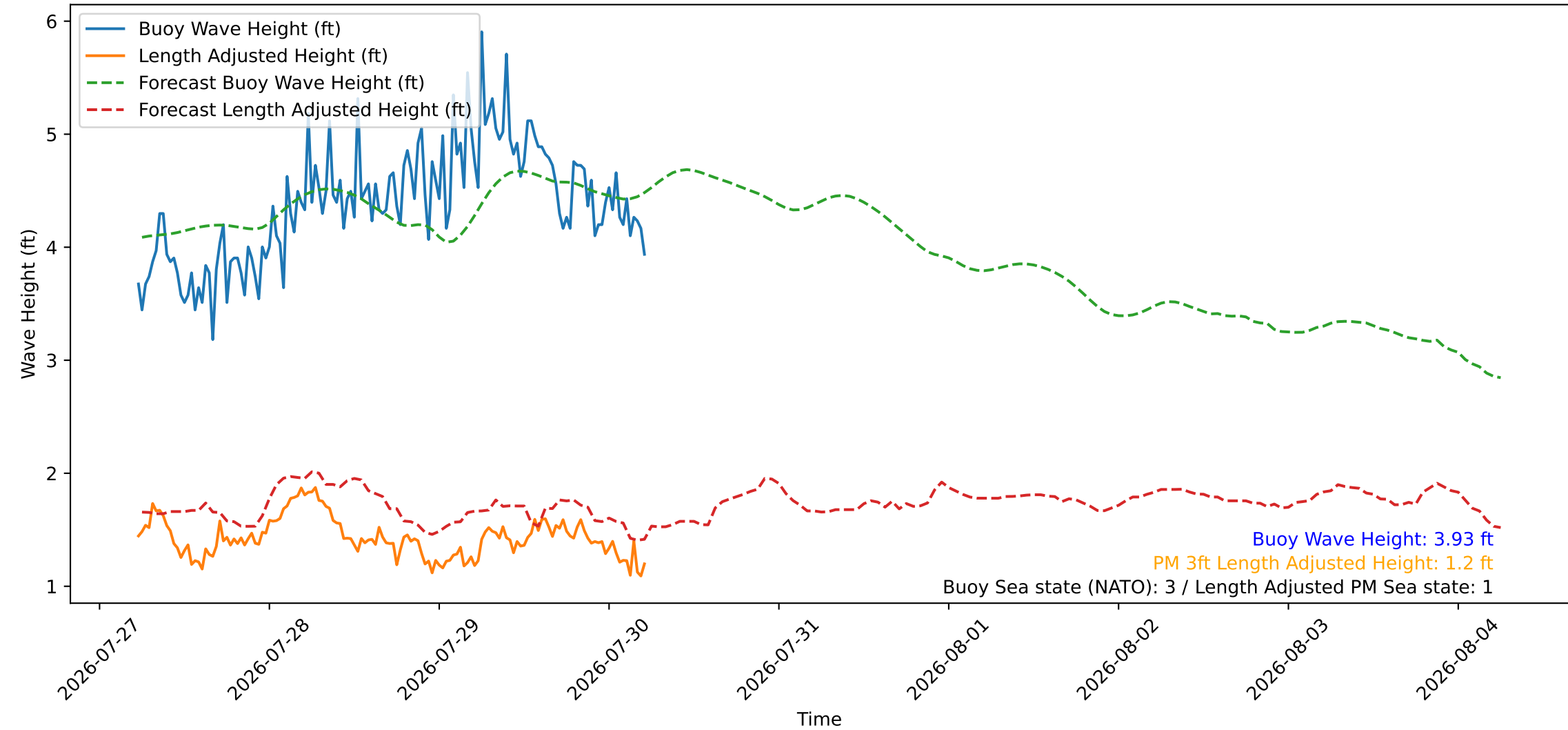
Wave Heights over Time for Oceanside Harbor at 2026-07-30 05:30:26
