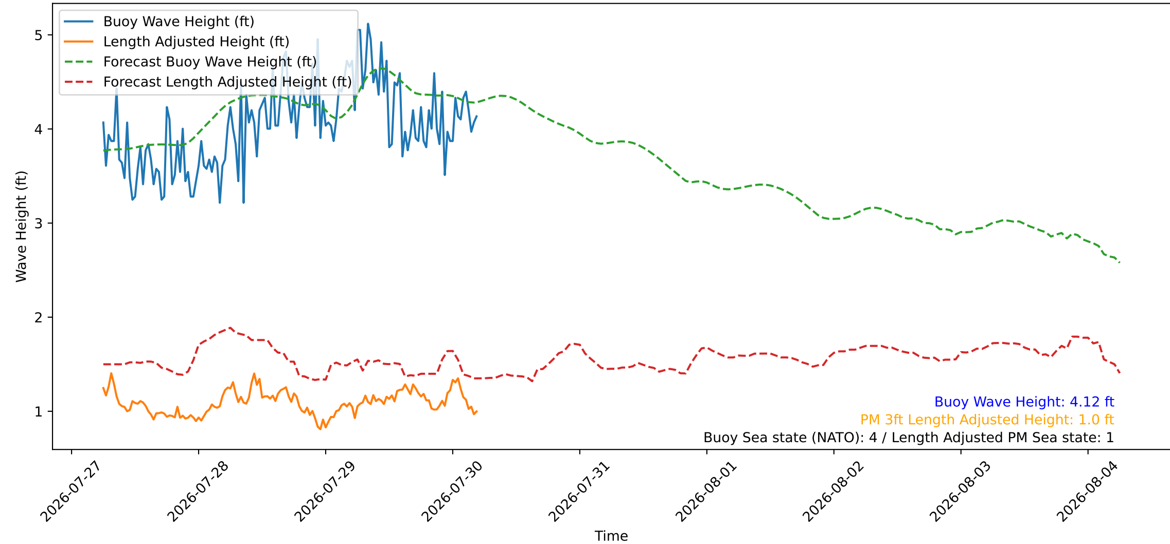
Wave Heights over Time for Red Beach at 2026-07-30 05:30:45
