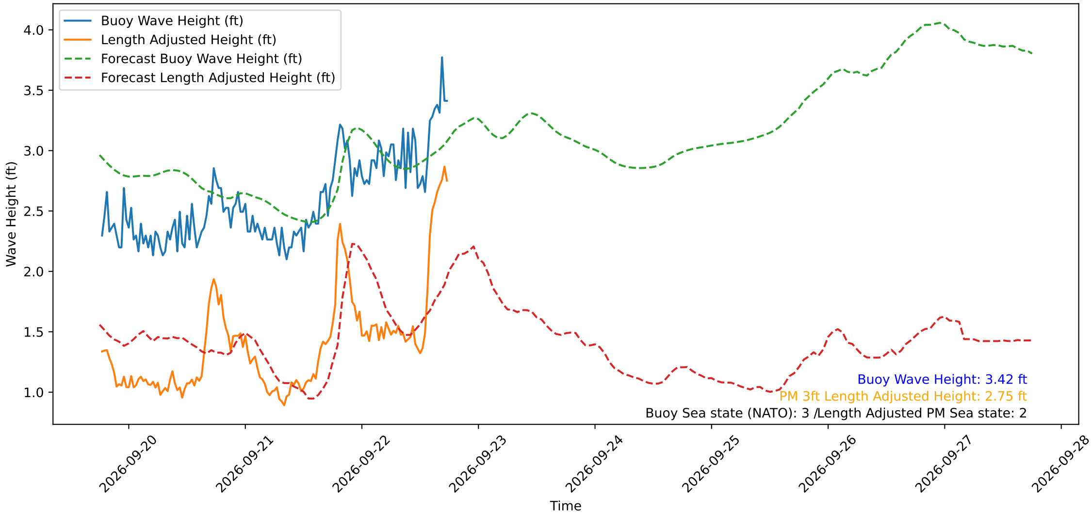
Wave Heights over Time for Oceanside Harbor at 2026-09-22 18:20:30
