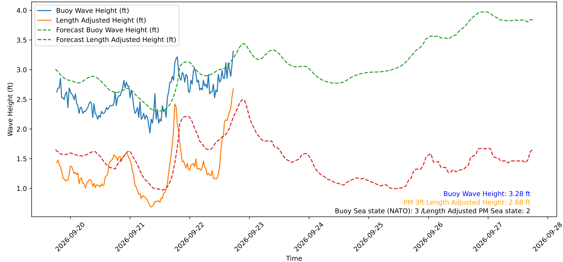
Wave Heights over Time for Green Beach at 2026-09-22 18:21:15
