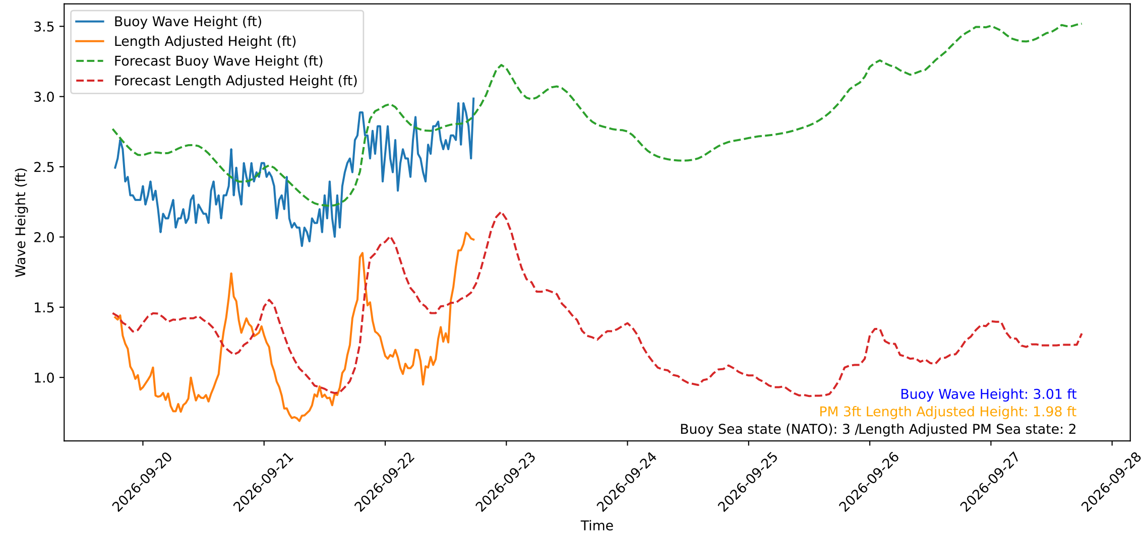
Wave Heights over Time for Red Beach at 2026-09-22 18:20:51
