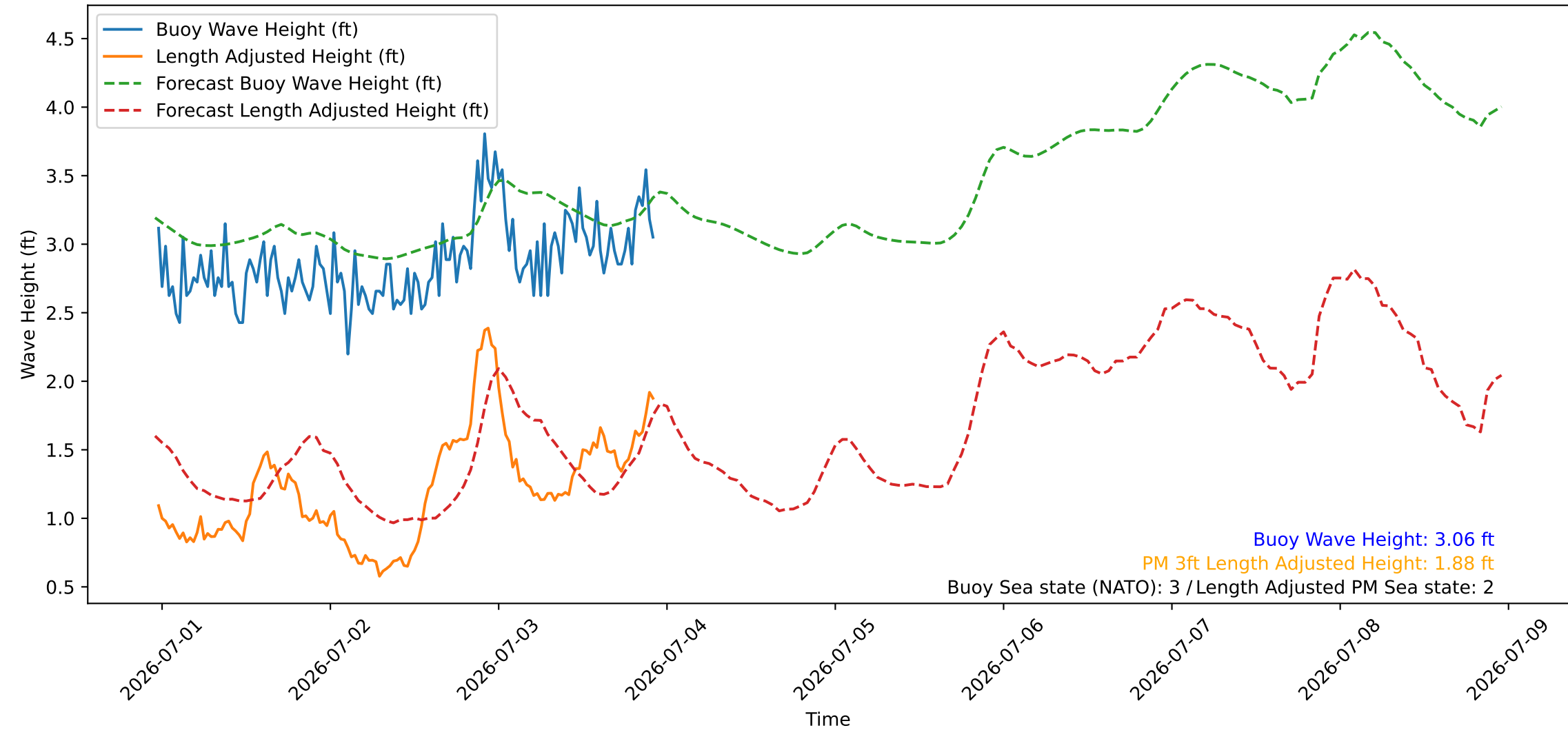
Wave Heights over Time for Red Beach at 2026-07-03 23:00:46
