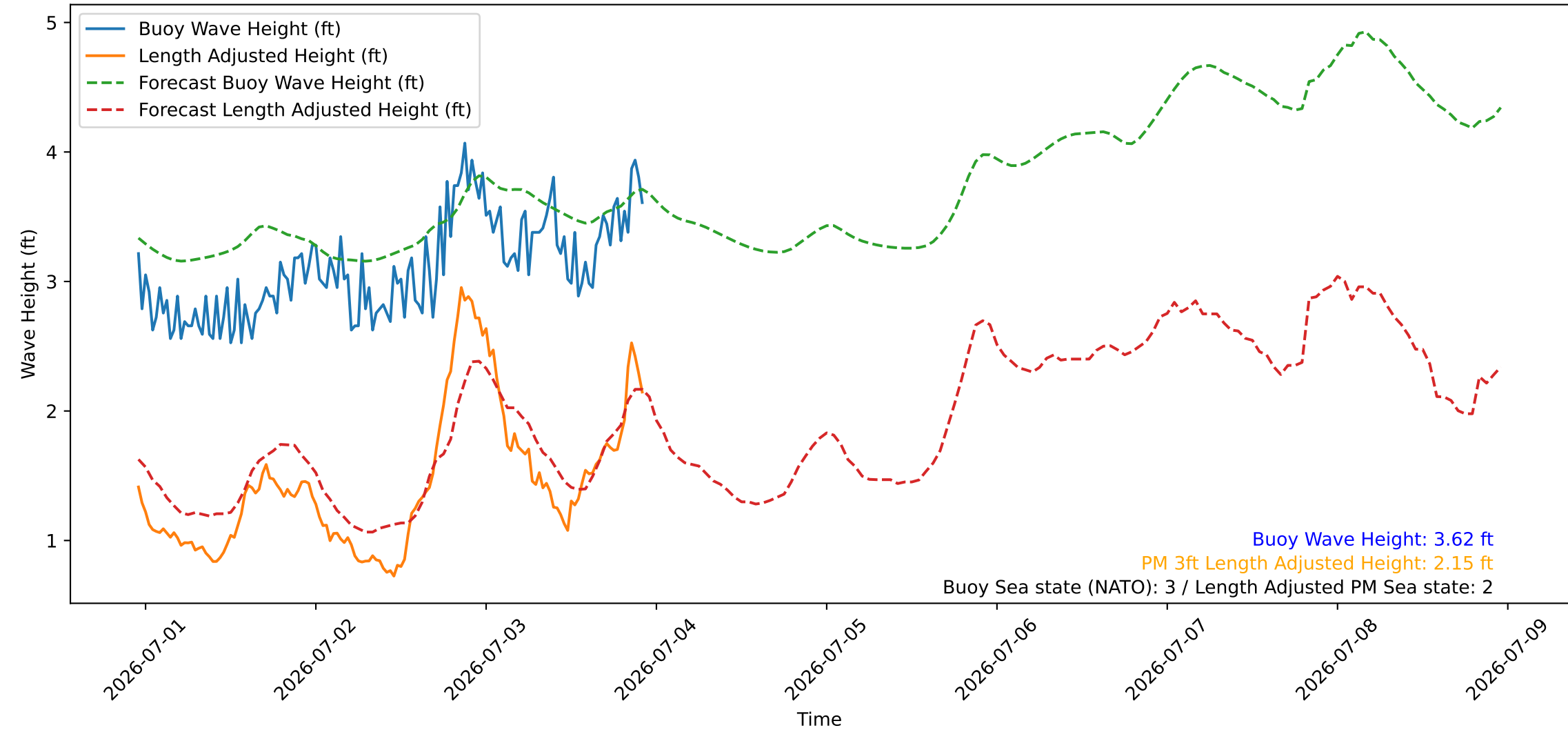
Wave Heights over Time for Green Beach at 2026-07-03 23:01:08
