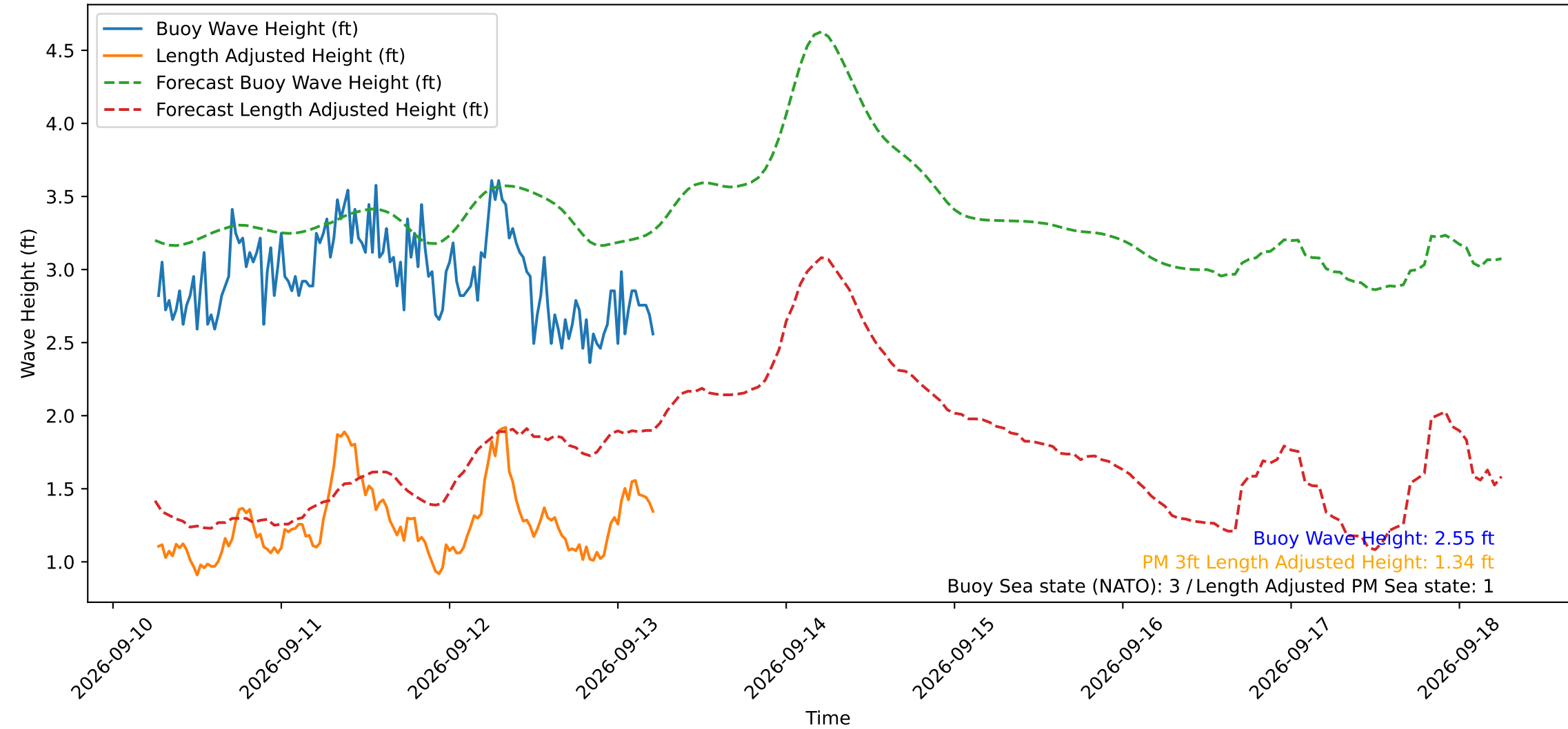
Wave Heights over Time for Green Beach at 2026-09-13 06:01:12
