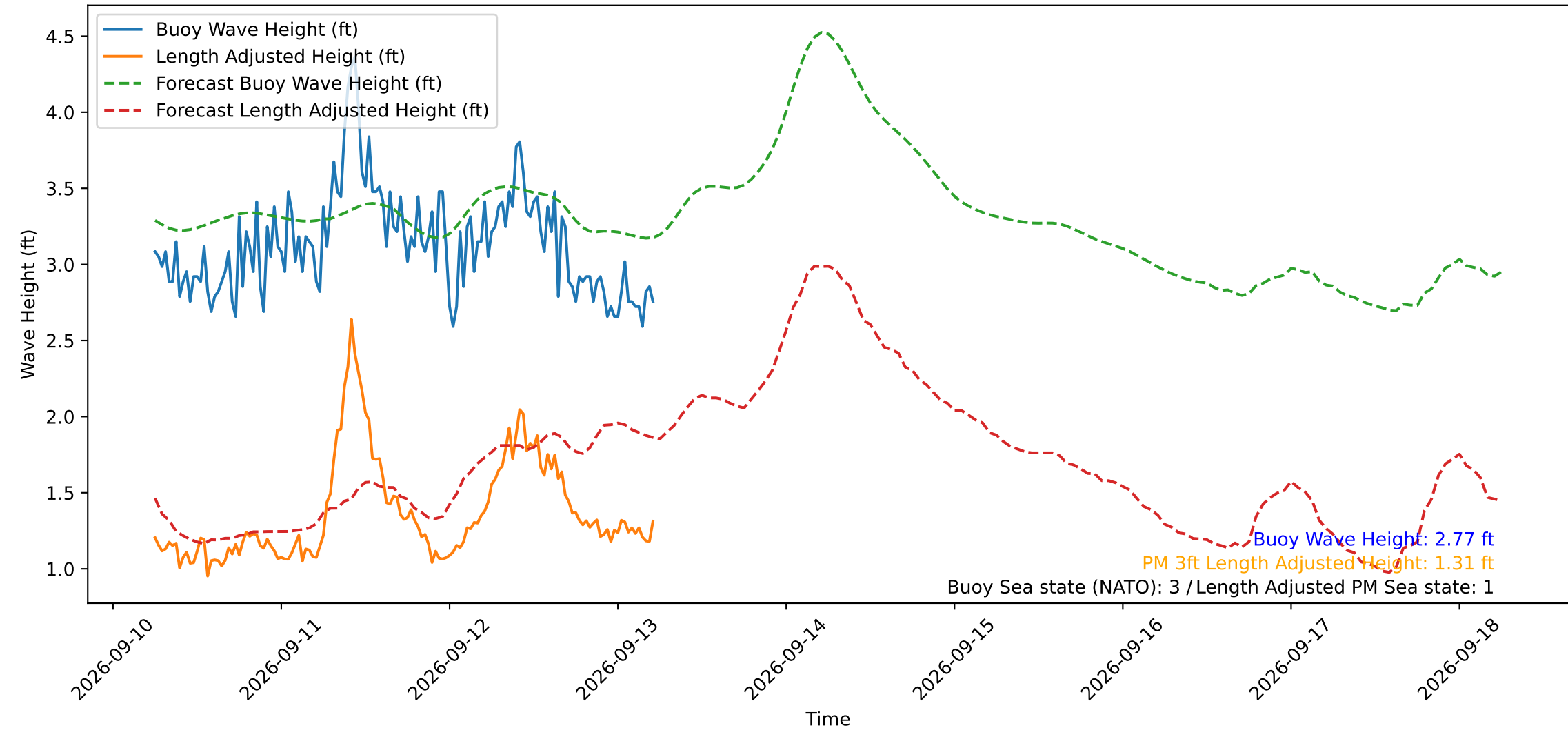
Wave Heights over Time for Oceanside Harbor at 2026-09-13 06:00:30
