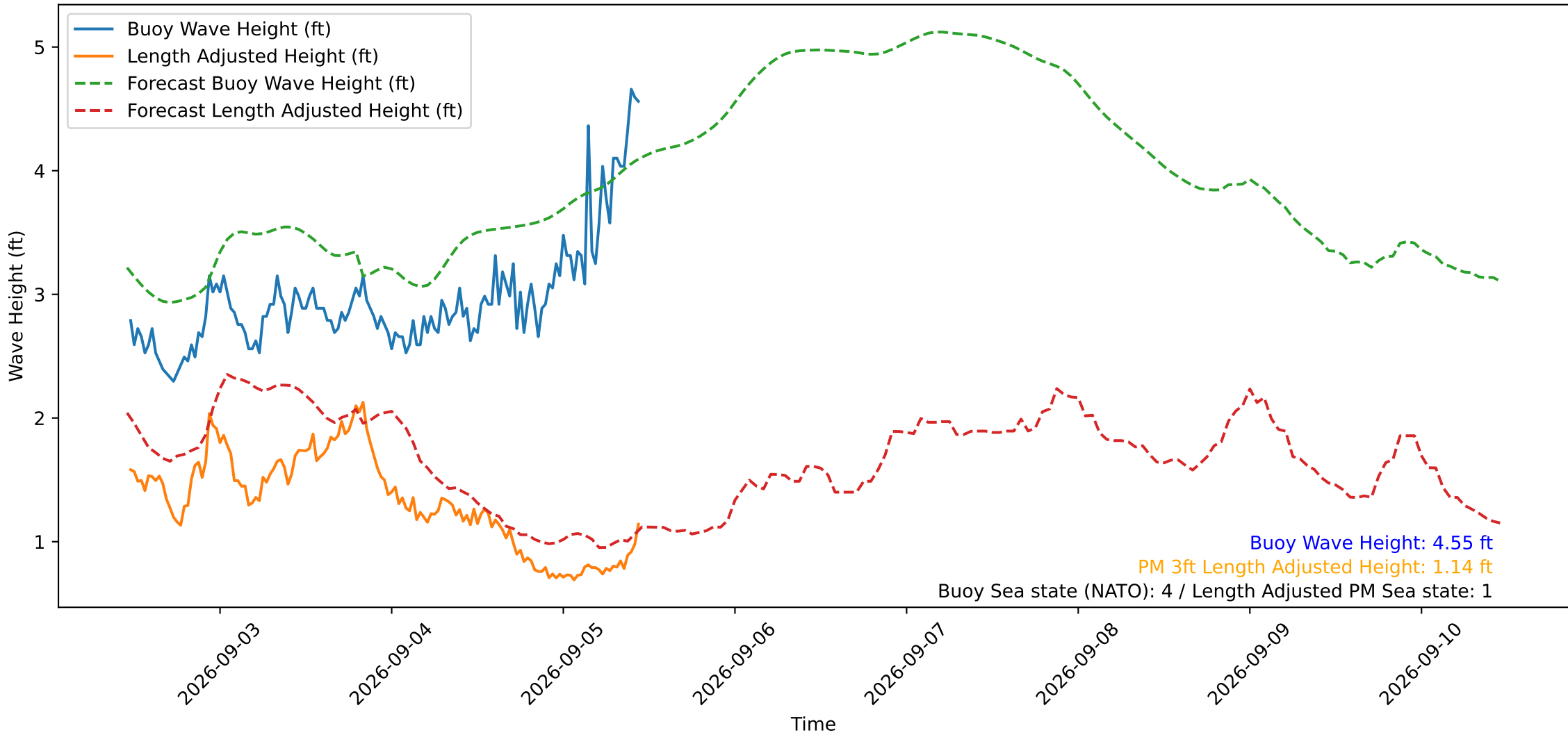
Wave Heights over Time for Red Beach at 2026-09-05 11:10:50
