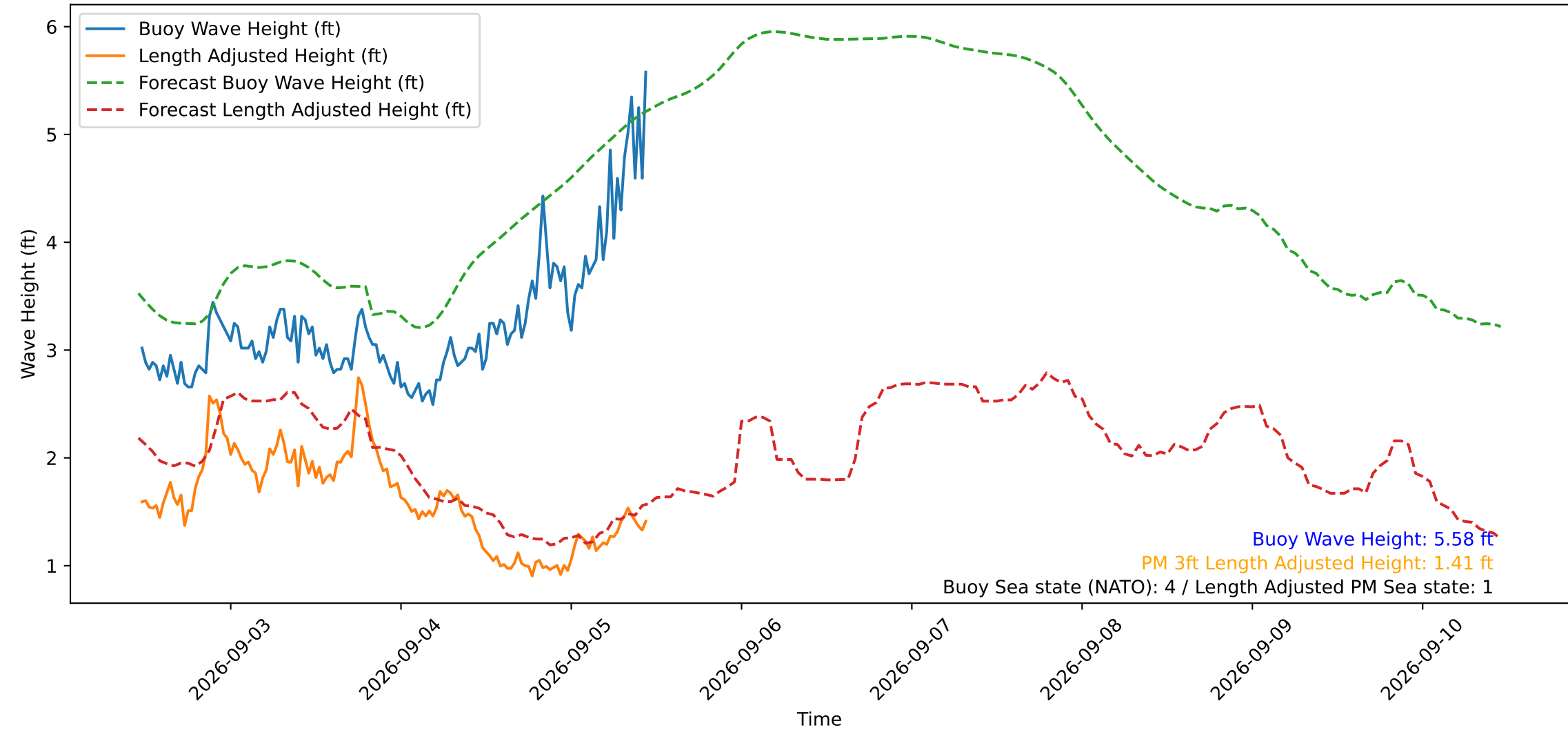
Wave Heights over Time for Green Beach at 2026-09-05 11:11:12
