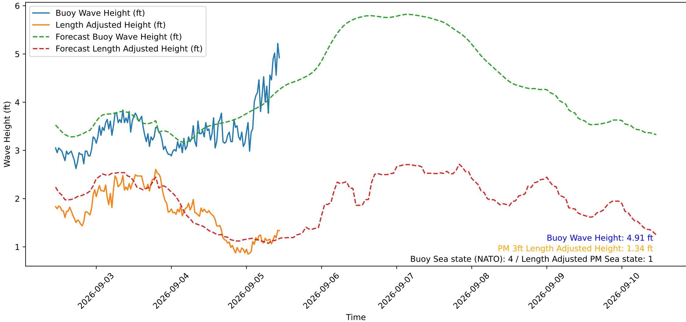
Wave Heights over Time for Oceanside Harbor at 2026-09-05 11:10:30
