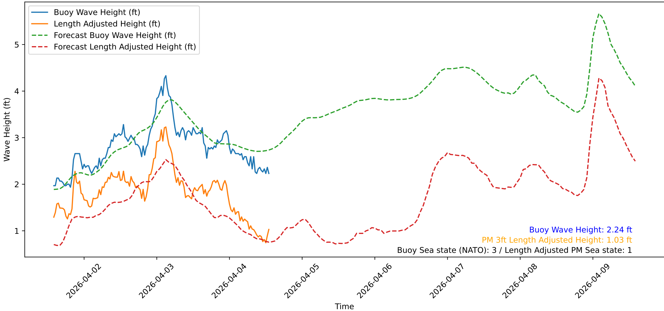
Wave Heights over Time for Green Beach at 2026-04-04 14:11:10
