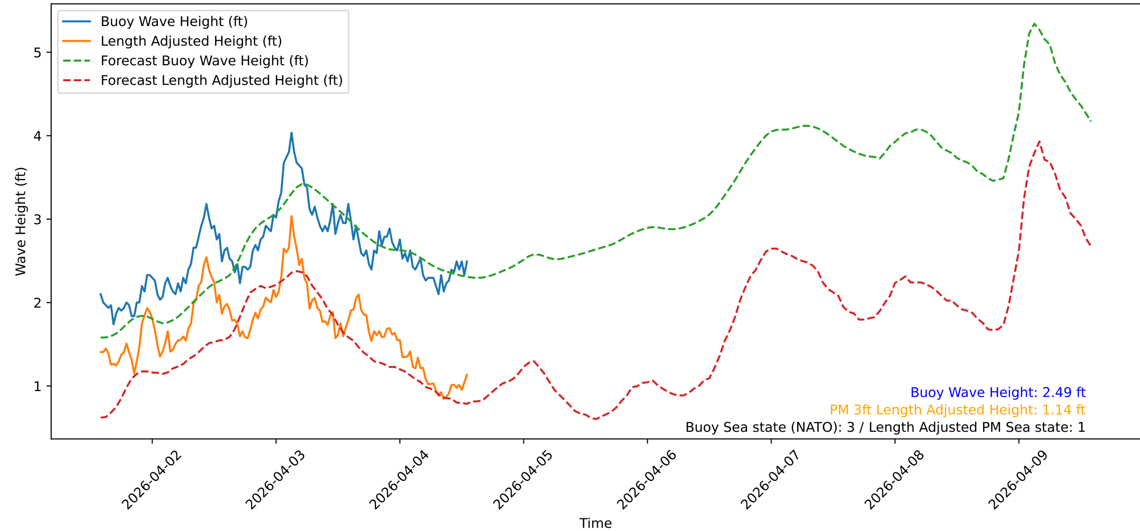
Wave Heights over Time for Oceanside Harbor at 2026-04-04 14:10:31
