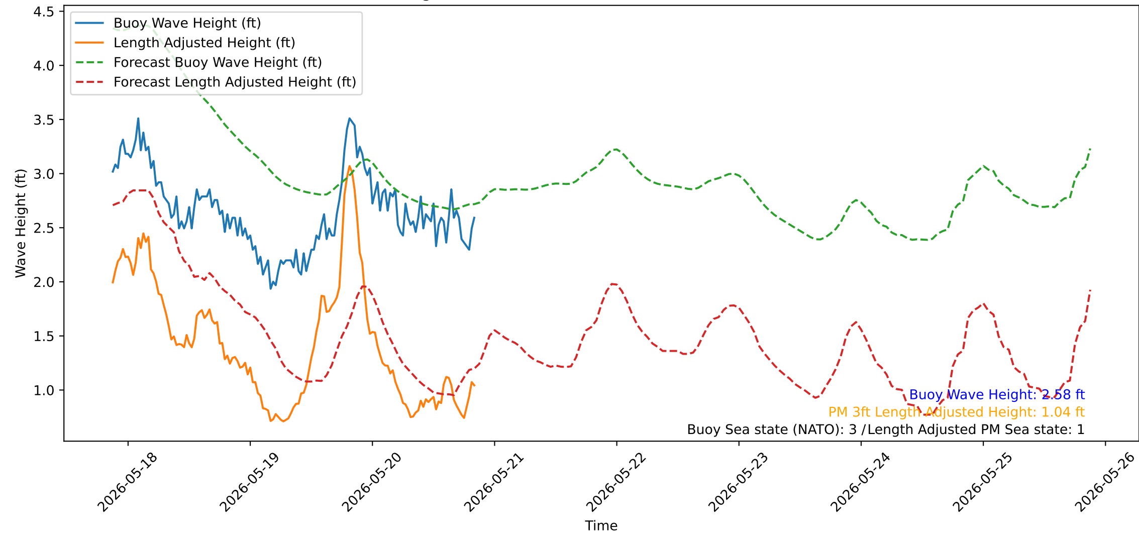
Wave Heights over Time for Red Beach at 2026-05-20 20:40:51
