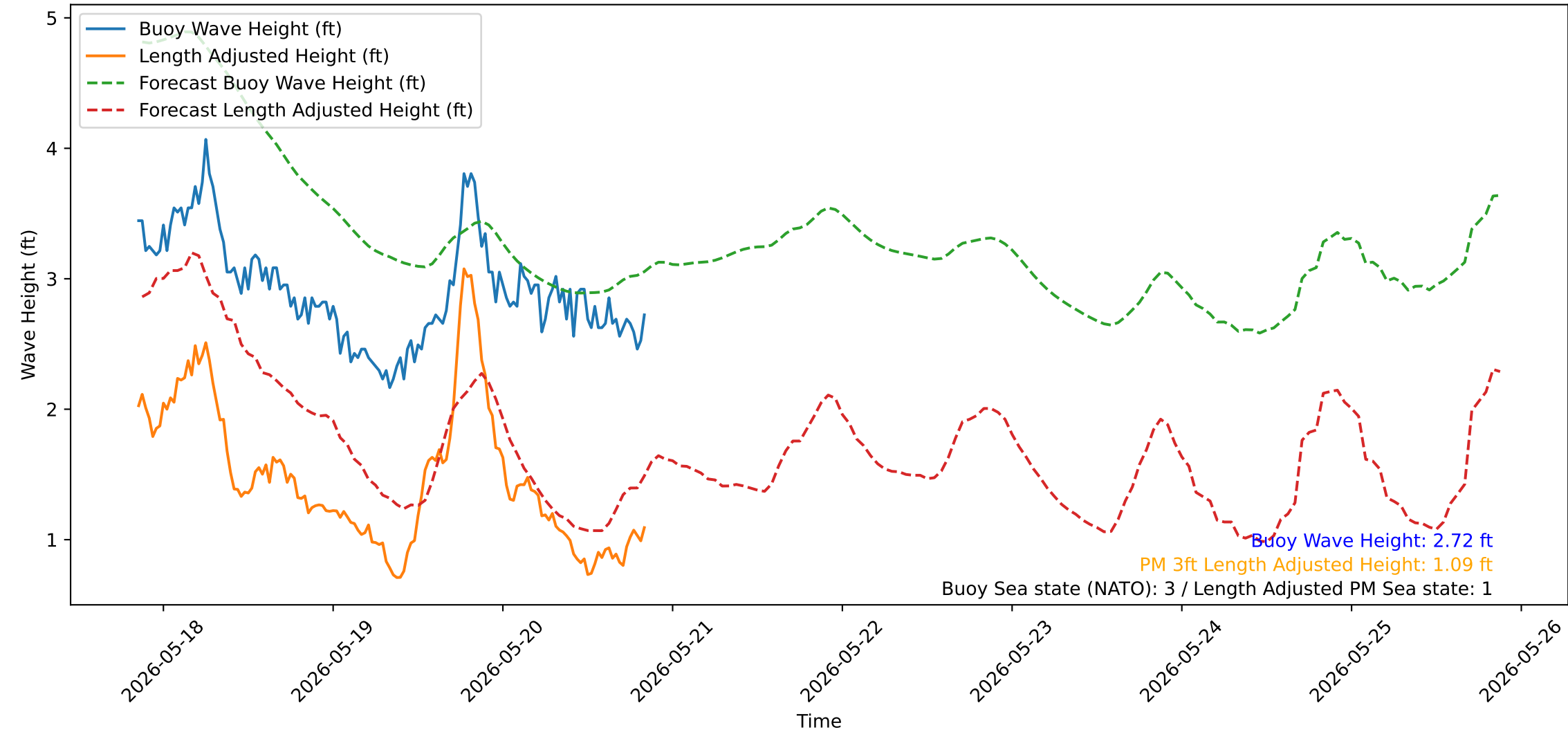
Wave Heights over Time for Green Beach at 2026-05-20 20:41:13
