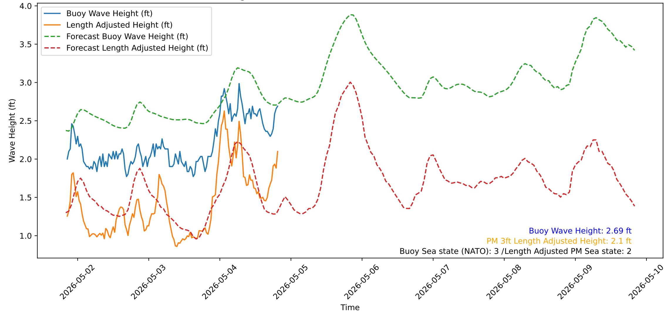
Wave Heights over Time for Green Beach at 2026-05-04 20:21:15
