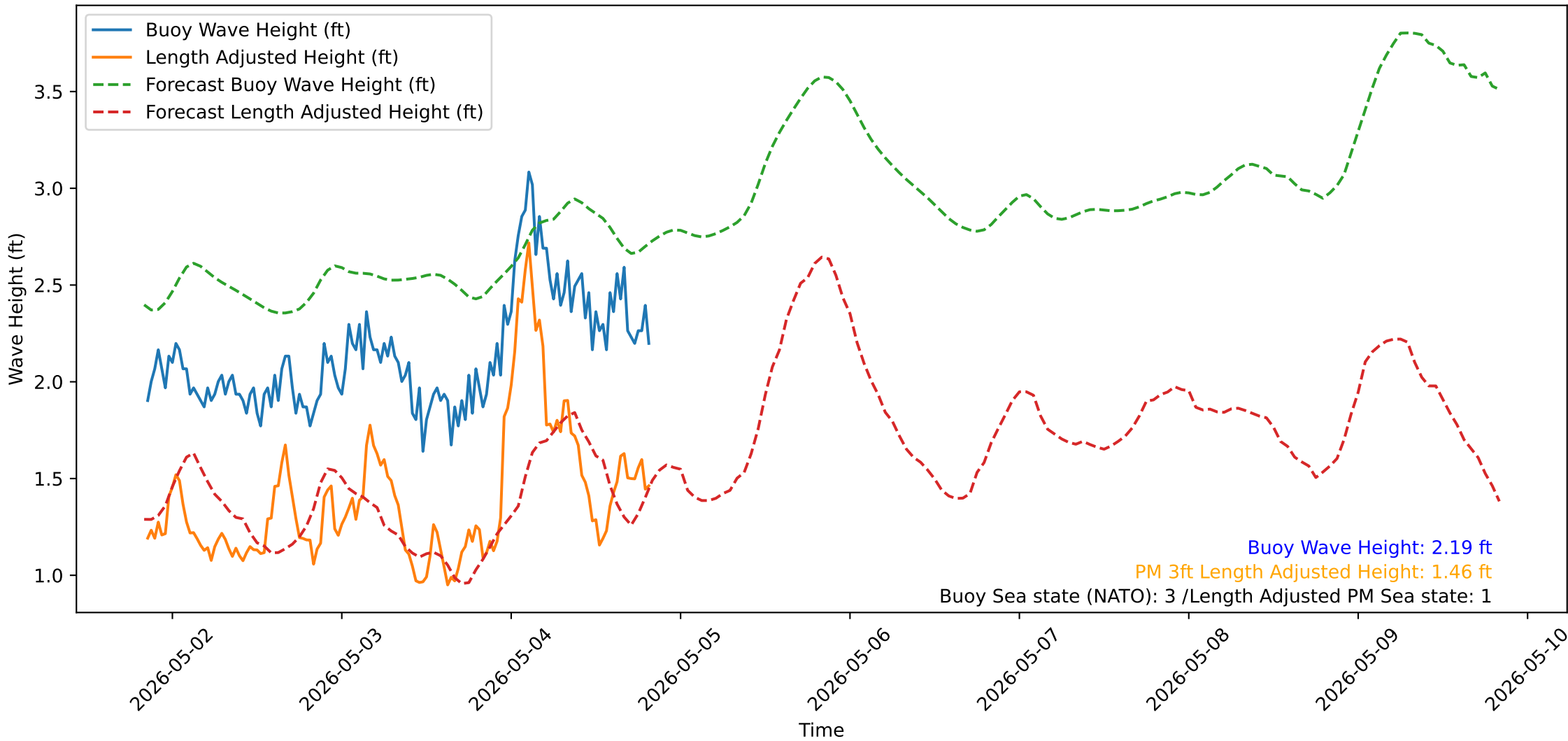
Wave Heights over Time for Oceanside Harbor at 2026-05-04 20:20:32
