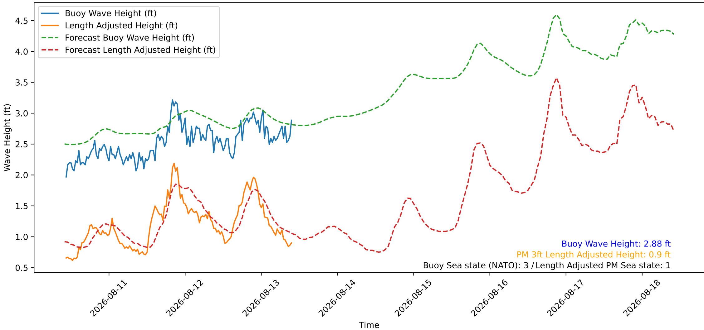
Wave Heights over Time for Green Beach at 2026-08-13 10:21:08
