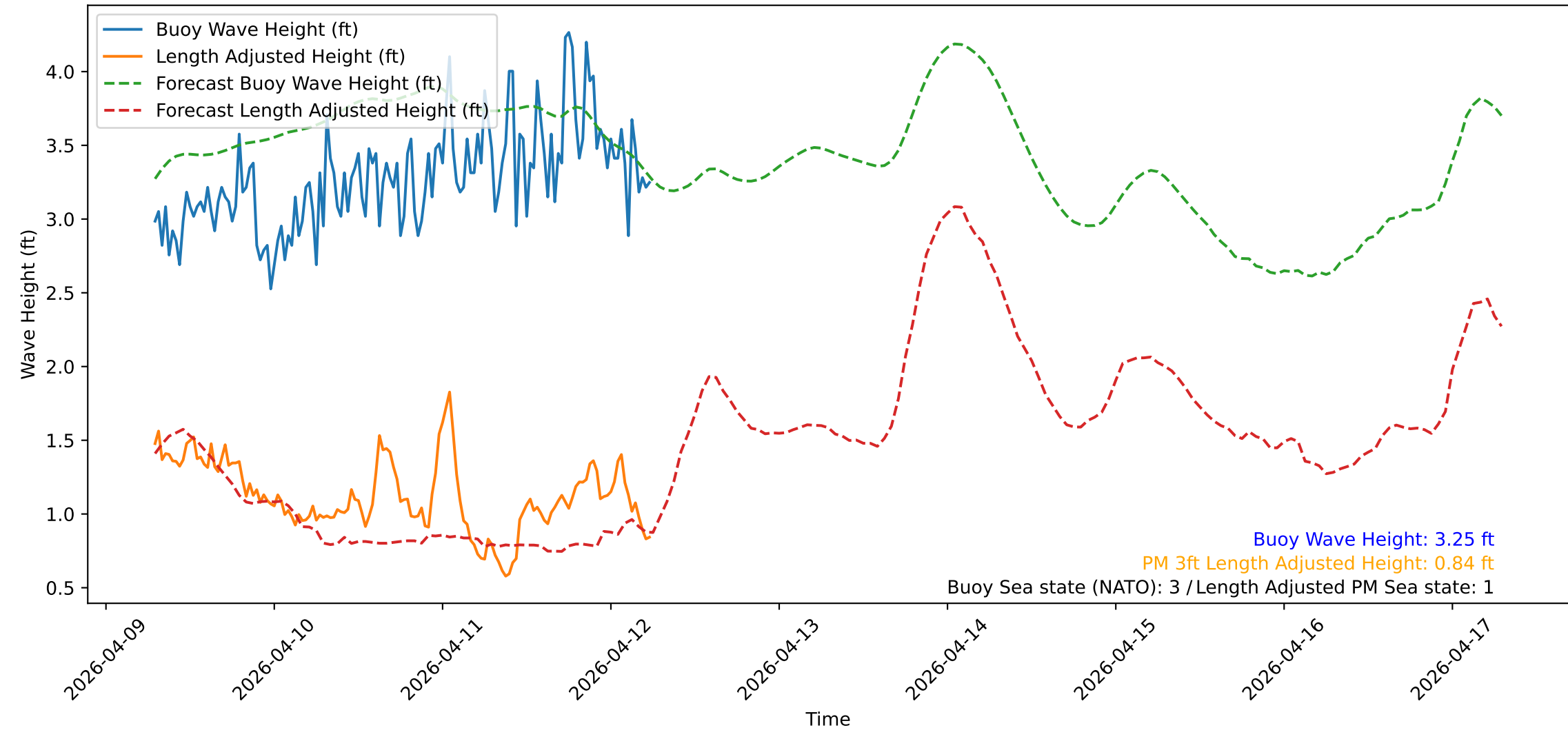
Wave Heights over Time for Red Beach at 2026-04-12 06:40:51
