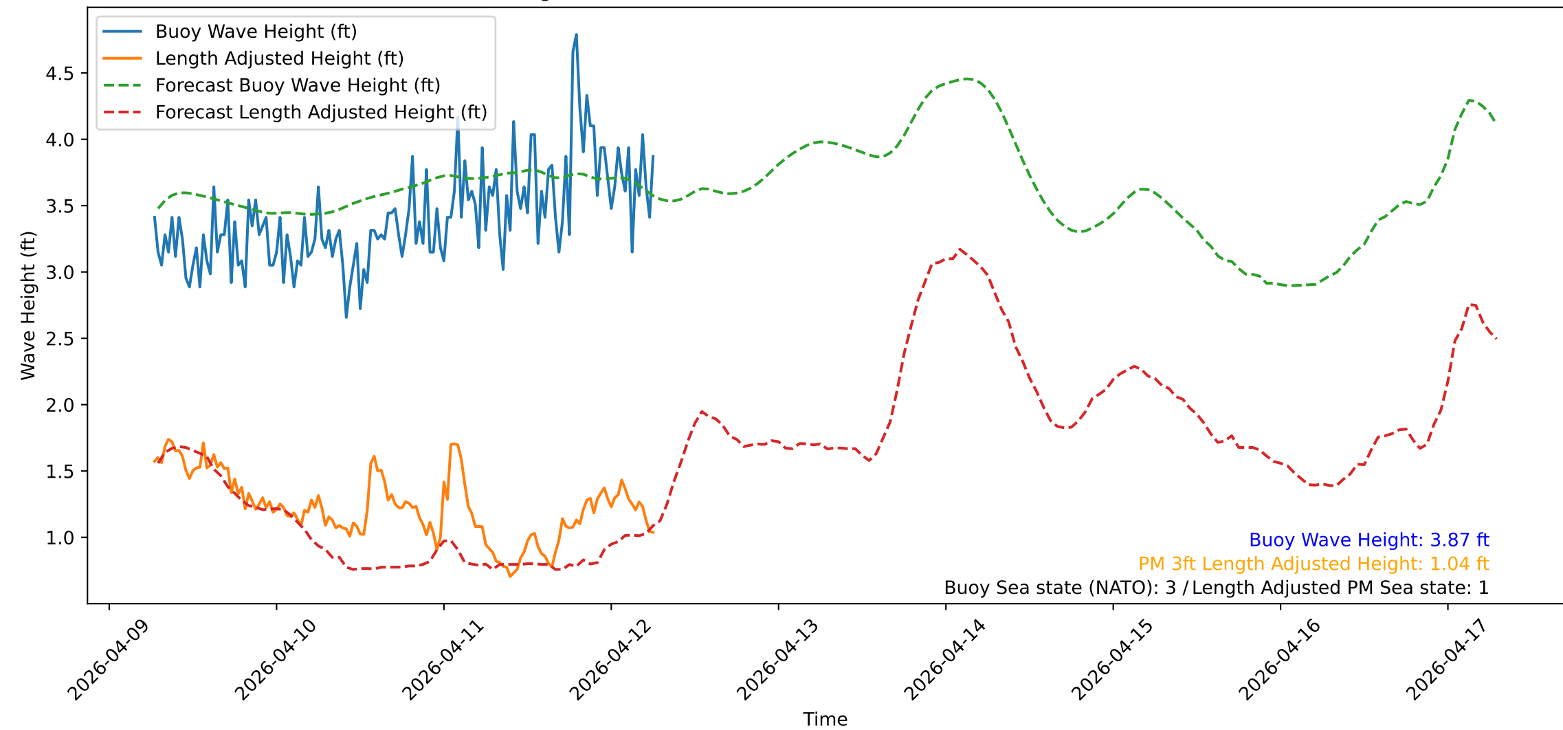
Wave Heights over Time for Oceanside Harbor at 2026-04-12 06:40:32
