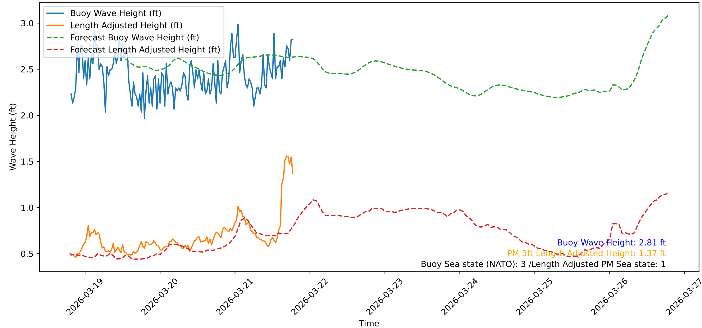
Wave Heights over Time for Oceanside Harbor at 2026-03-21 19:20:31
