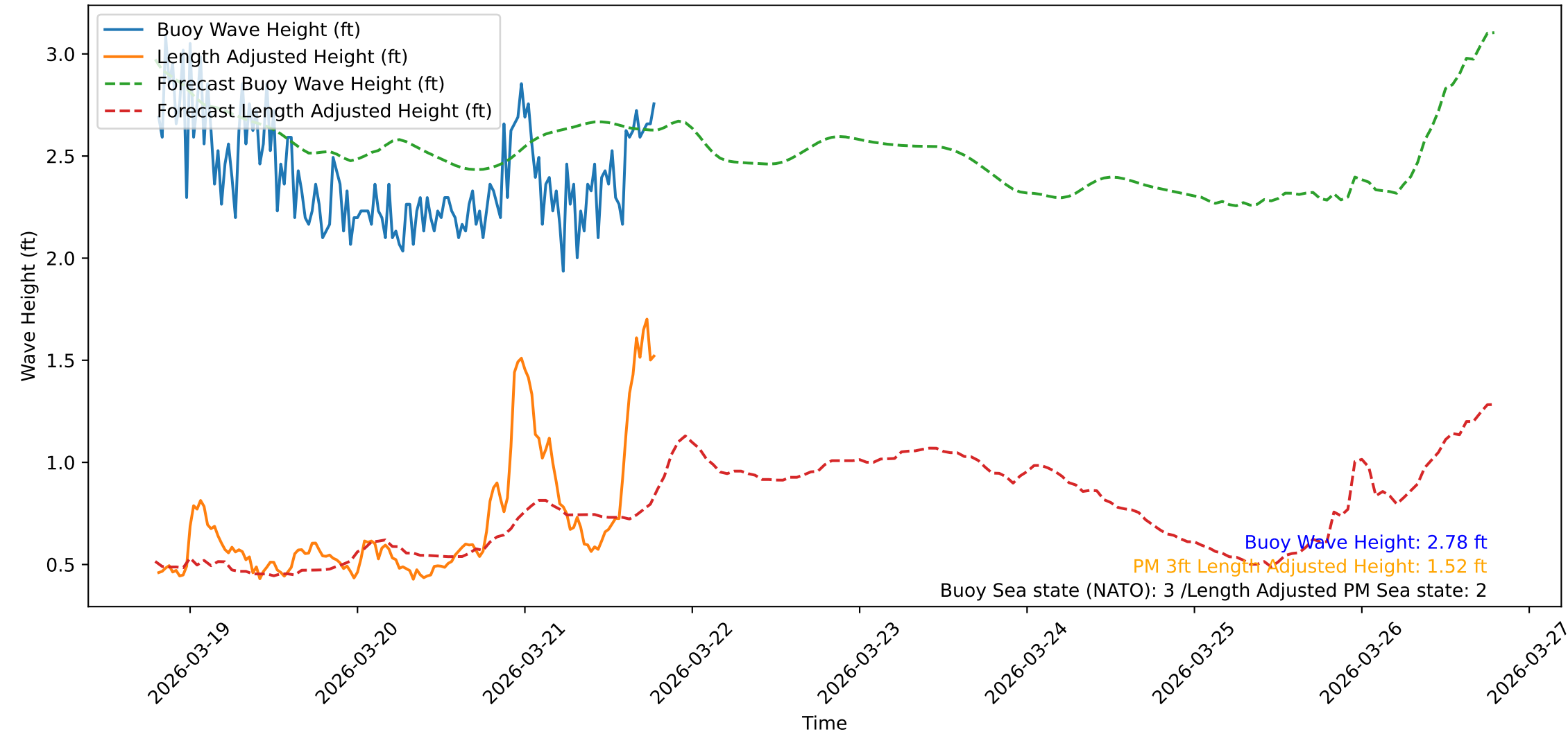
Wave Heights over Time for Green Beach at 2026-03-21 19:21:10
